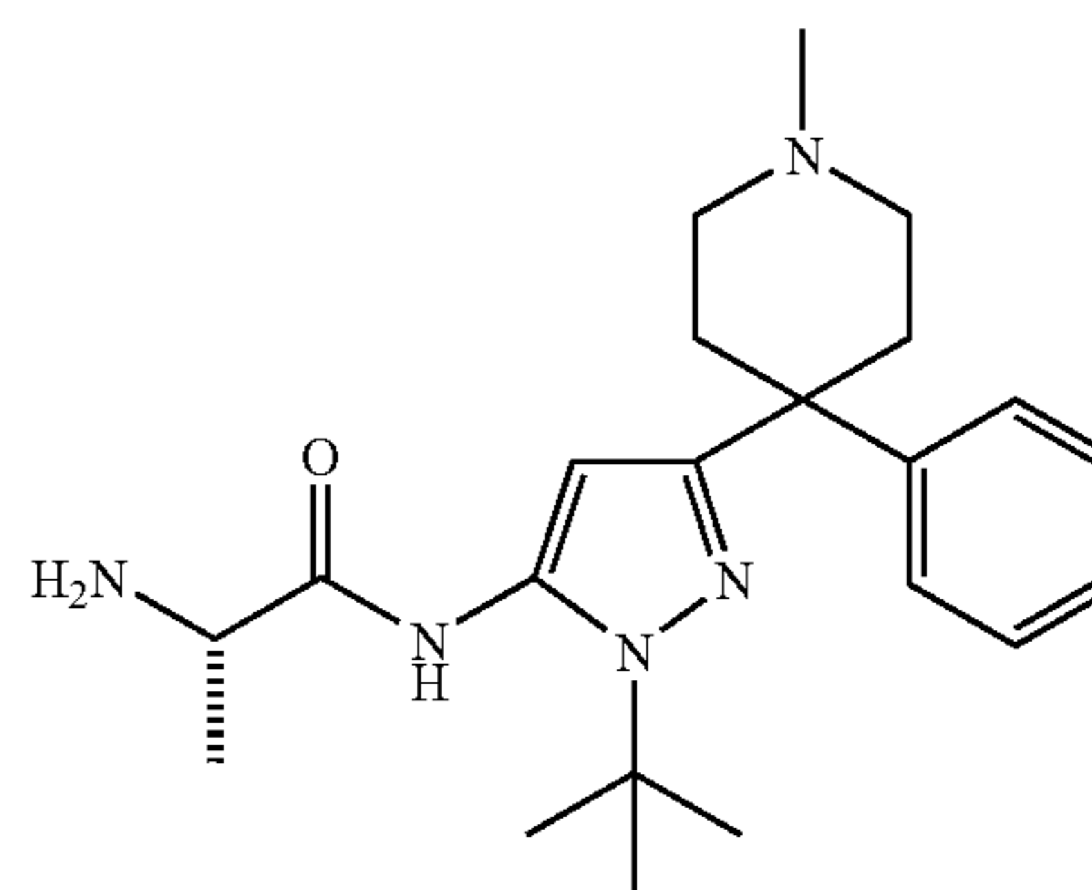
(2S)-2-Amino-N-[2-tert-butyl-5-(1-methyl-4-phenylpiperidin-4-yl)-2H-pyrazol-3-yl]-propionamide (7)
