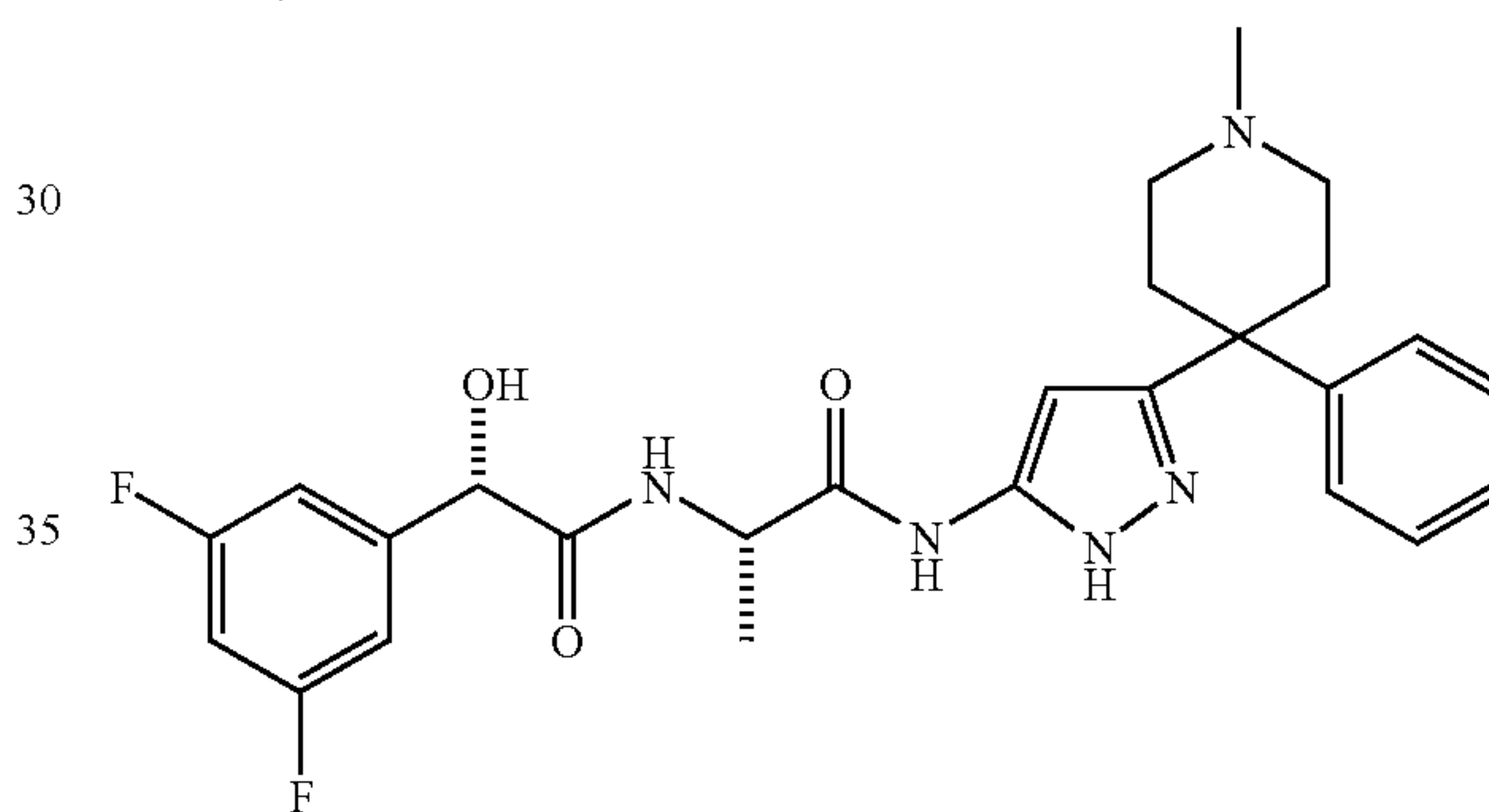
(2S,2'S)-2-[2'-(3,5-Difluorophenyl)-2'-hydroxyacetyl-amino]-N-[5-(1-methyl-4-phenylpiperidin-4-yl)-2H-pyrazol-3-yl]-propionamide
