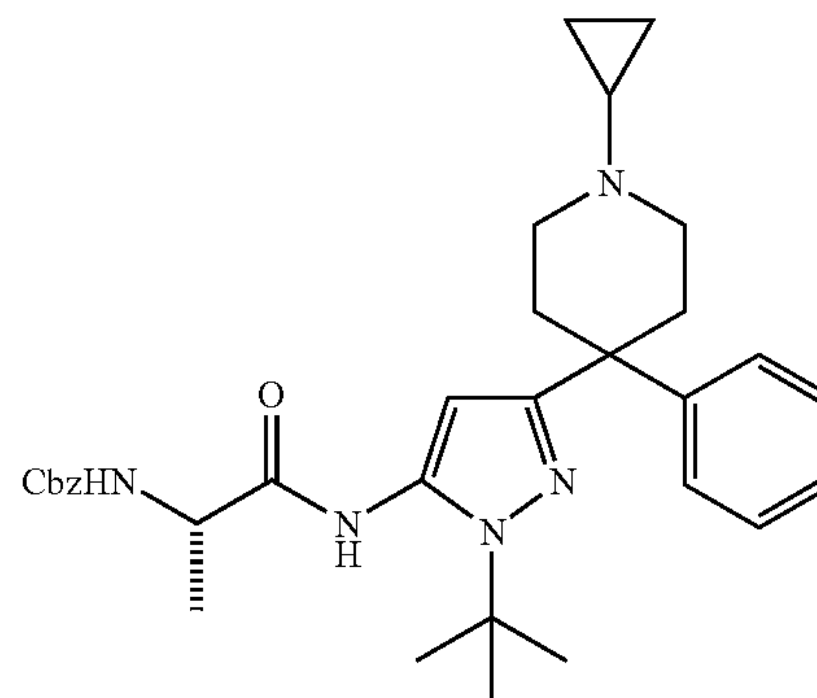
(S)-1-[2-tert-Butyl-5-(1-cyclopropyl-4-phenyl-piperidin-4-yl)-2H-pyrazol-3-ylcarbamoyl]-ethylcarbamate benzyl ester (11)
