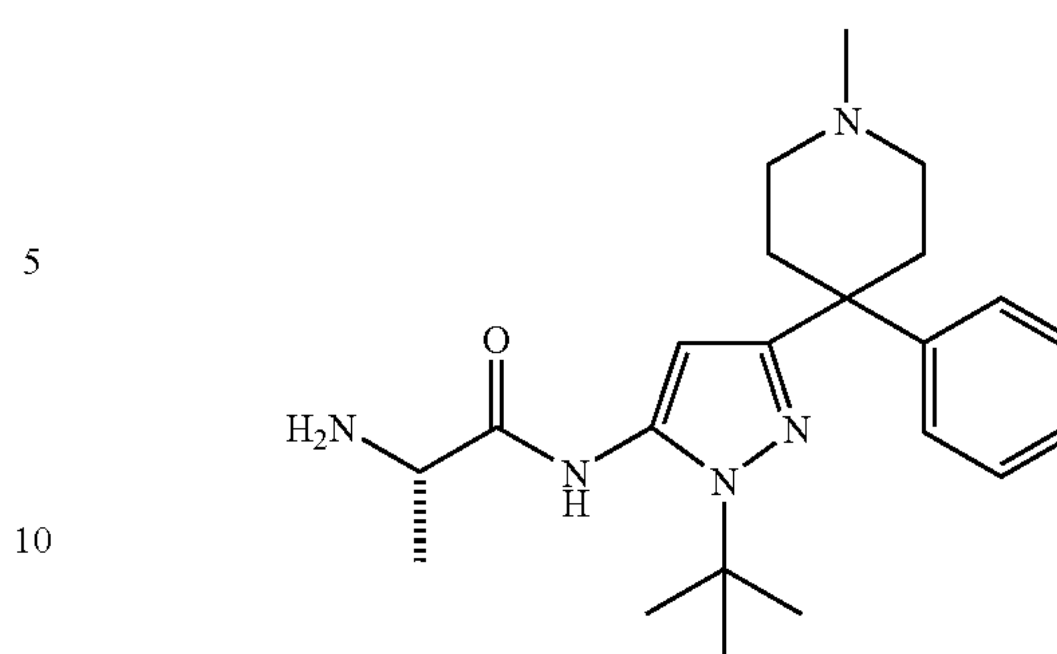
(2S)-2-Amino-N-[2-tert-butyl-5-(1-methyl-4-phenylpiperidin-4-yl)-2H-pyrazol-3-yl]-propionamide (7)
