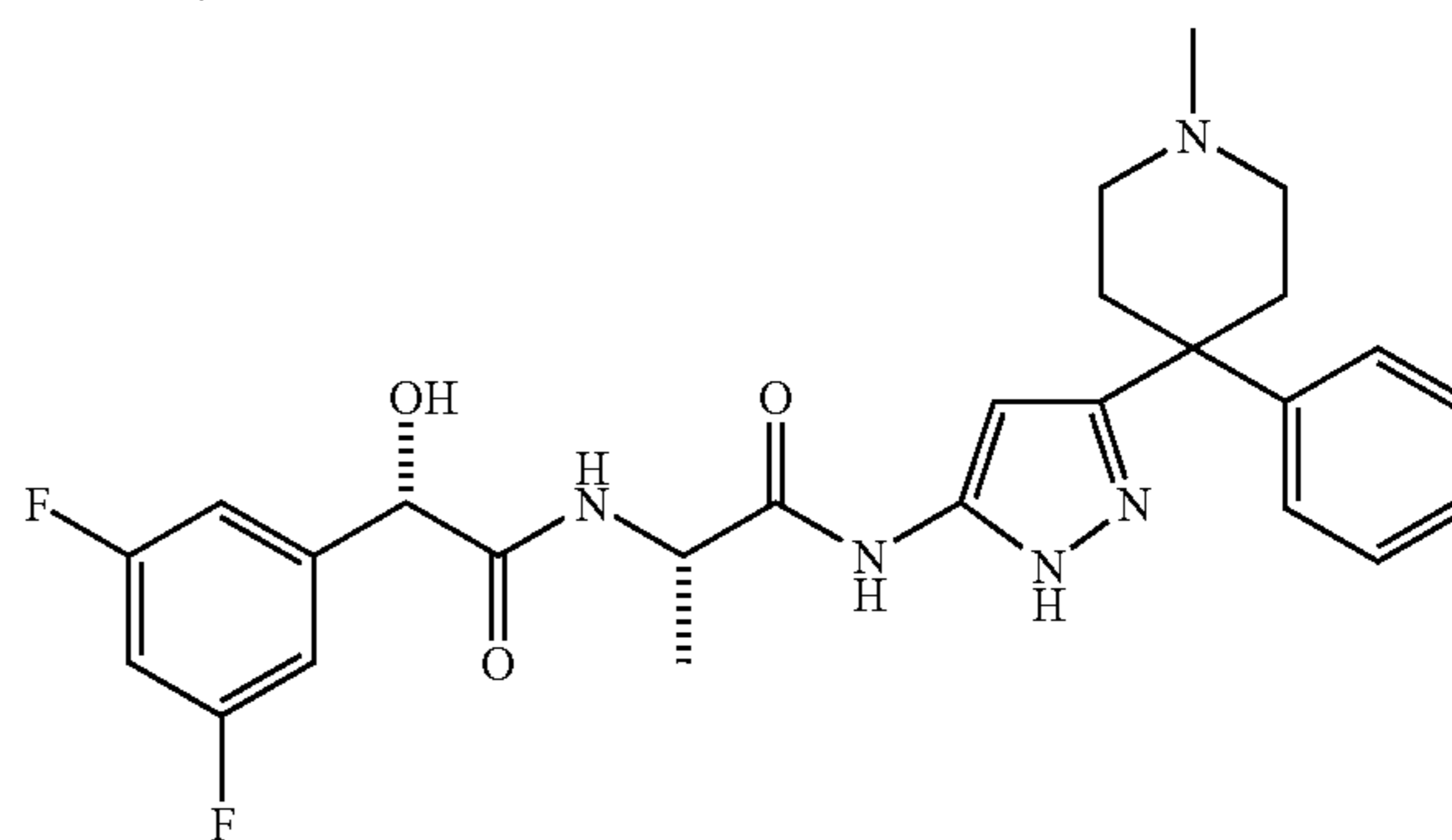
(2S,2'S)-2-[2'-(3,5-Difluorophenyl)-2'-hydroxyacetyl-amino]-N-[5-(1-methyl-4-phenylpiperidin-4-yl)-2H-pyrazol-3-yl]-propionamide
