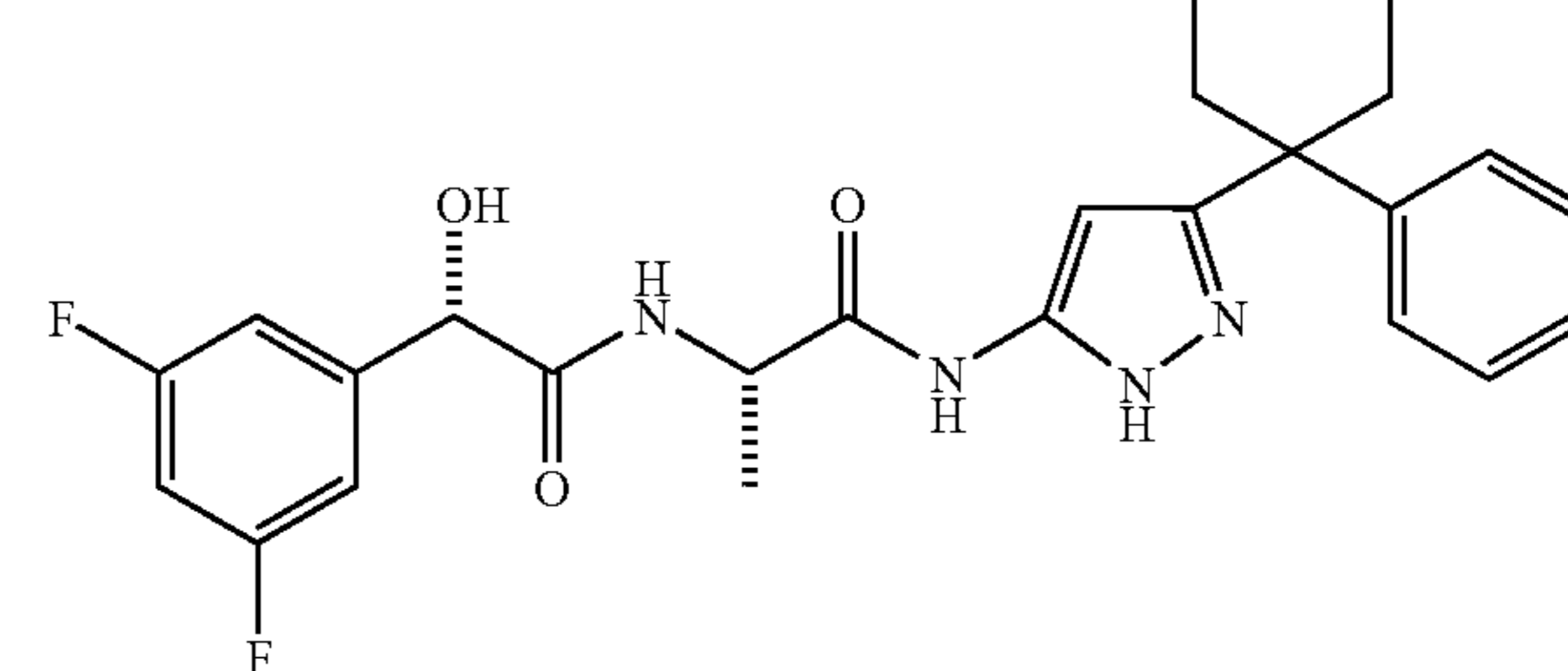
45 (2S,2'S)-N-[5-(1-Cyclopropyl-4-phenylpiperidin-4-yl)-2H-pyrazol-3-yl]-2-[2'-(3,5-difluorophenyl)-2'-hydroxylacetyl-amino]-propionamide
