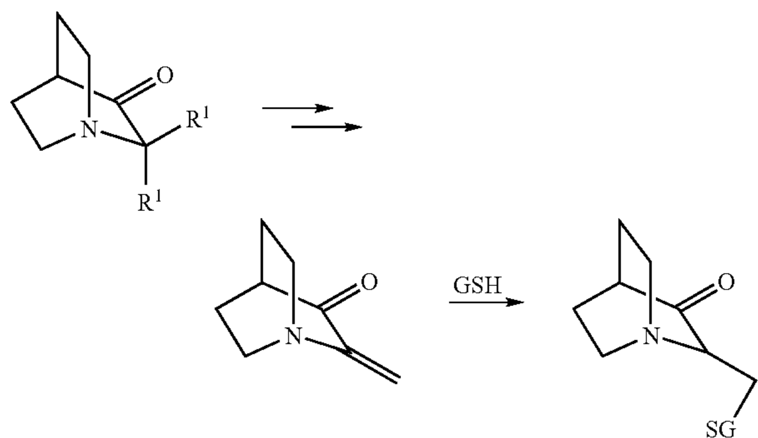
Reaction Scheme 1
