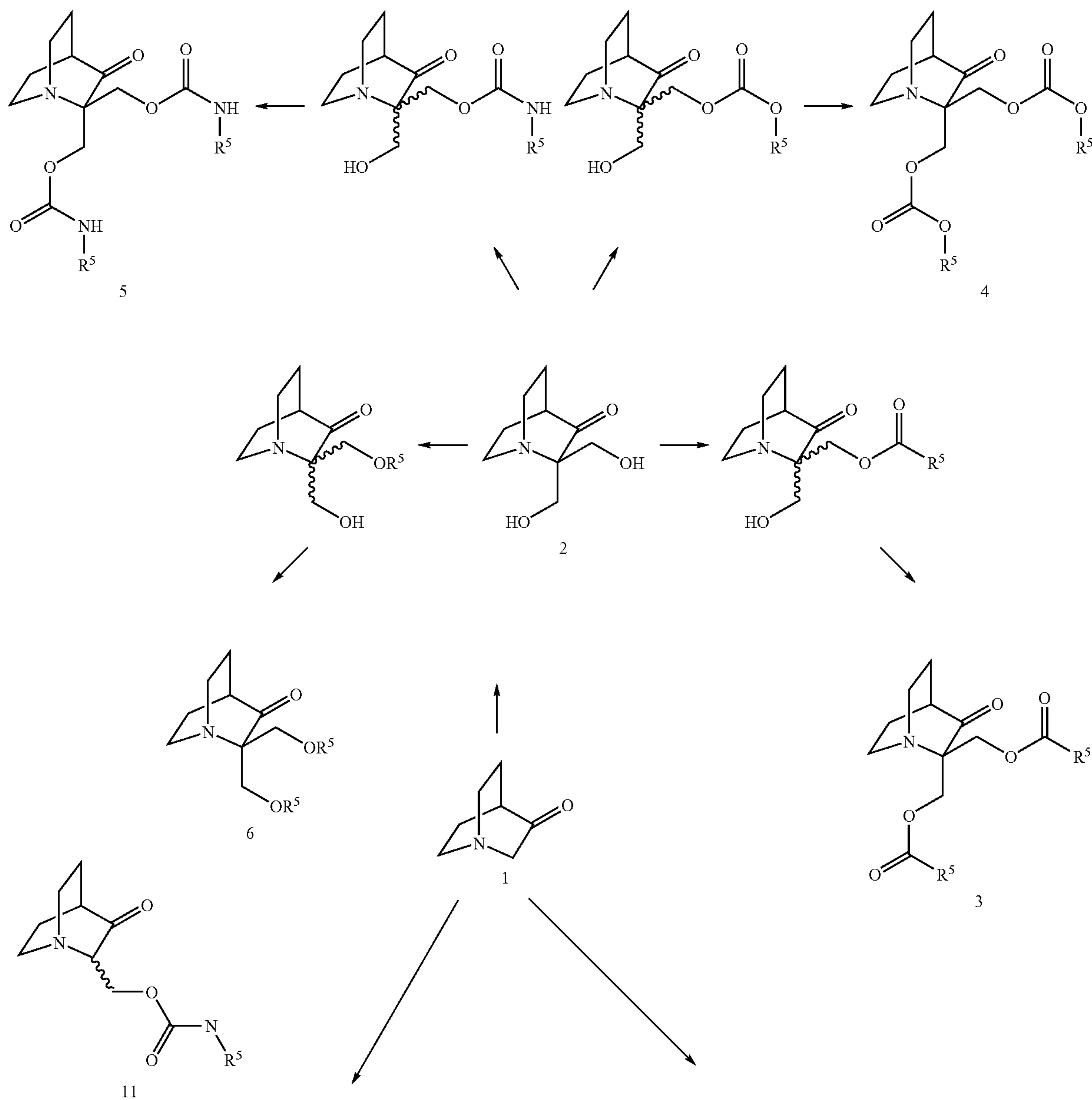
Reaction Scheme 2
