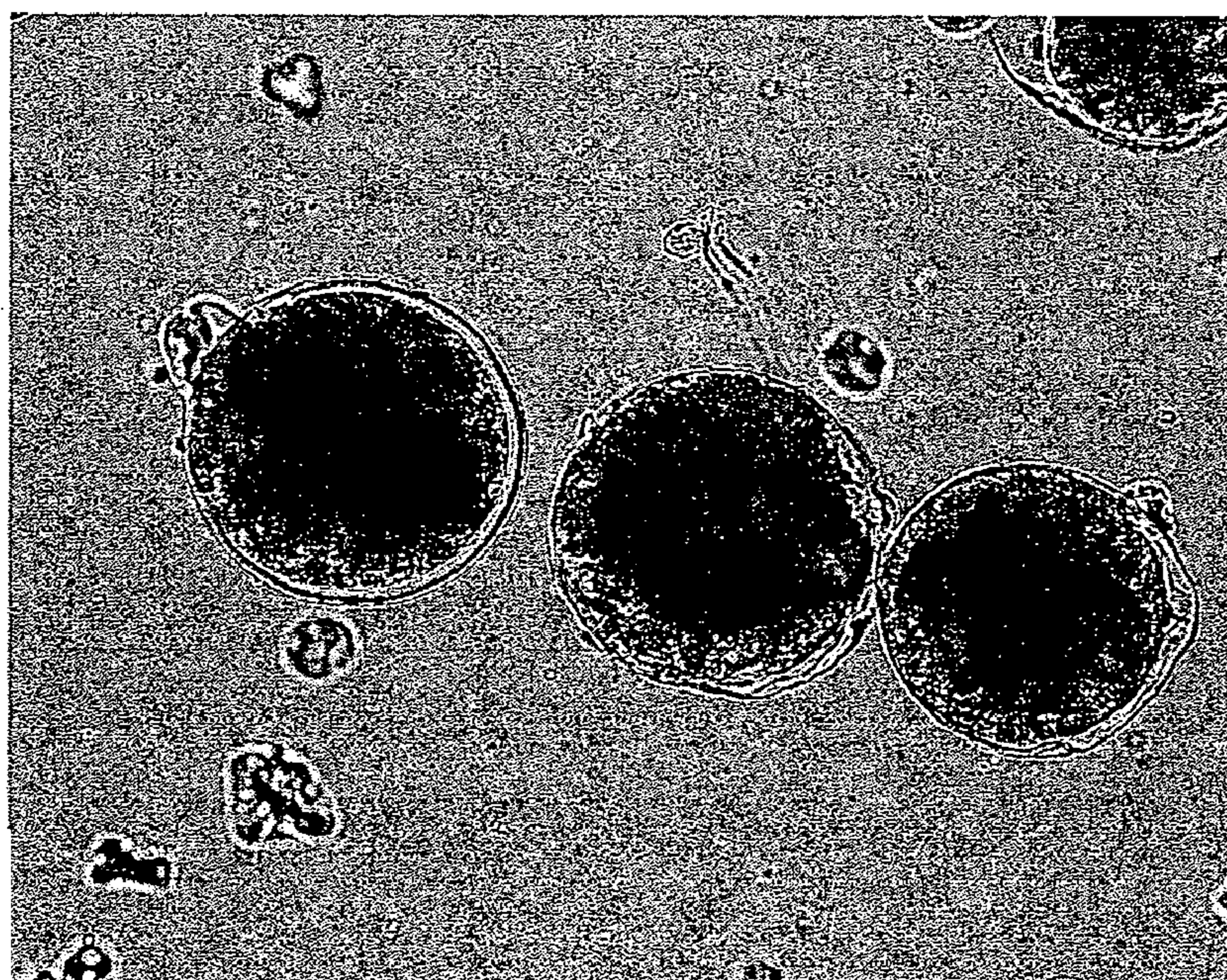
Microcapsules produced using conventional disk. (200X magnification)
