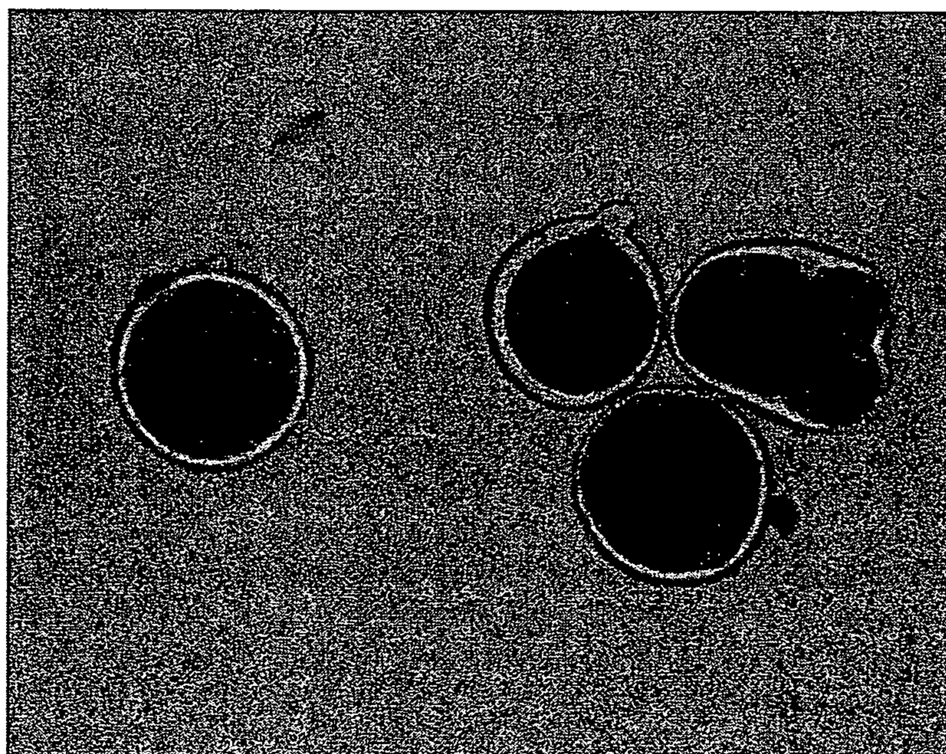
Microcapsules with improved coating uniformity. (200X magnification)
