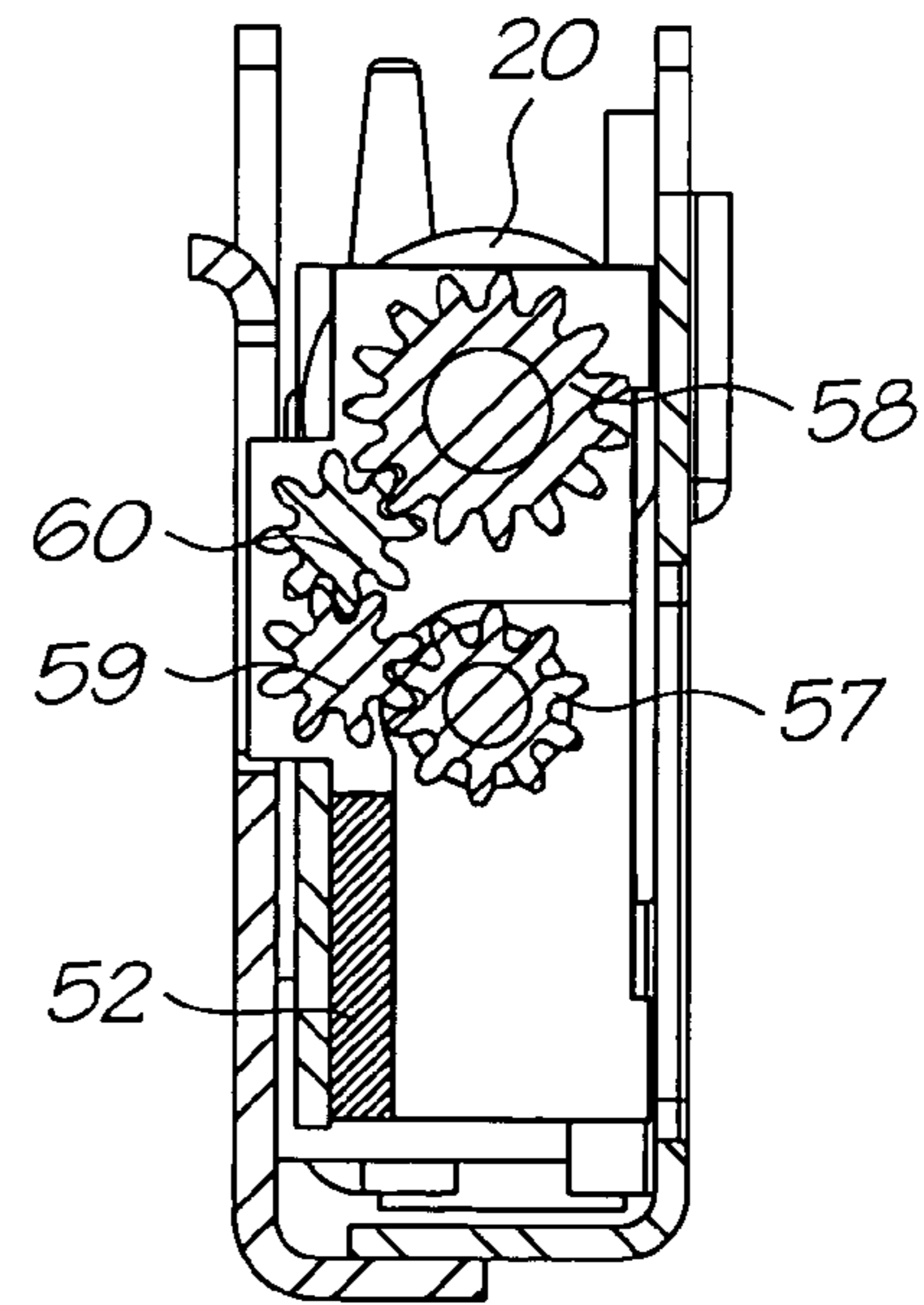
Section B-B
