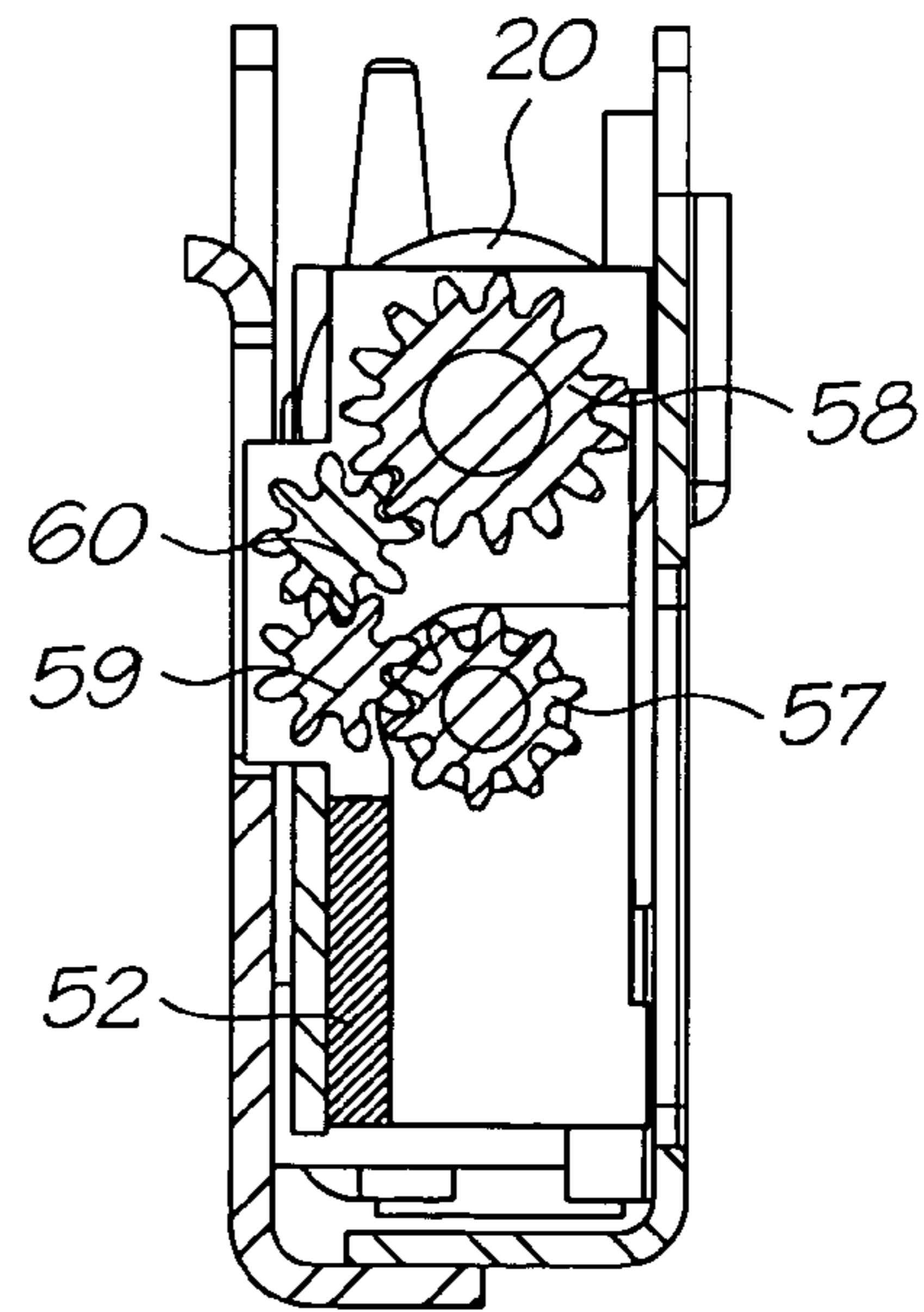
Section B-B
