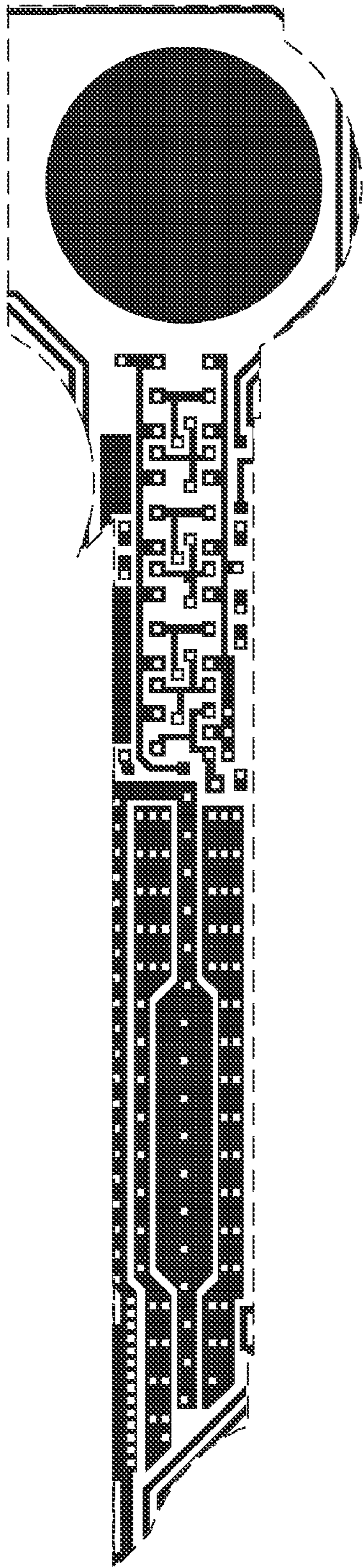
Metal 1 mask
