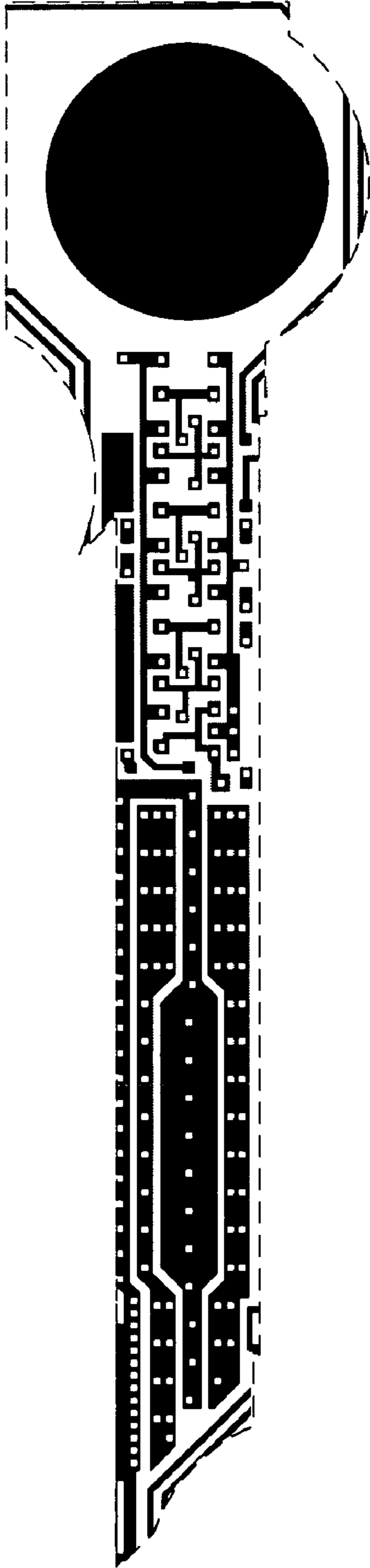
Metal 1 mask
