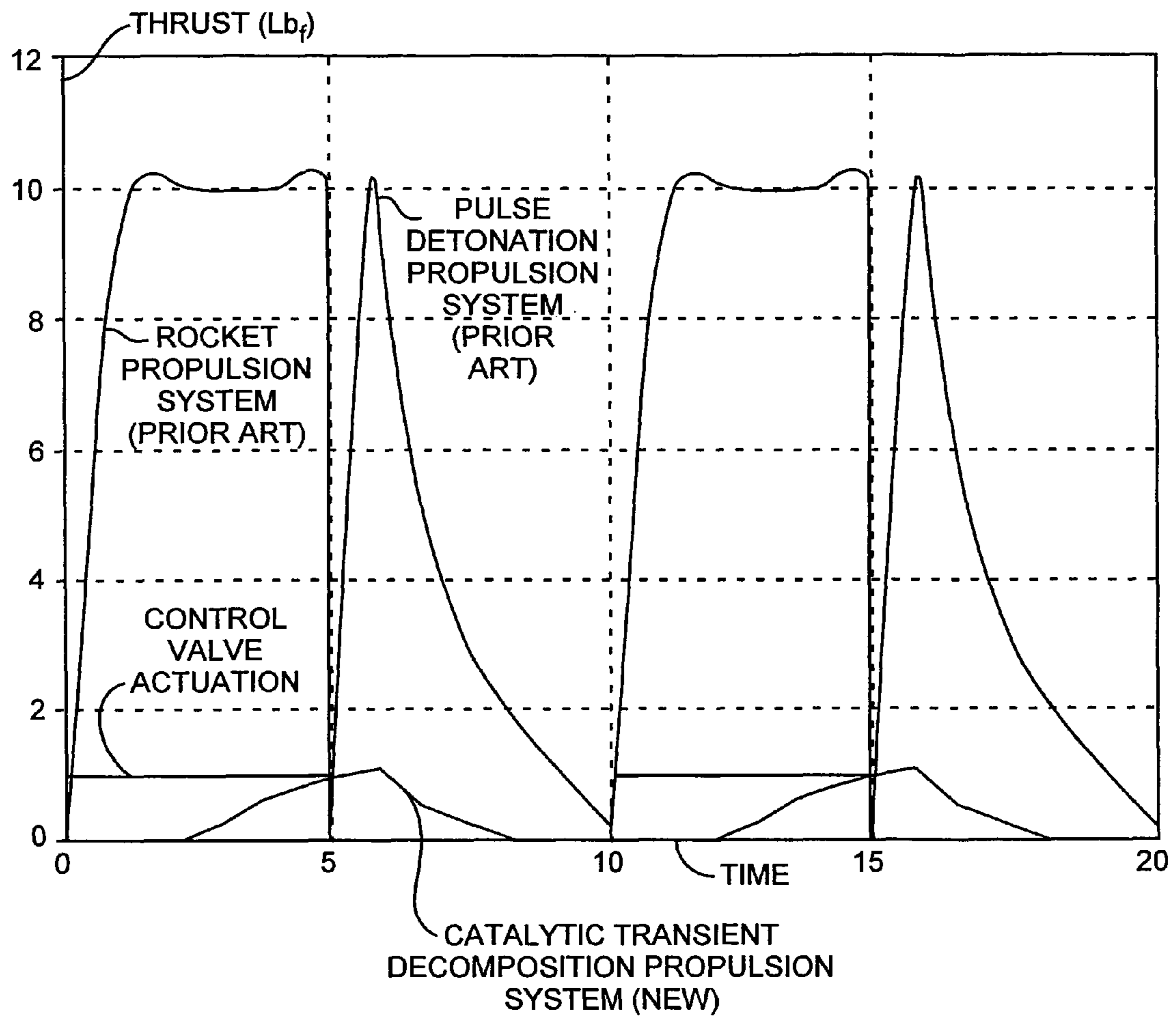
PROPULSION SYSTEM CONTROL DIAGRAM FIG. 2
