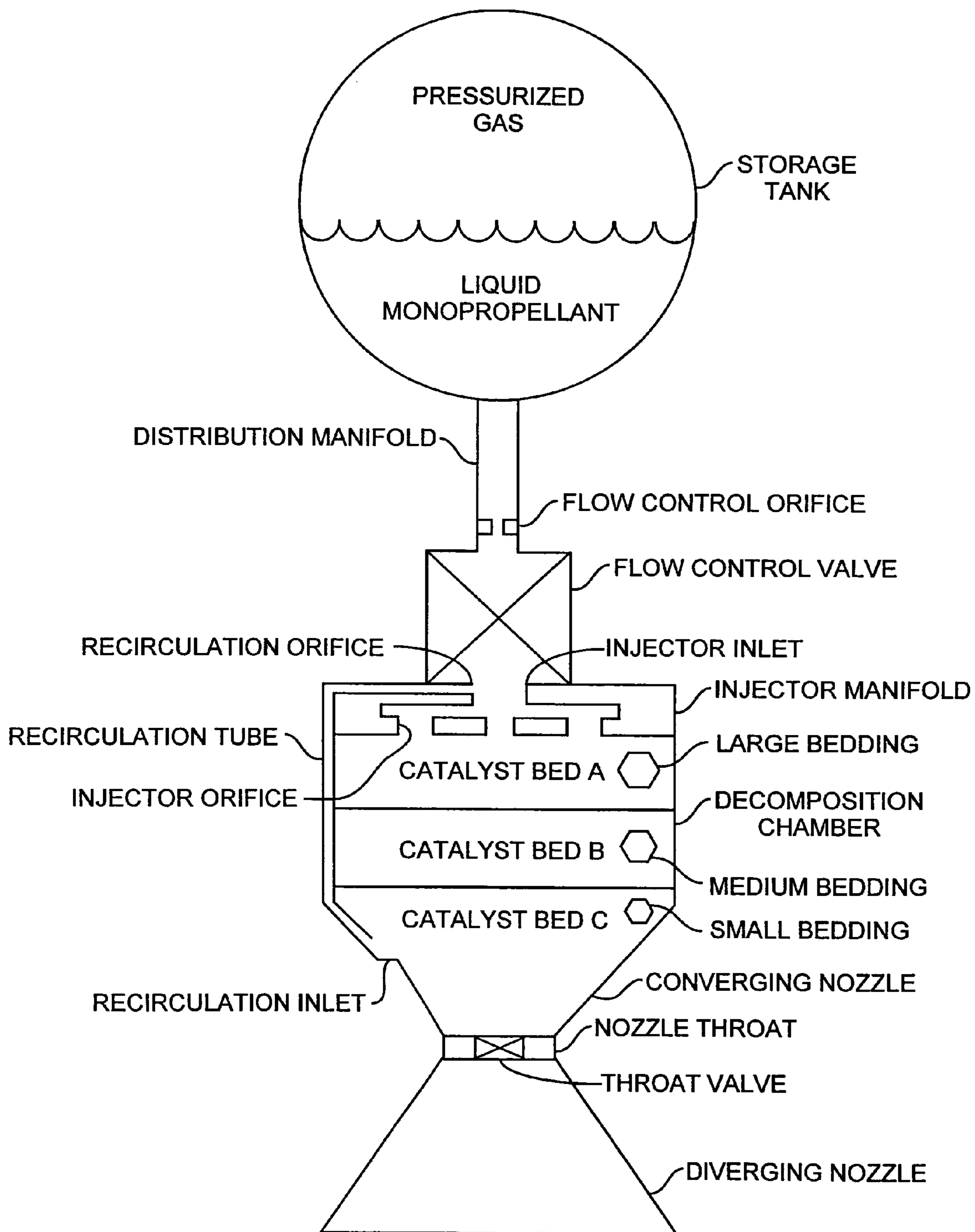
CATALYTIC TRANSIENT DECOMPOSITION PROPULSION SYSTEM
