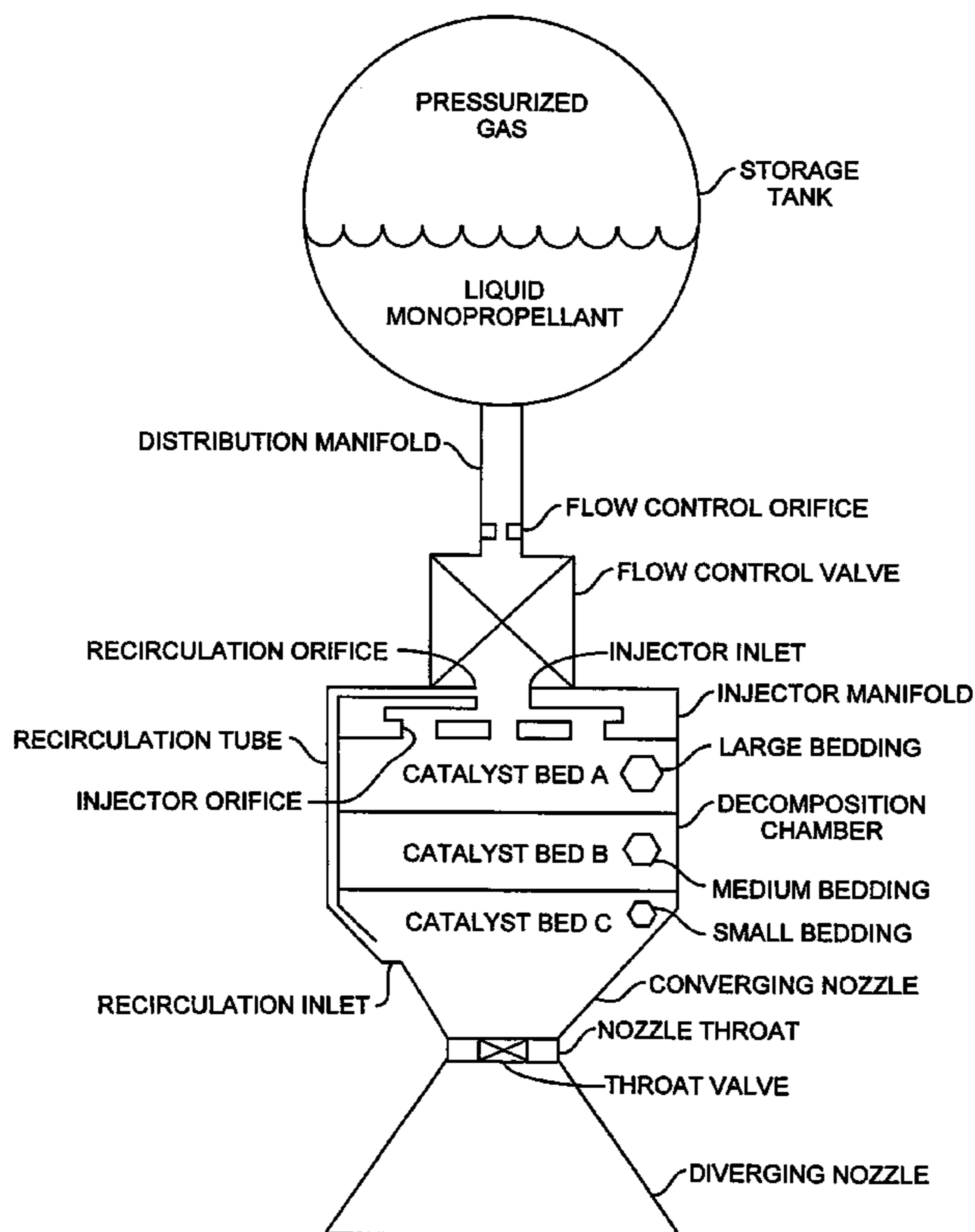
CATALYTIC TRANSIENT DECOMPOSITION PROPULSION SYSTEM
