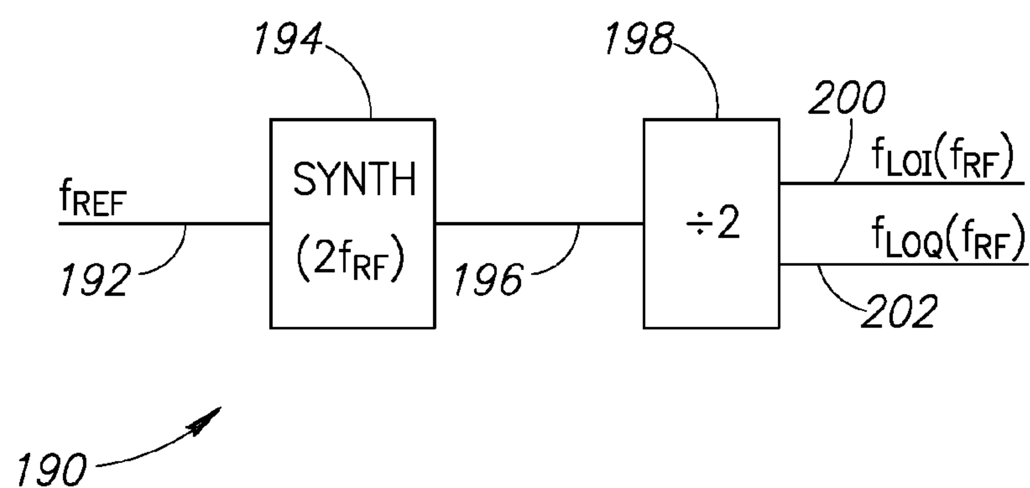
FIG. 3 (PRIOR ART)
