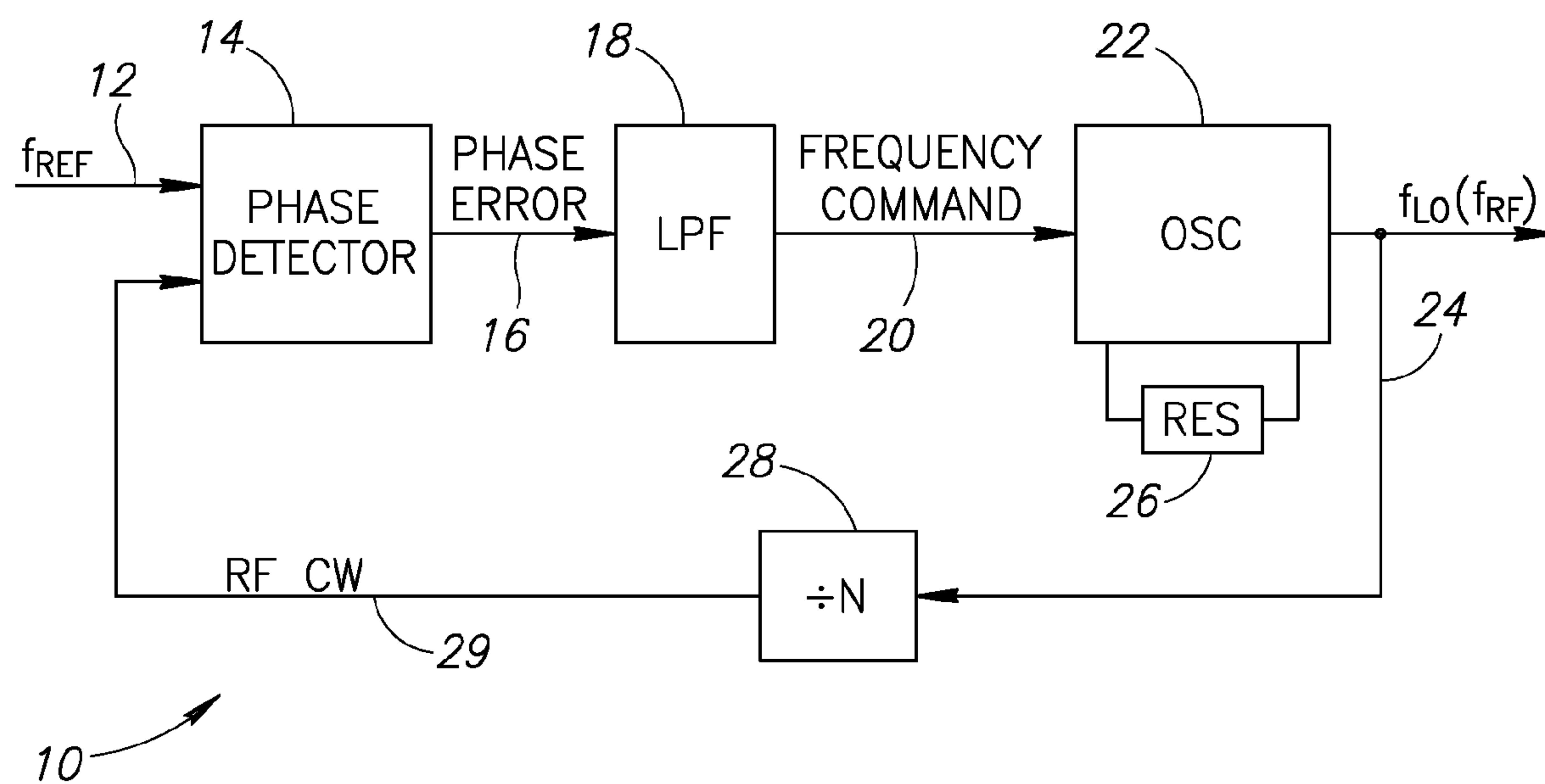
FIG. 1 (PRIOR ART)
