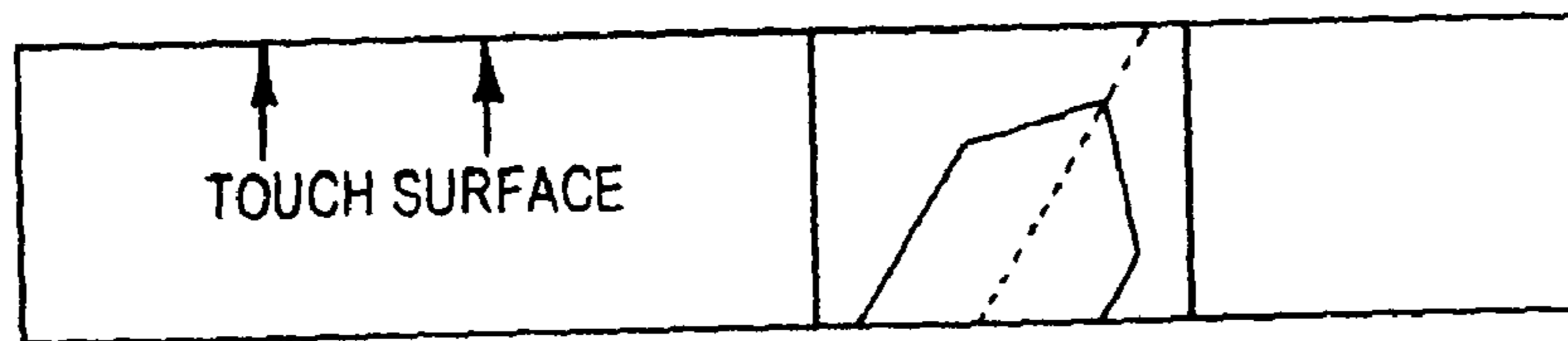
NON-PERPENDICULAR POINTER APPROACHING TOUCH SURFACE CALCULATED CENTER LINE SHOWS EXPECTED POINT OF CONTACT.
