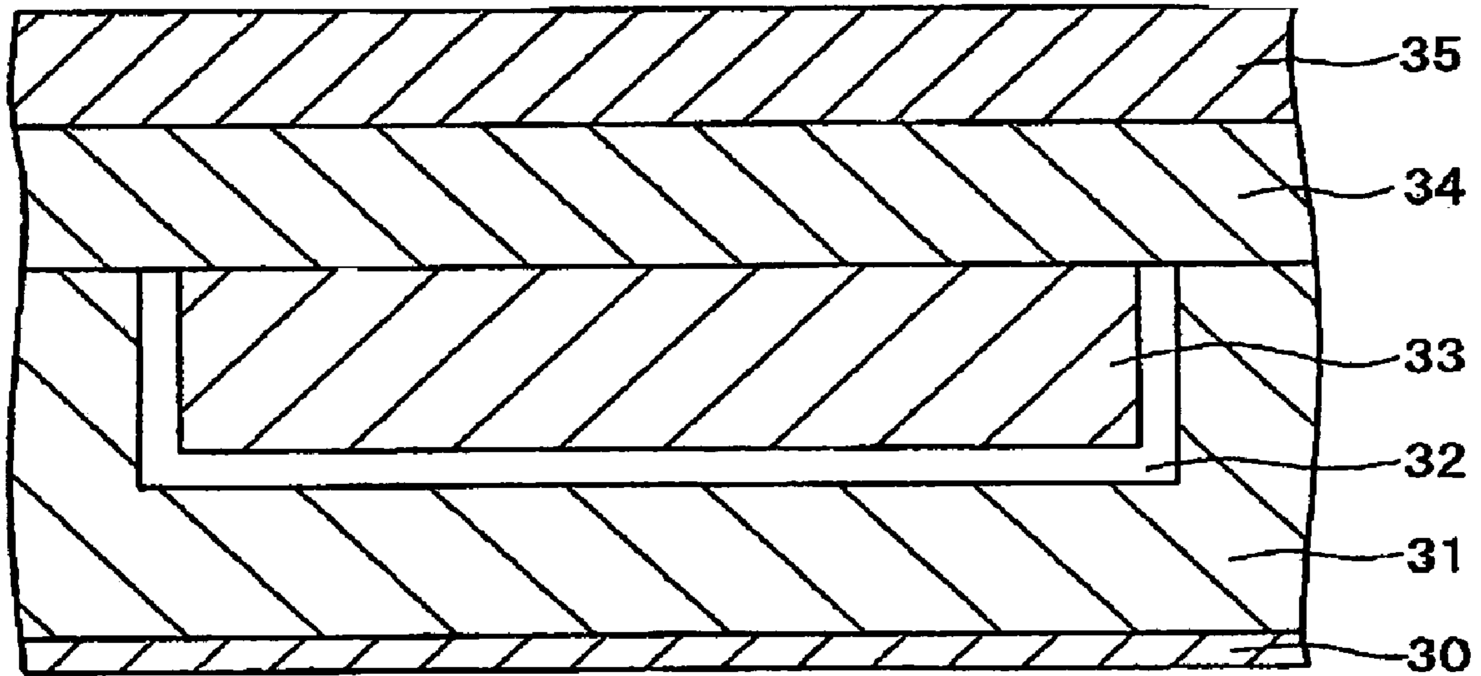
FIG. 12 (PRIOR ART)
