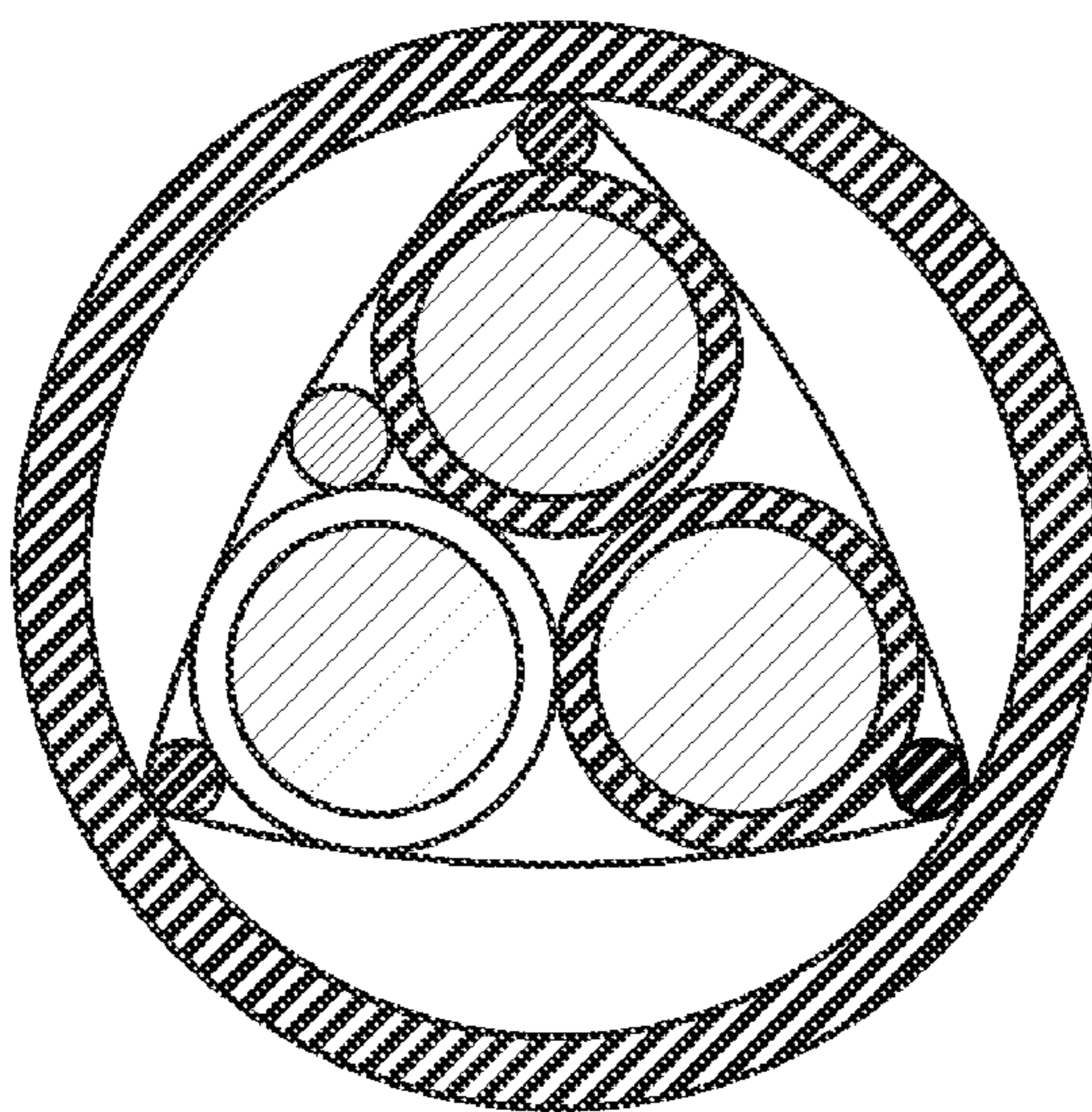
NO FILLER, CORDS UNDER NONMETALIC COVERING
