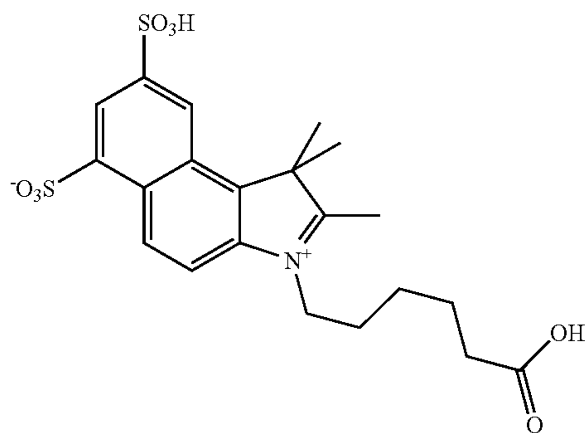
Example 28
