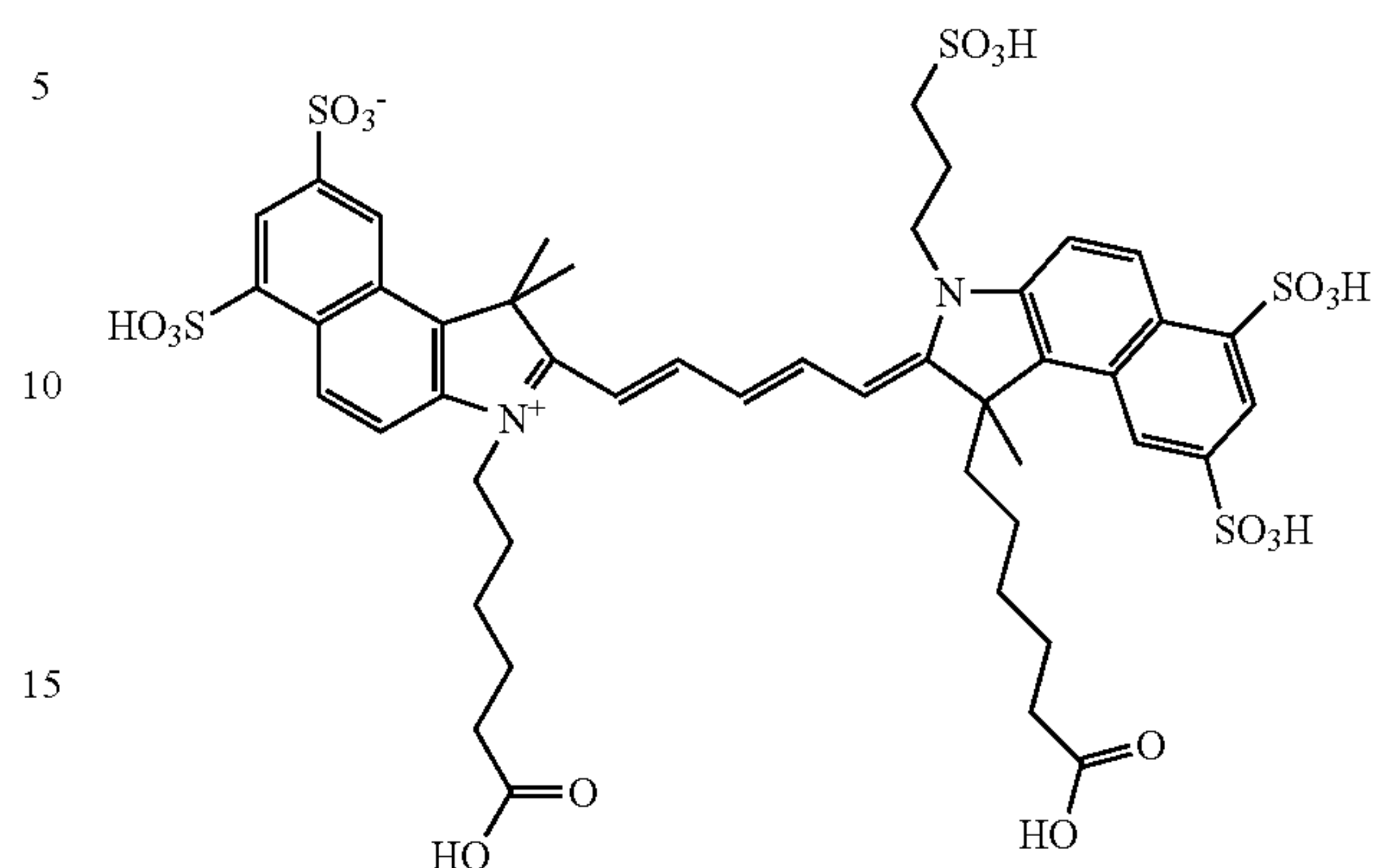
Compound 29
