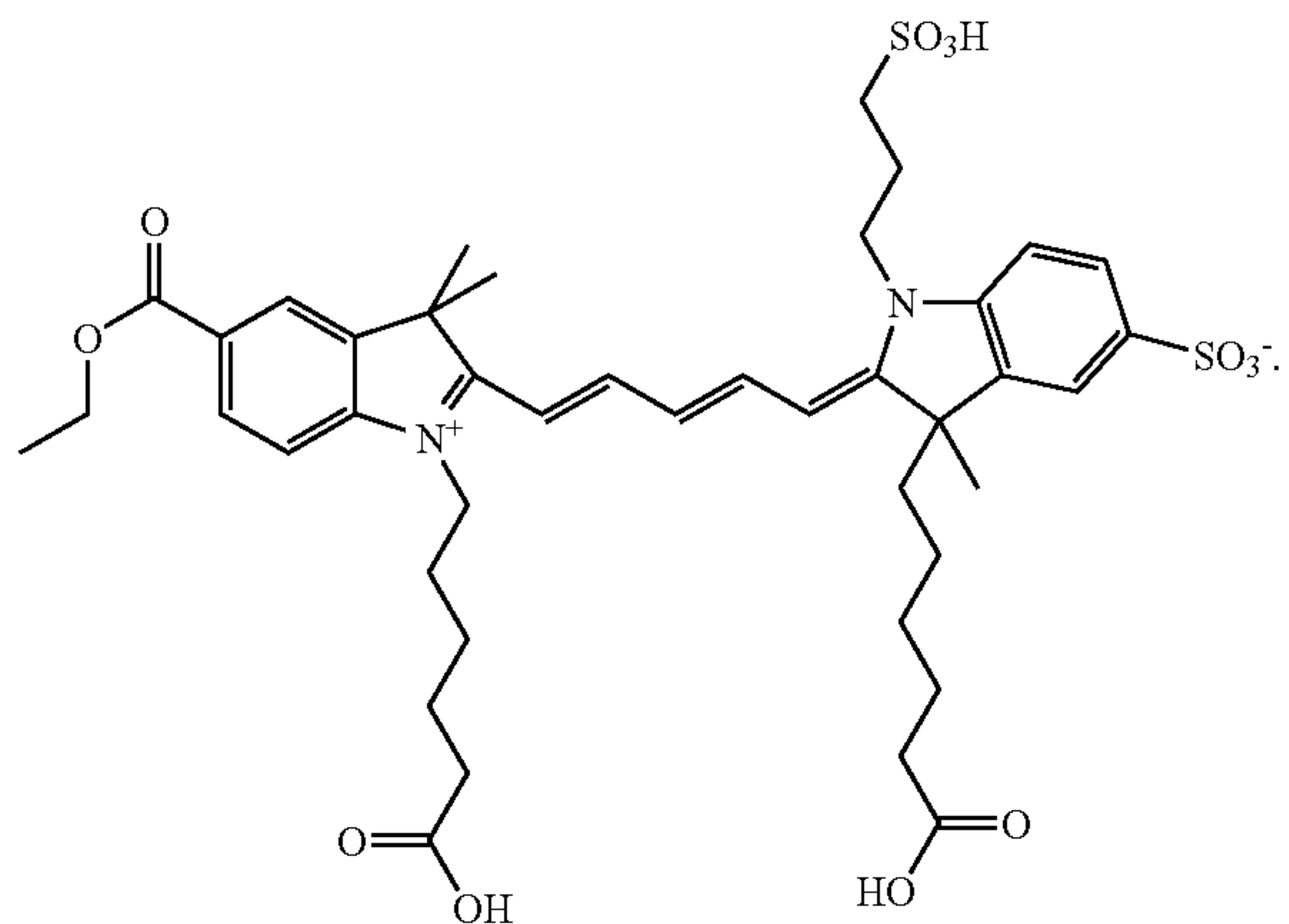
Compound 25
