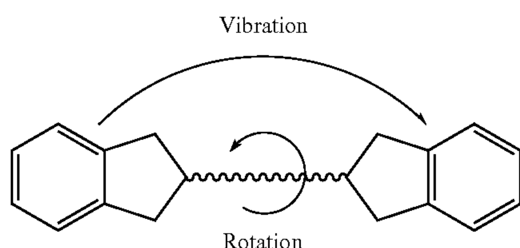
Scheme 1. 'Loose Belt Effect' through vibration and rotation around the middle conjugated double bonds
