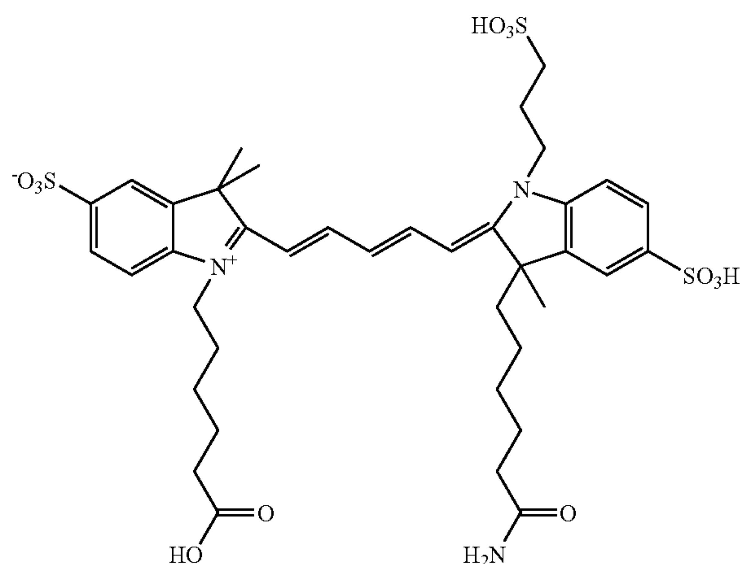
Compound 18
