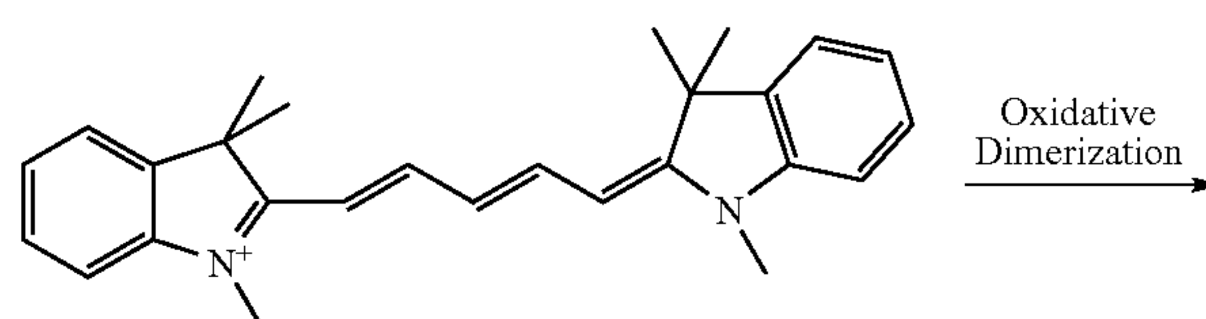
Scheme 2. Oxidation dimerization of carbocyanines
