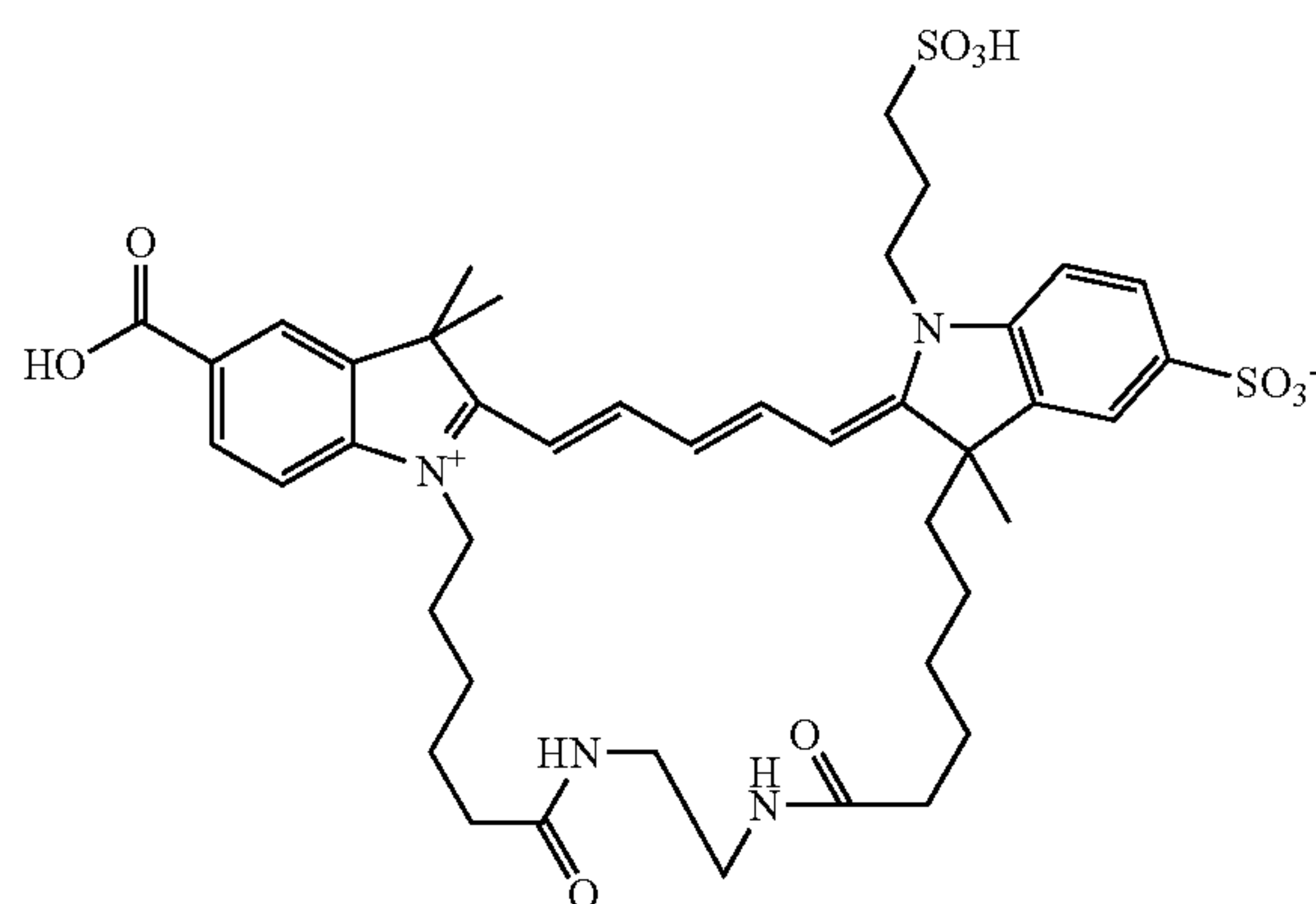
Compound 26
