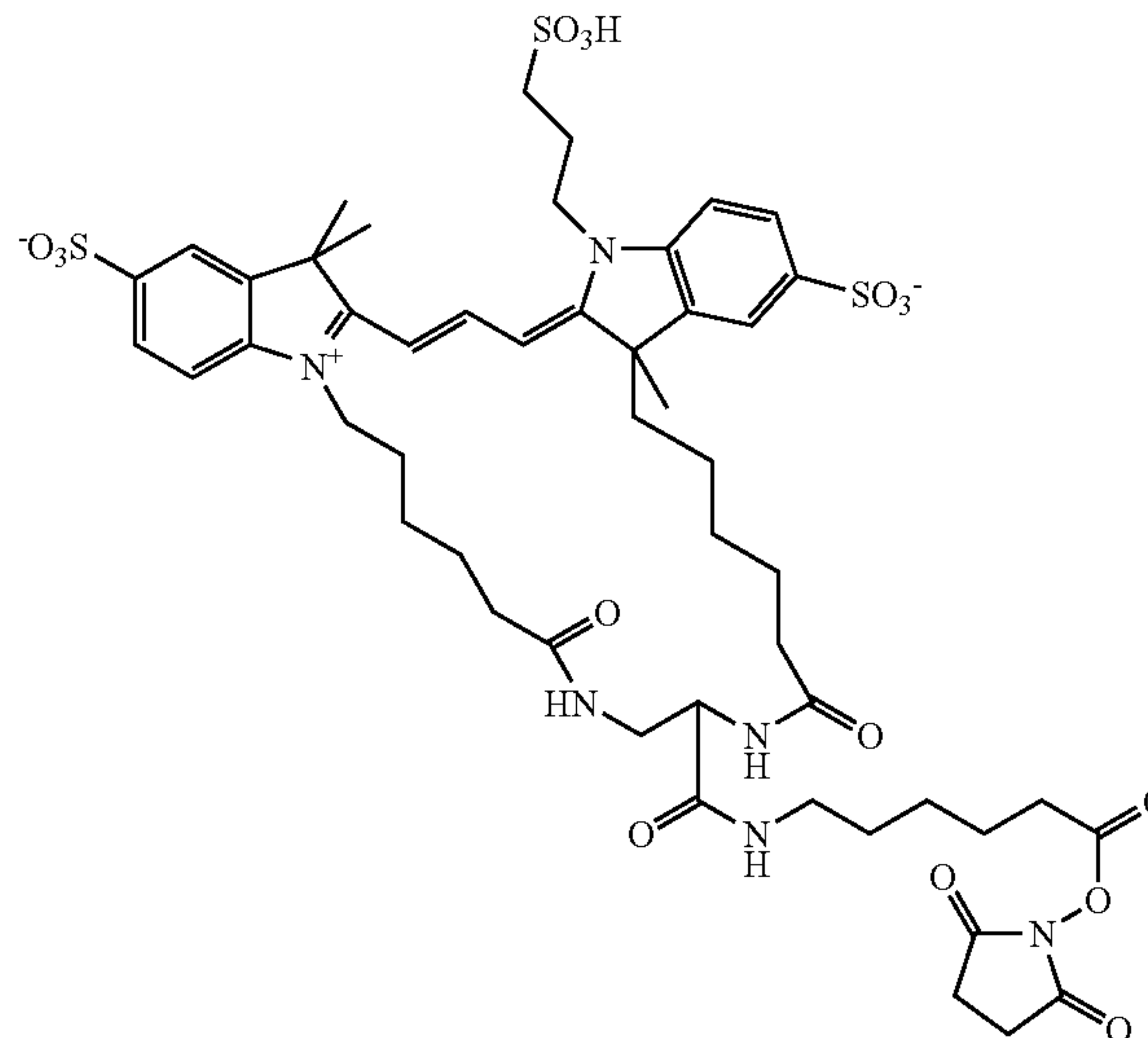
Compound 20
