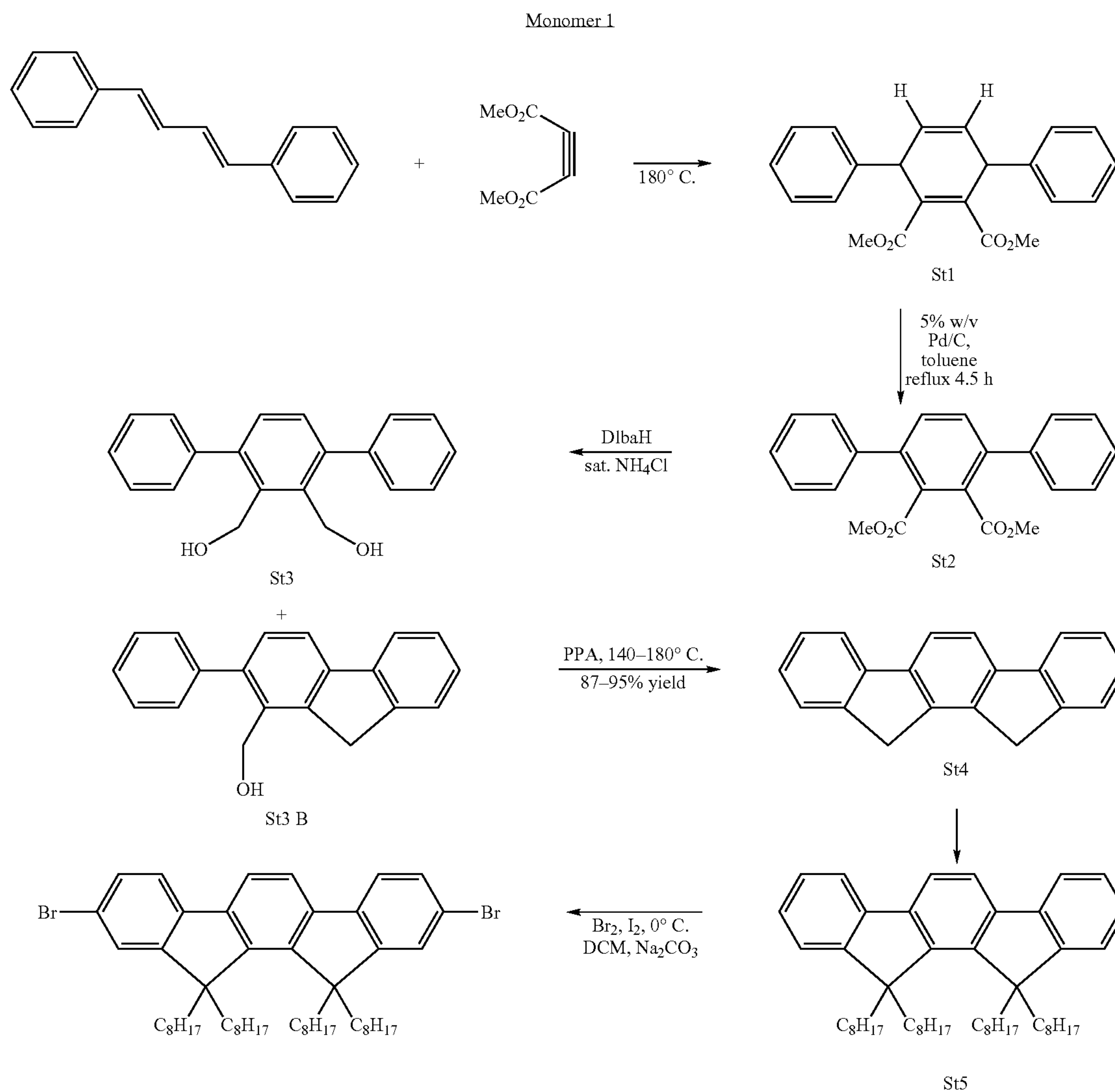
Synthesis of Diene, St1
