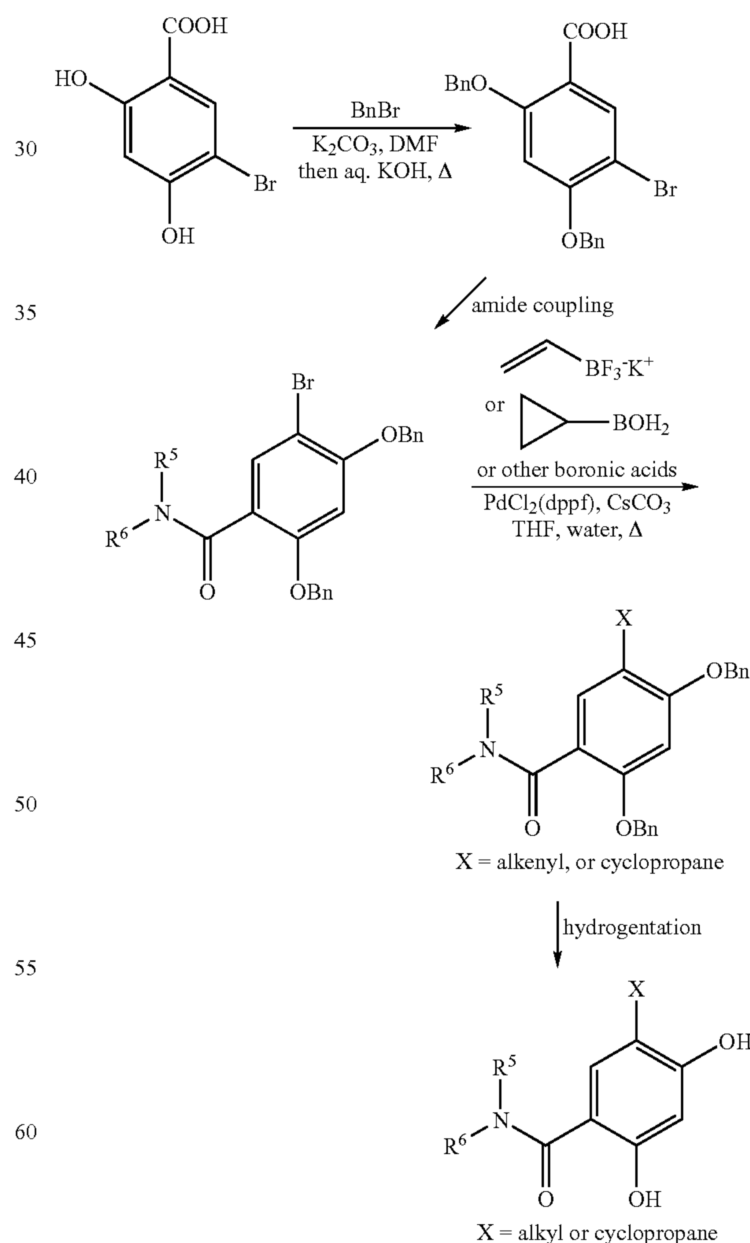
Scheme 6: 2,4-Dihydroxy-5-(alkyl)-benzoic acid amides
