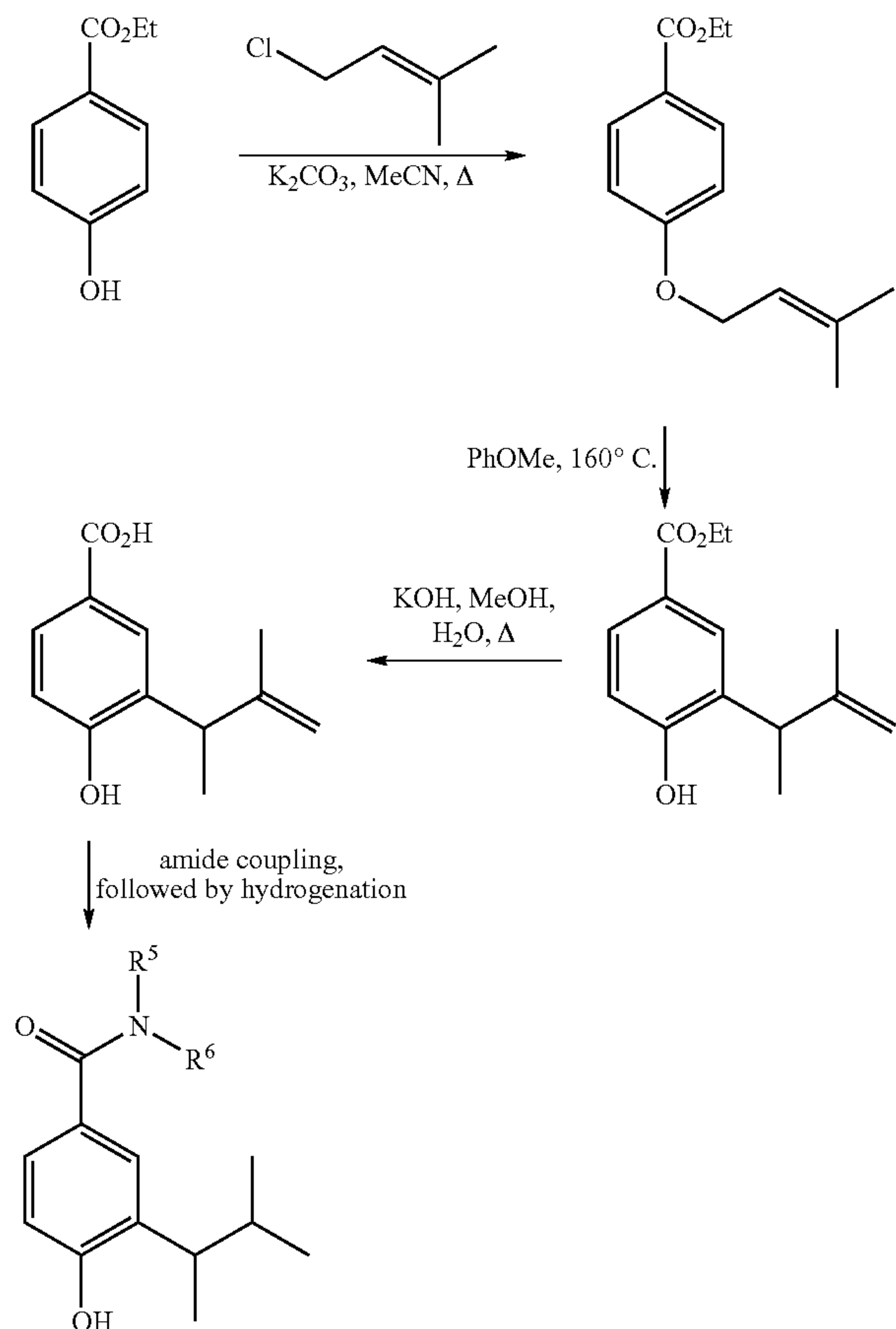
Scheme 5: 4-Hydroxy-3-(1',2'-dimethyl-propyl)-benzoic acid amides
