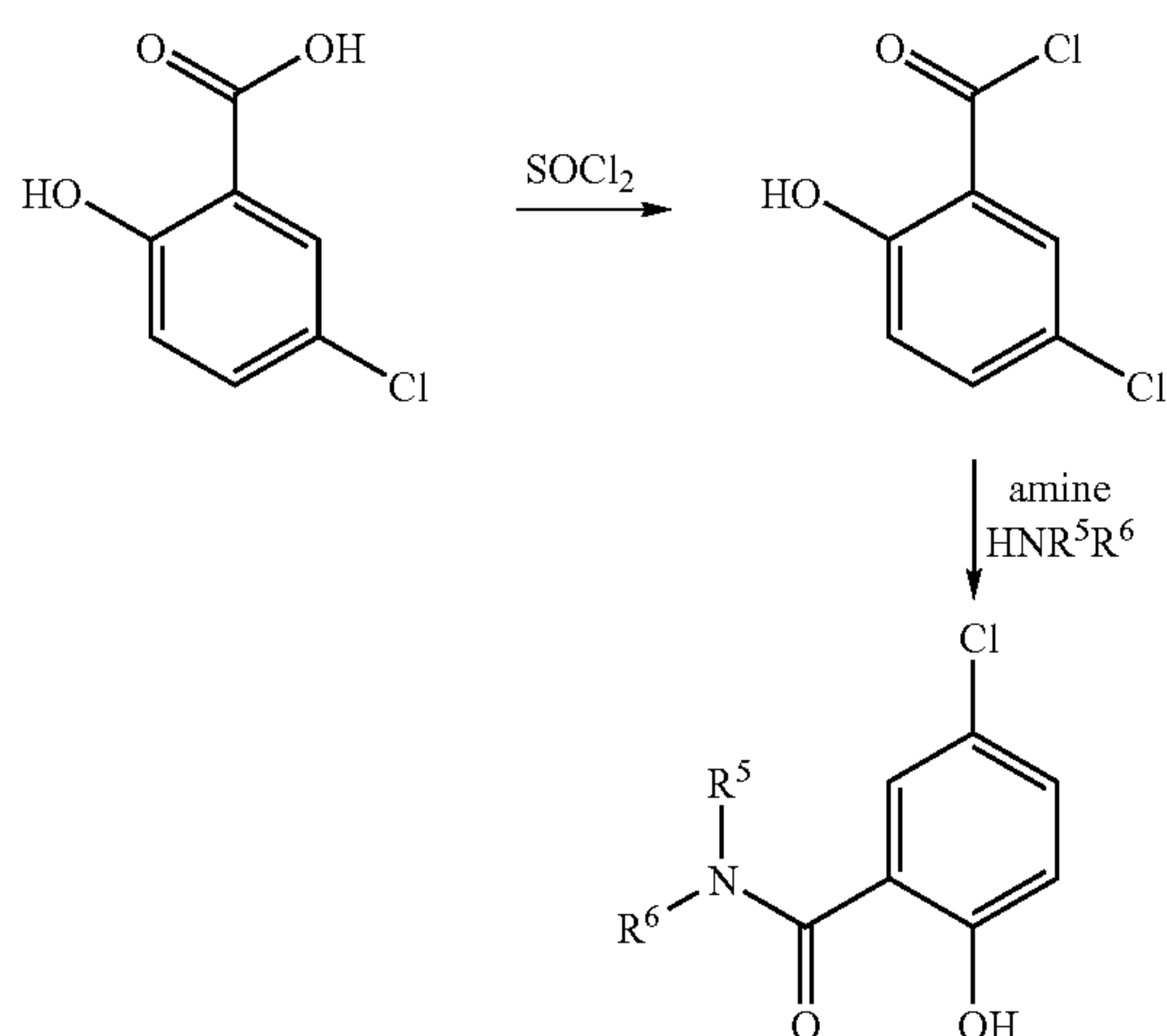
Scheme 1: 5-Chloro-2-hydroxybenzoic acid amides
