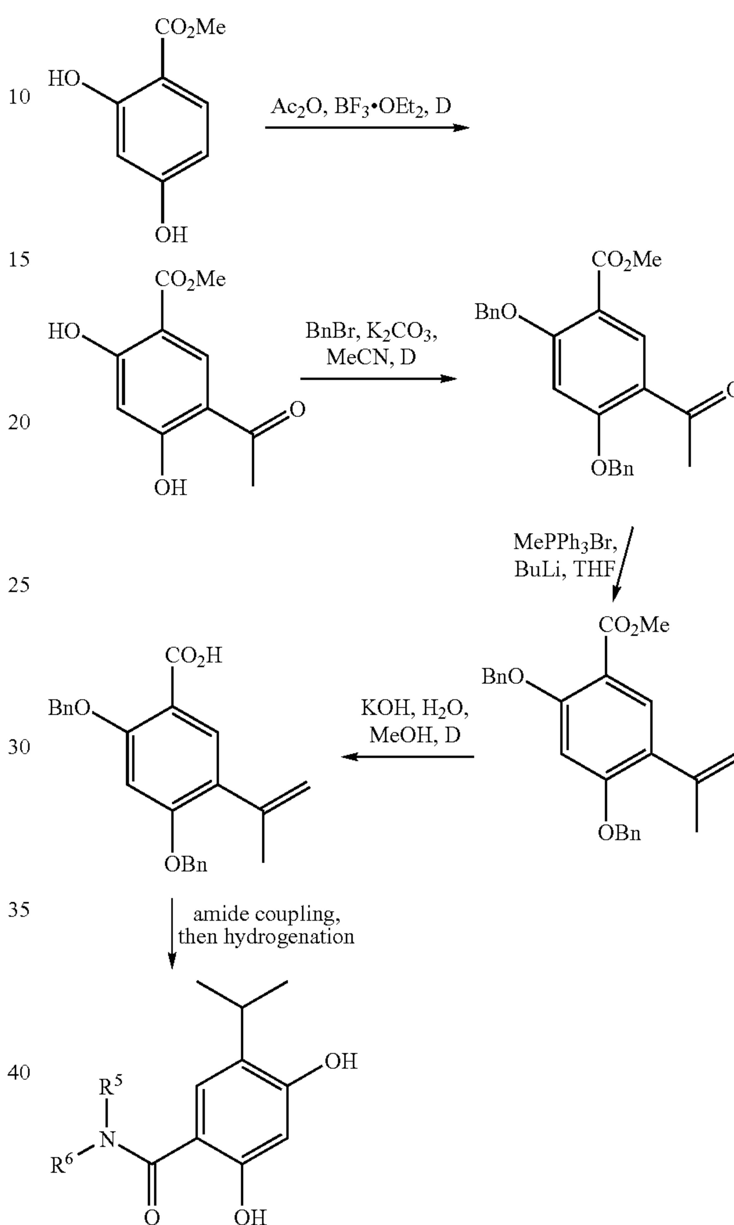
5 Scheme 4: 2,4-Dihydroxy-5-isopropyl-benzoic acid amides
