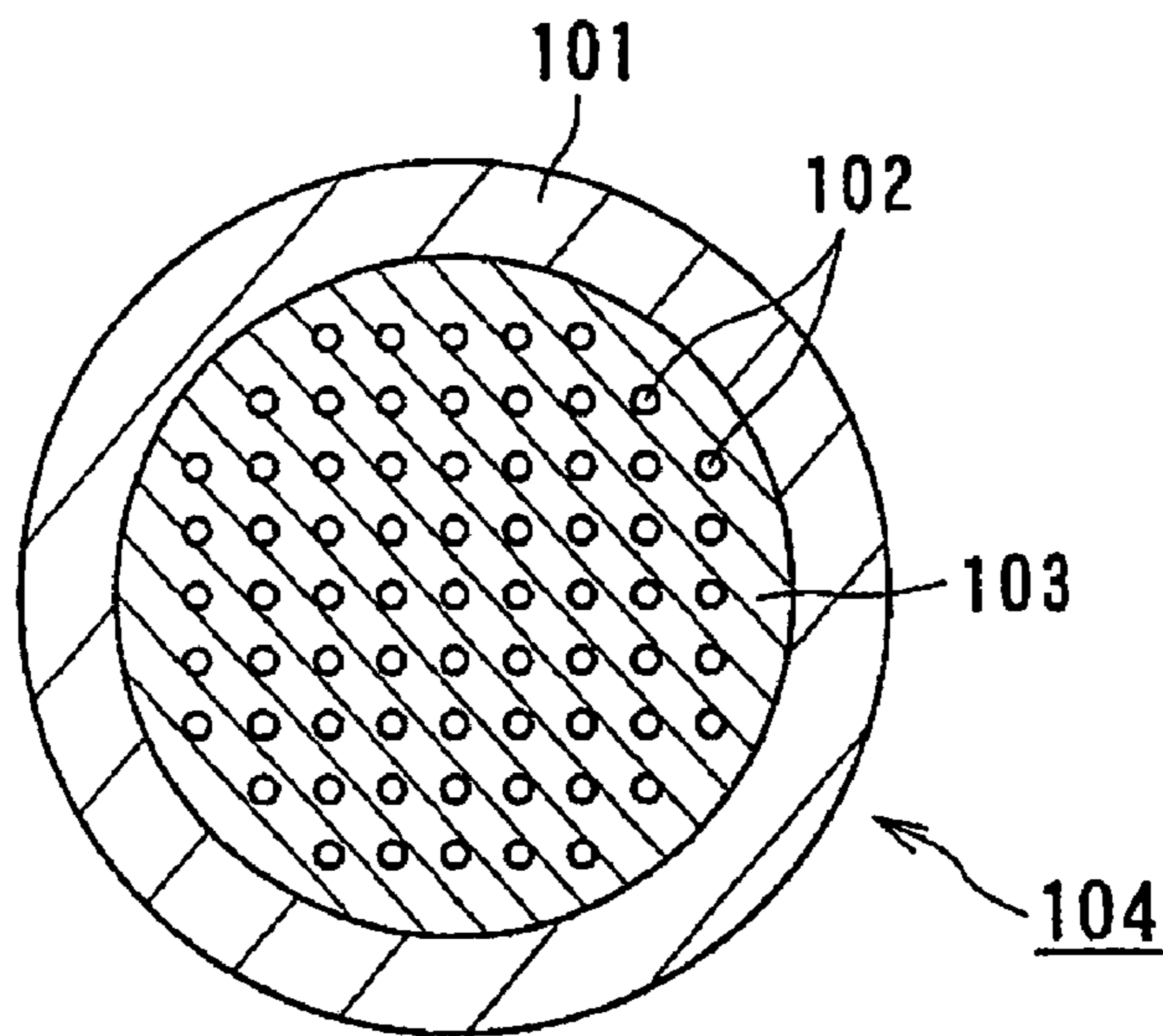
FIG. 21 PRIOR ART
