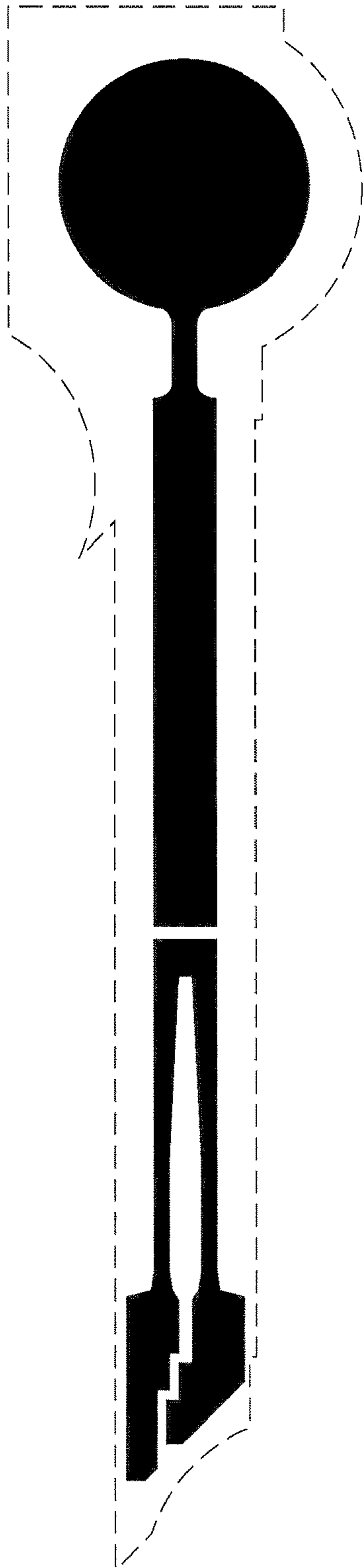
Heater mask
