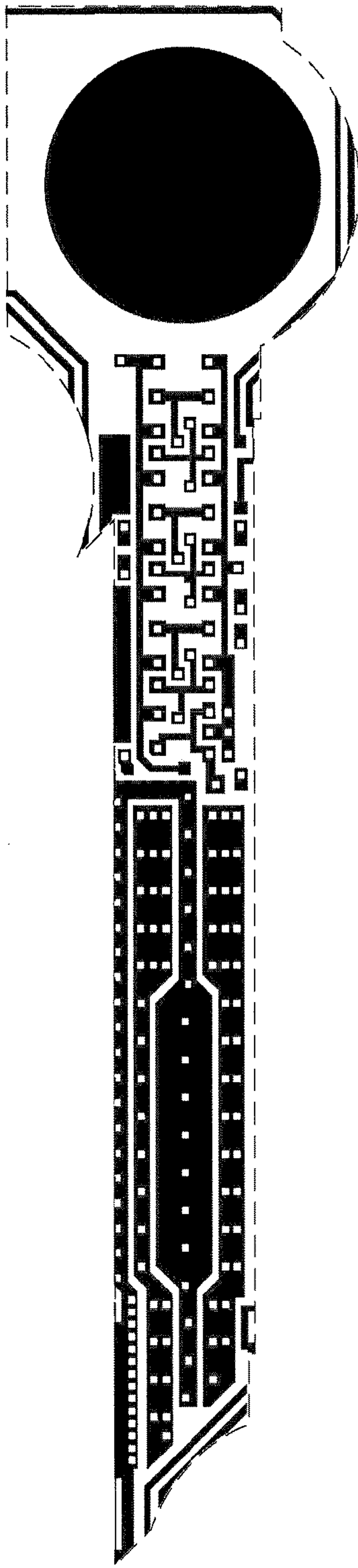
Metal 1 mask
