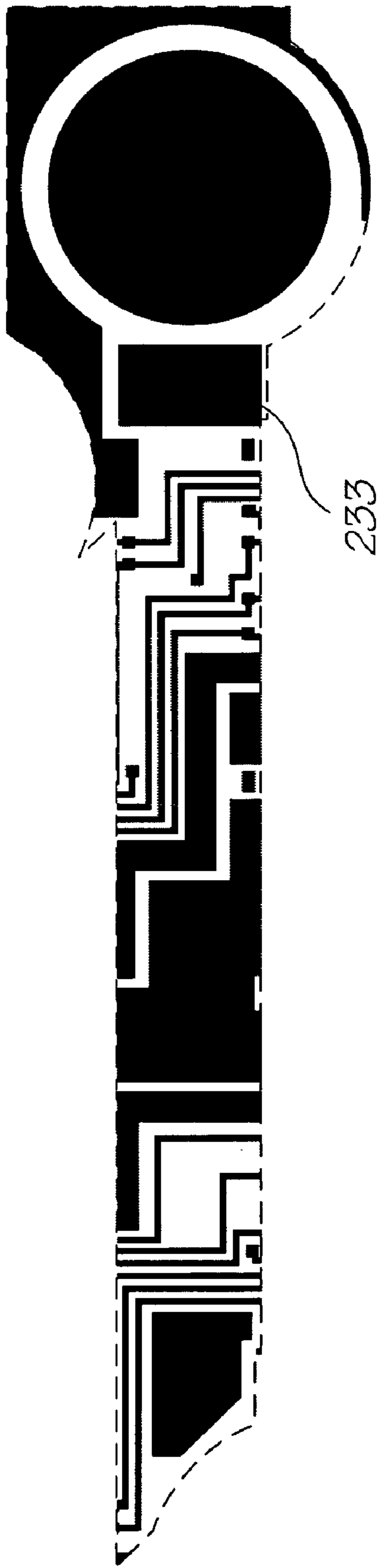
Metal 2 mask
