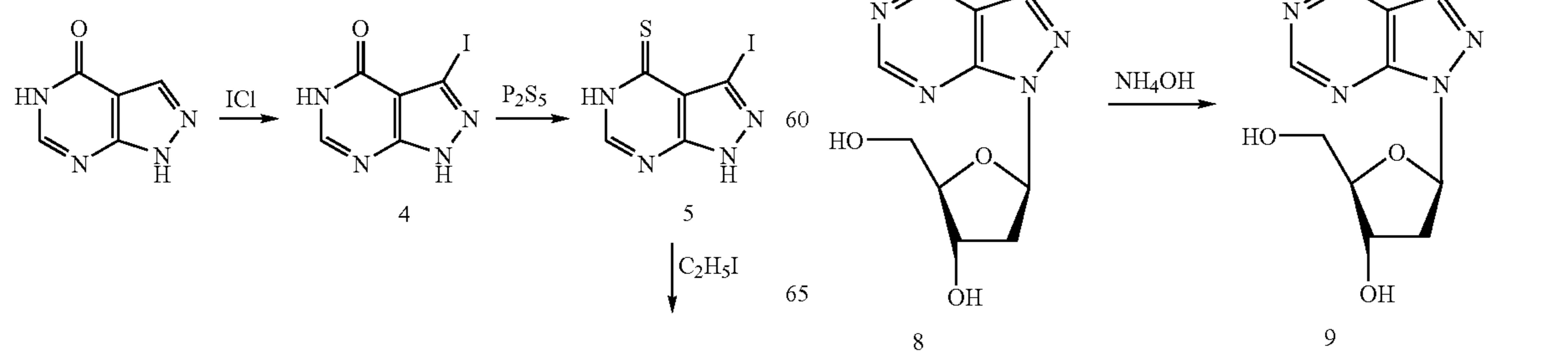
Reaction Scheme 2
