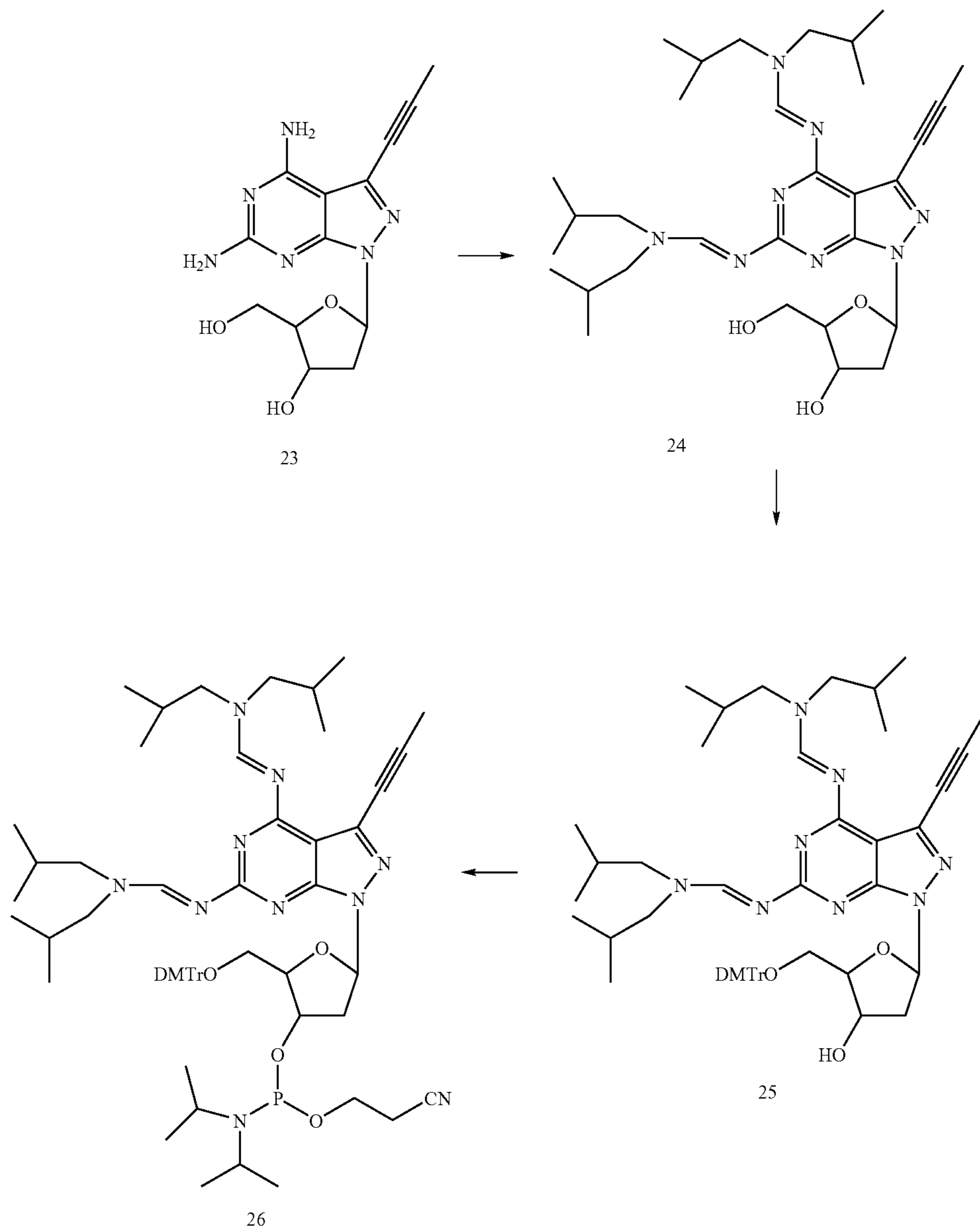
Reaction Scheme 5
