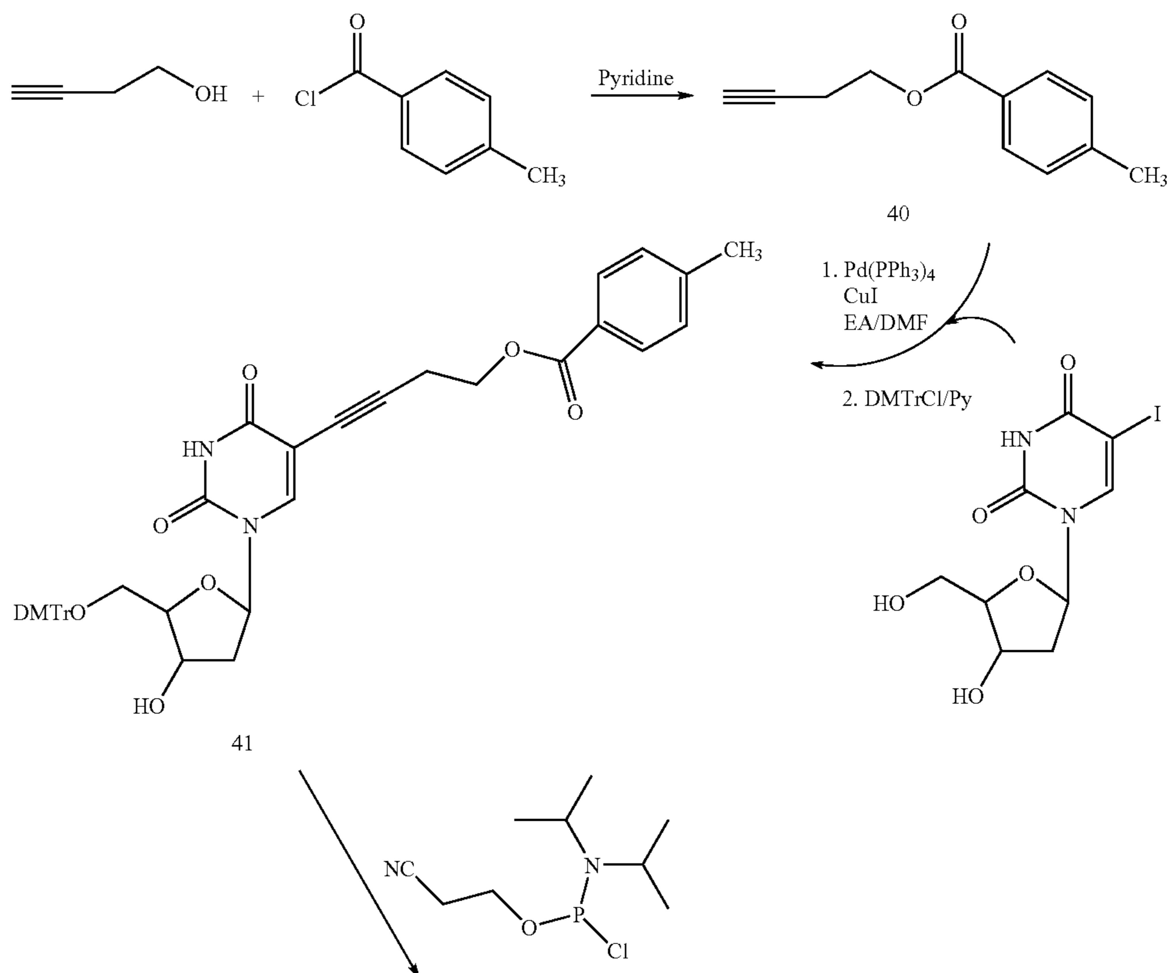
Reaction Scheme 10
