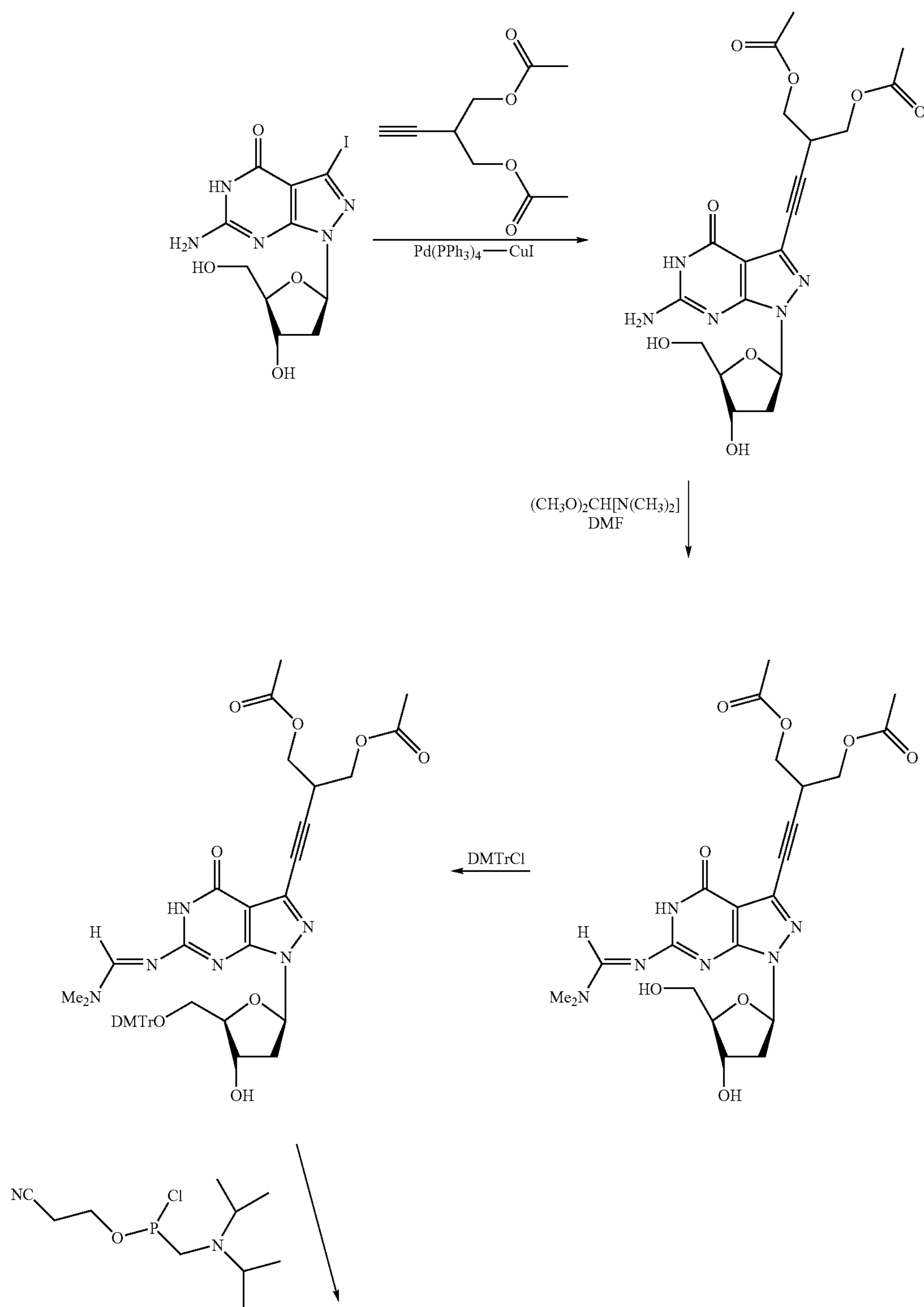
Reaction Scheme 6
