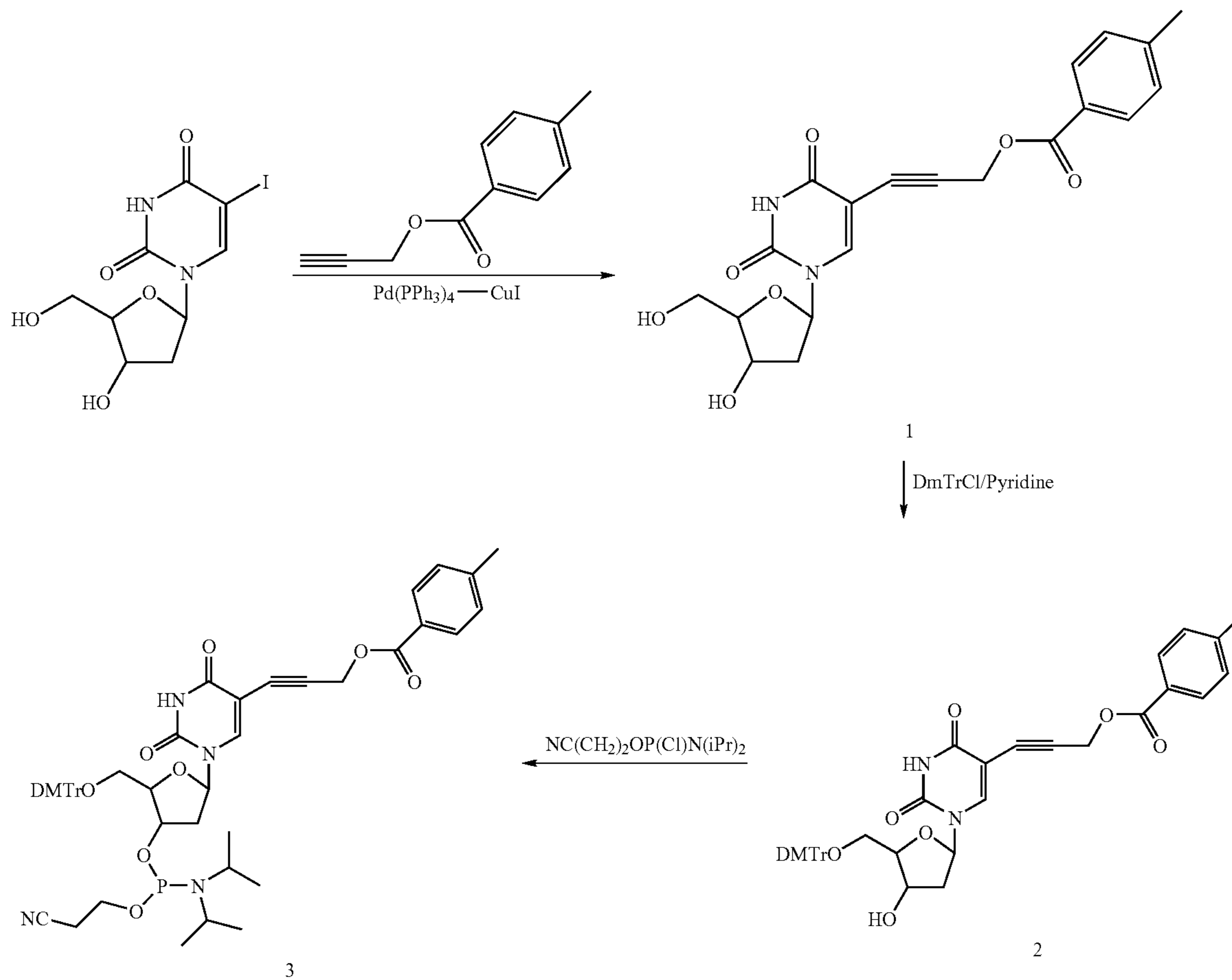
Reaction Scheme 1
