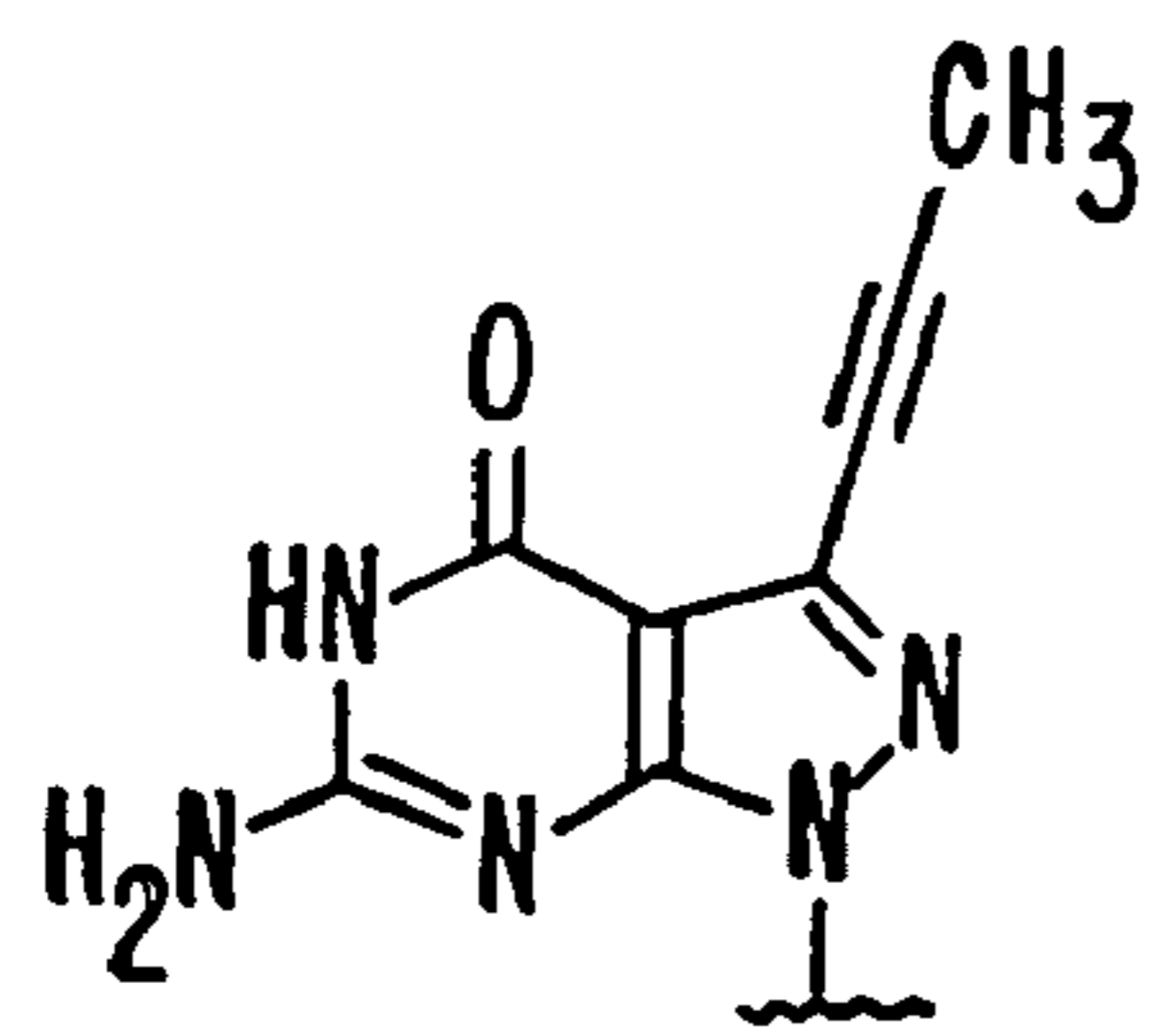
PPPG
