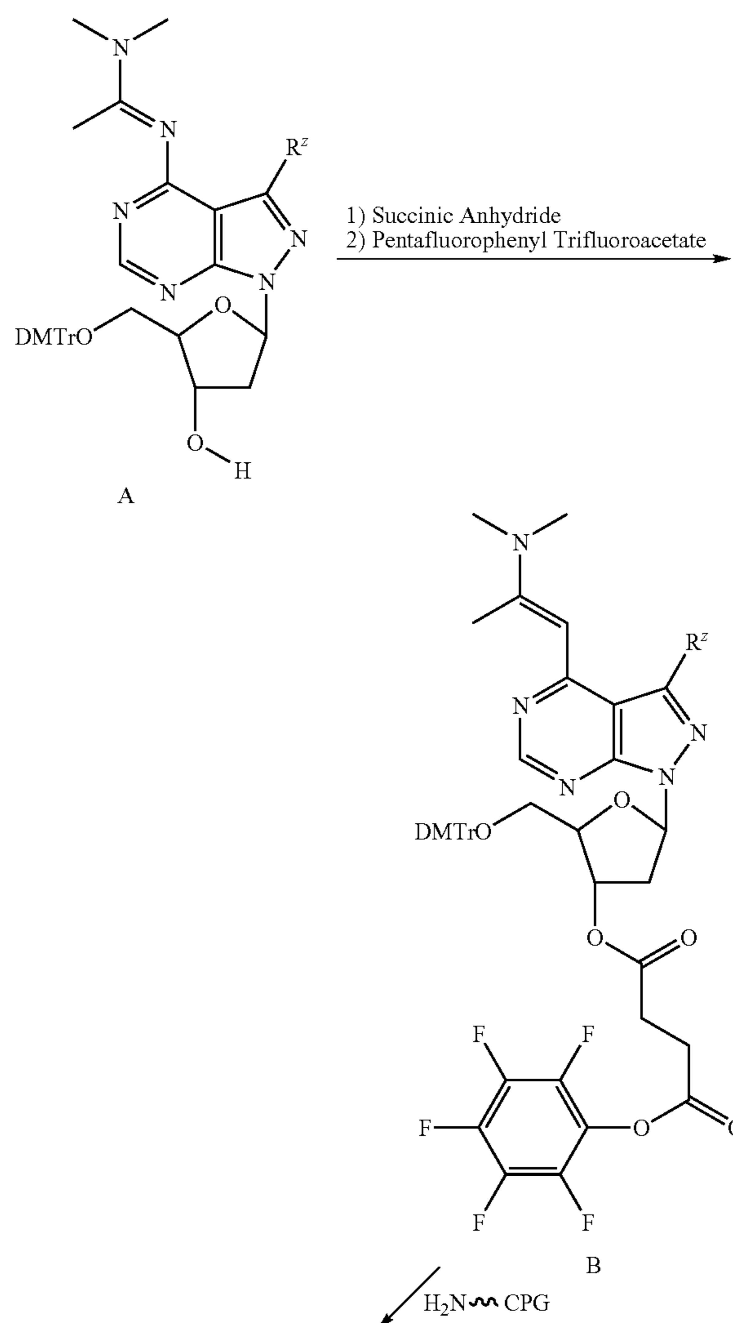
Reaction Scheme 11
