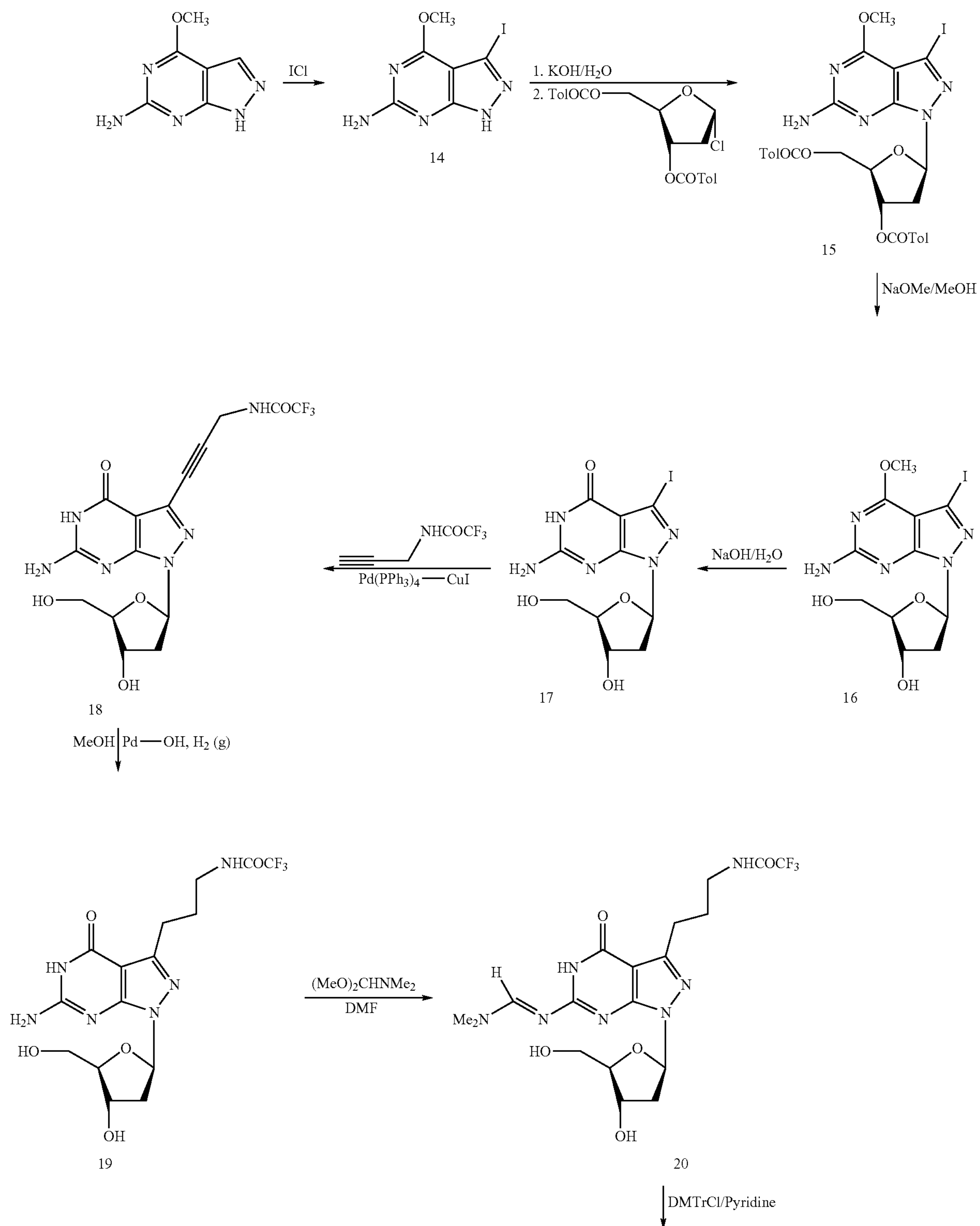
Reaction Scheme 4
