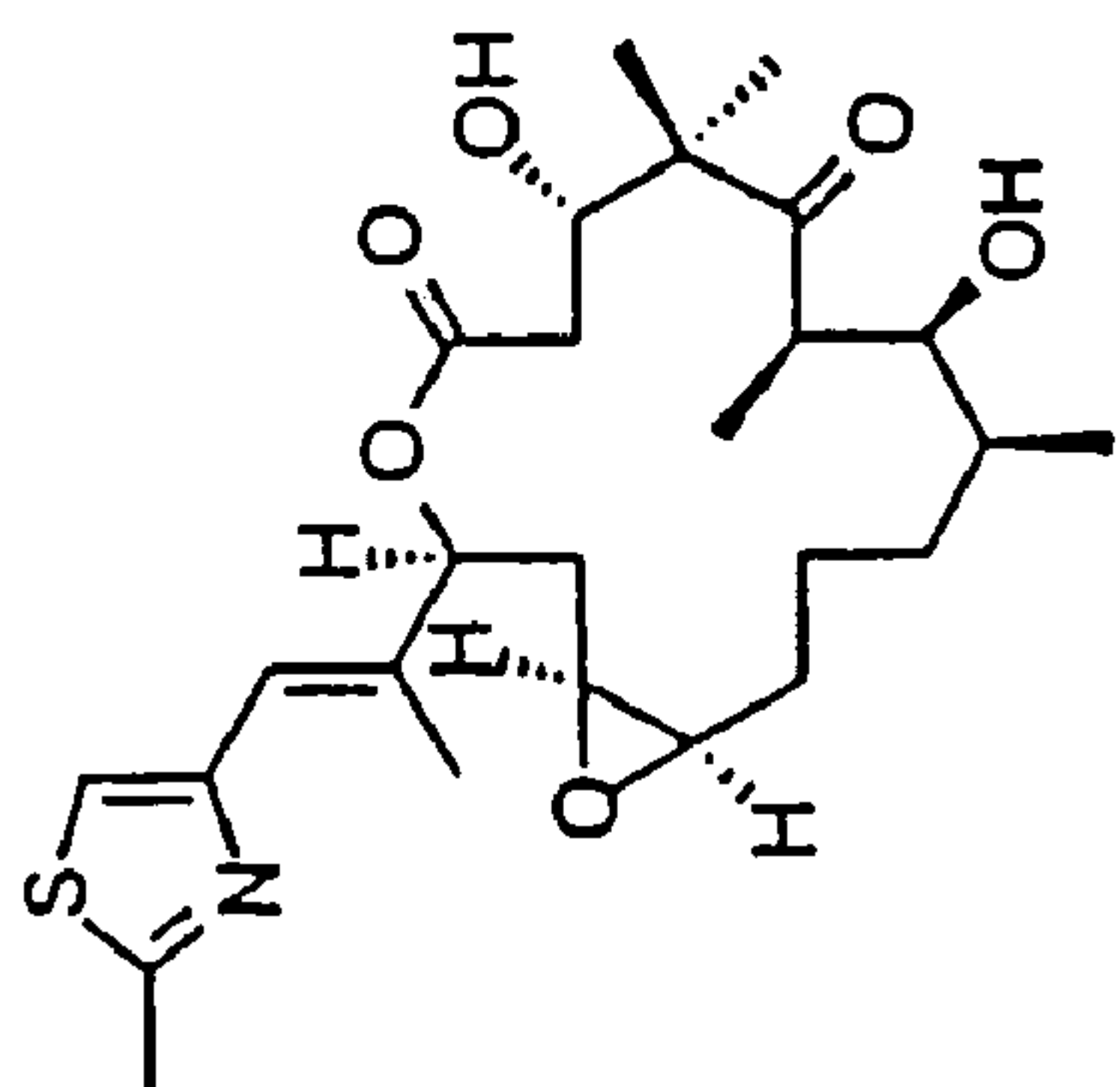
epothilone A
