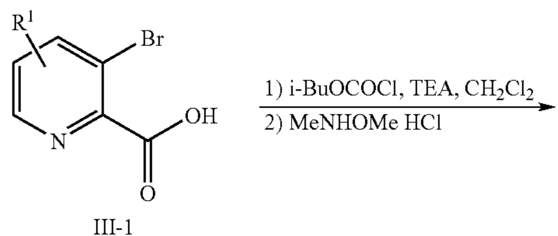
Reaction Scheme IV
