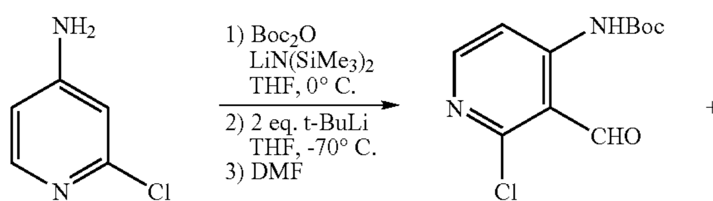
Reaction Scheme V
