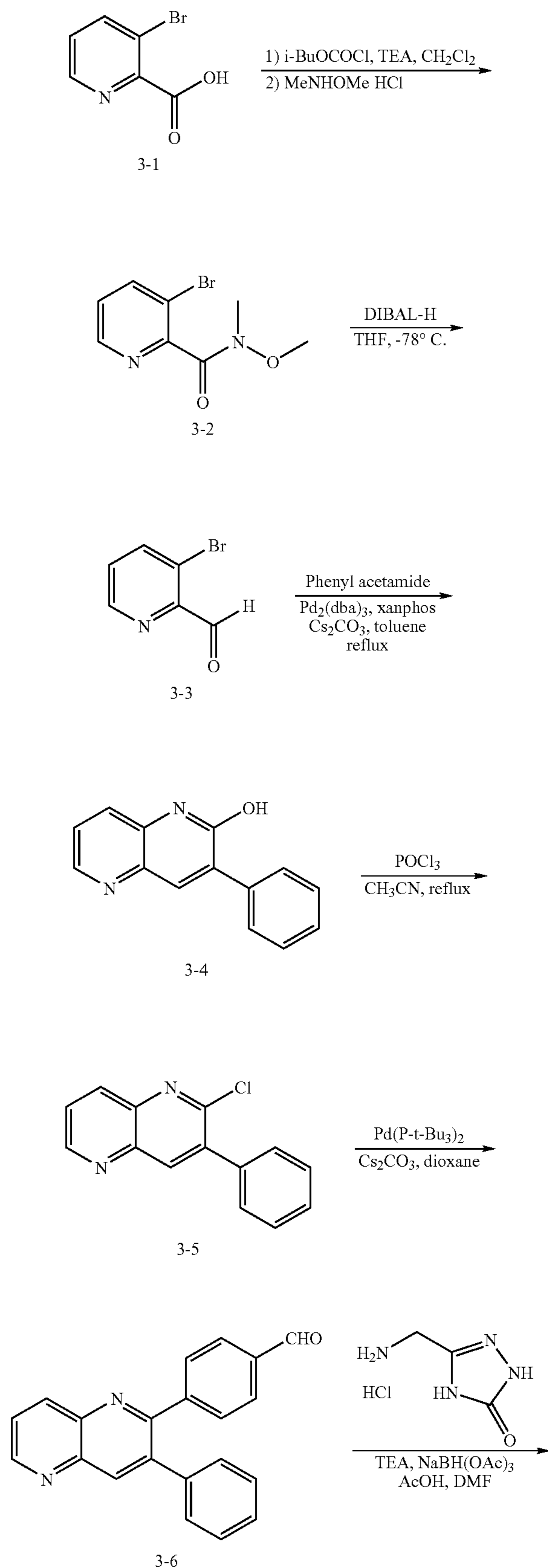
SCHEME 3
