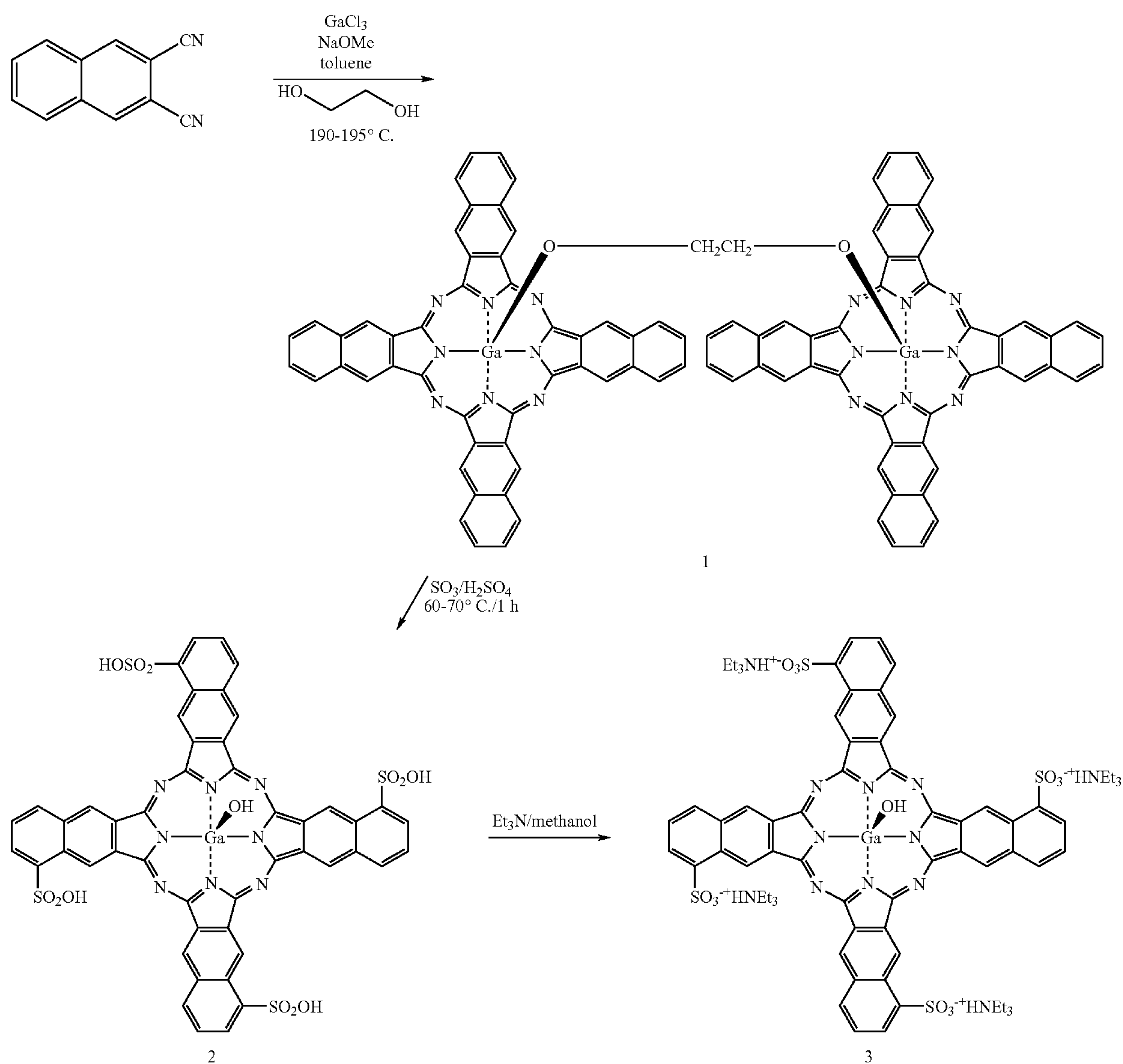
Scheme 1
