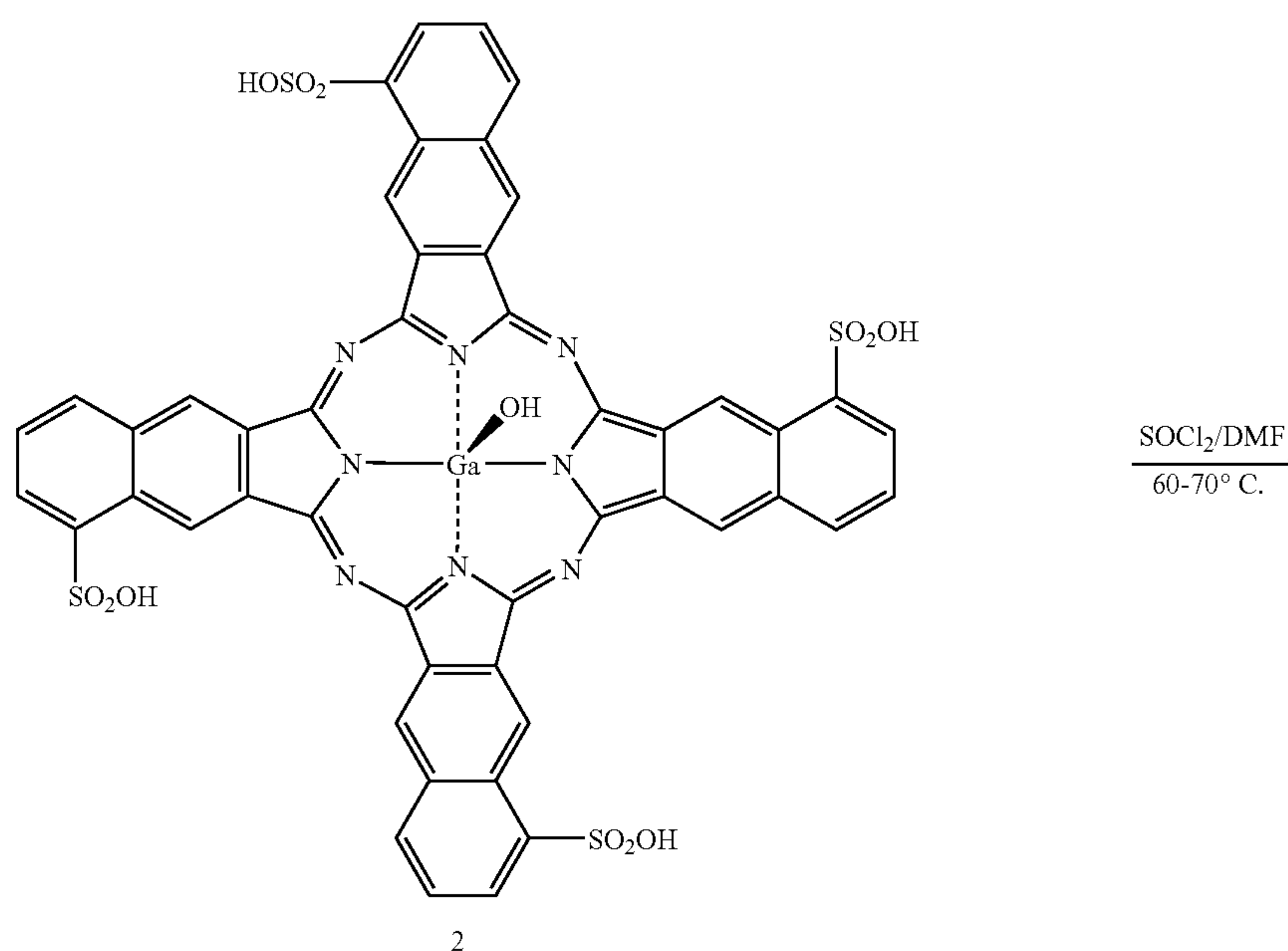
Scheme 2
