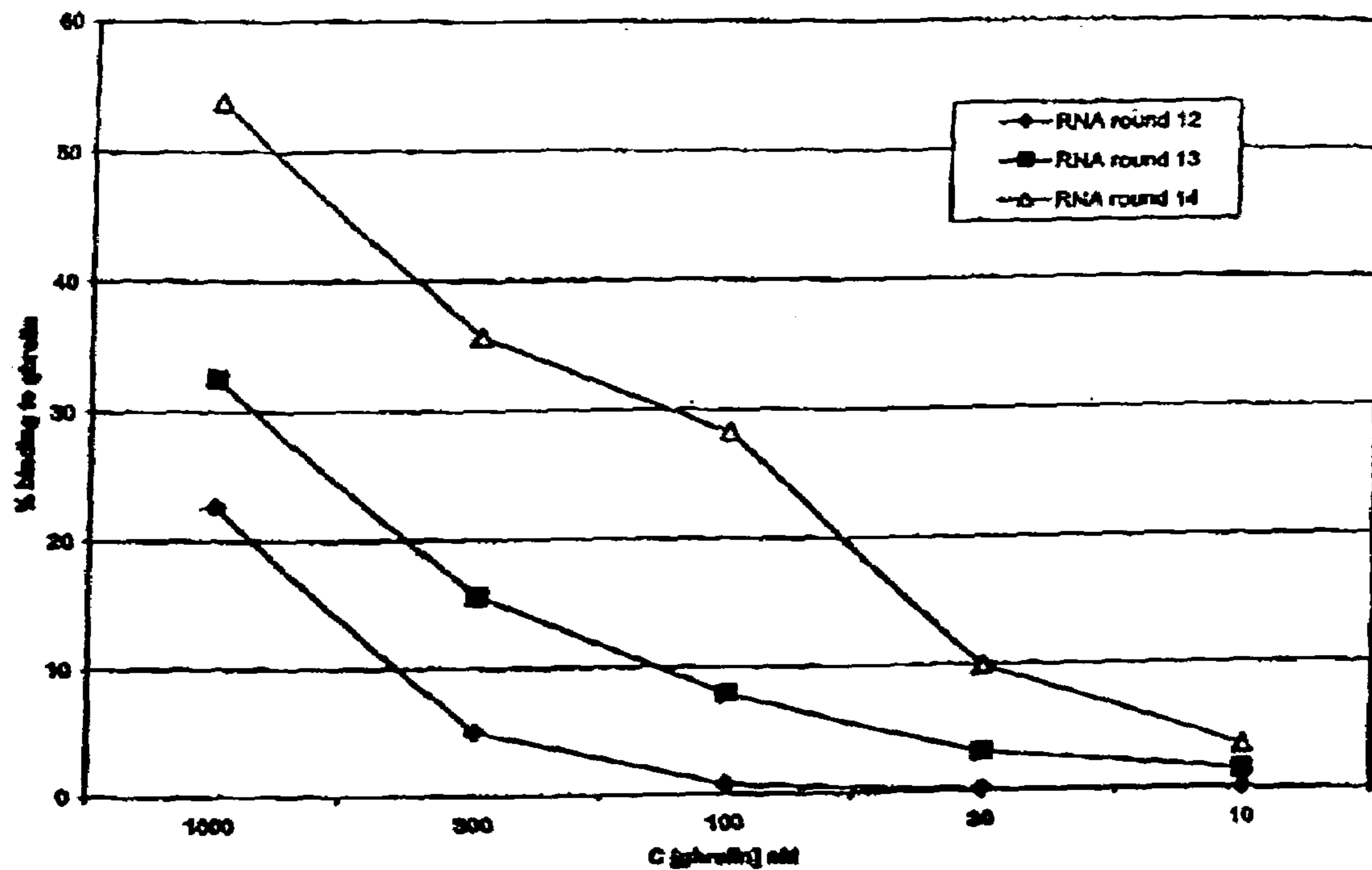
Fig.7B: Improvement of the RNA pool binding to D-ghrelin monitored over the double rounds
