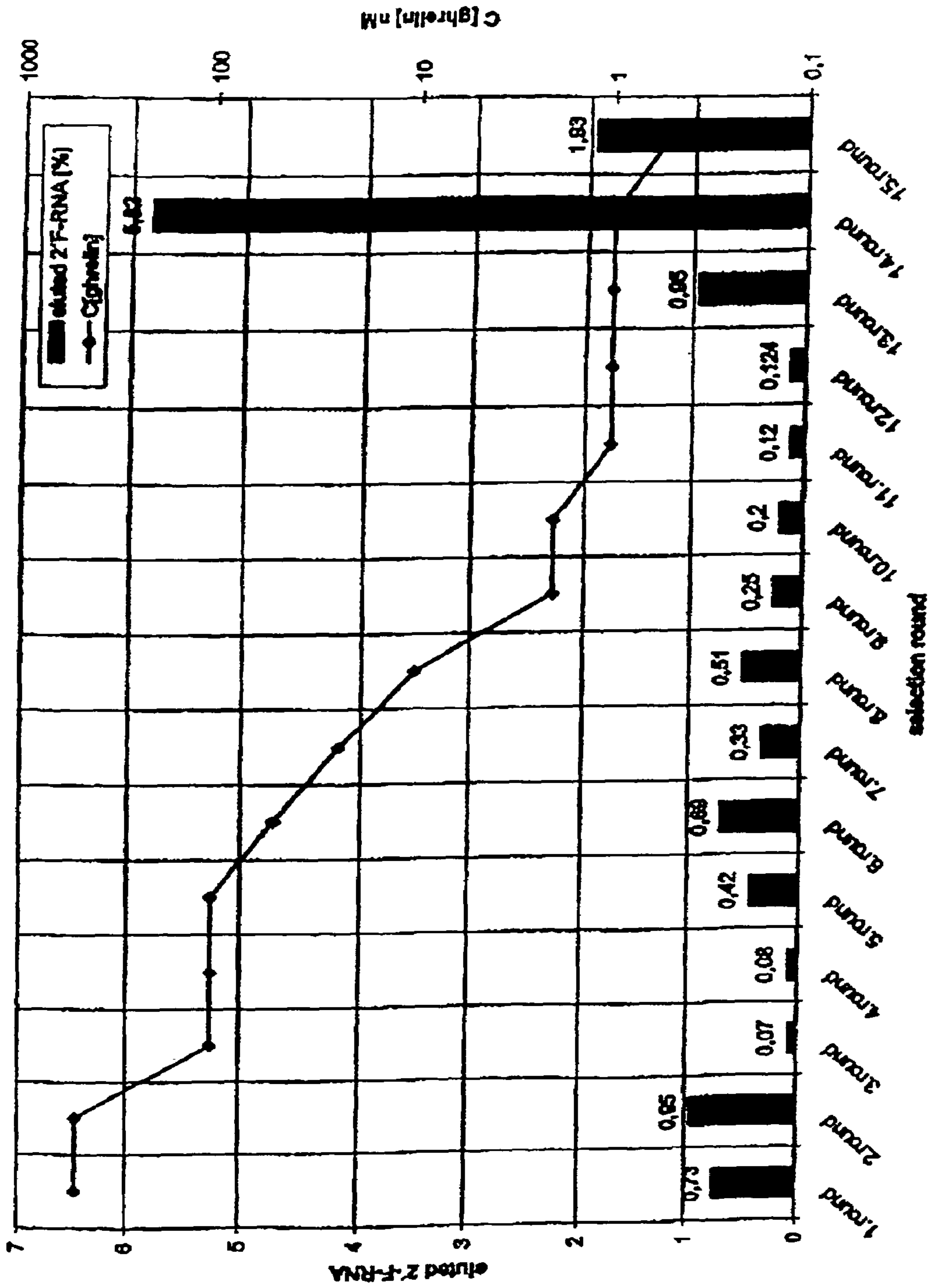
Fig.6: course of eluted 2'-F-RNA in percent of total used 2'-F-RNA and peptide concentration
