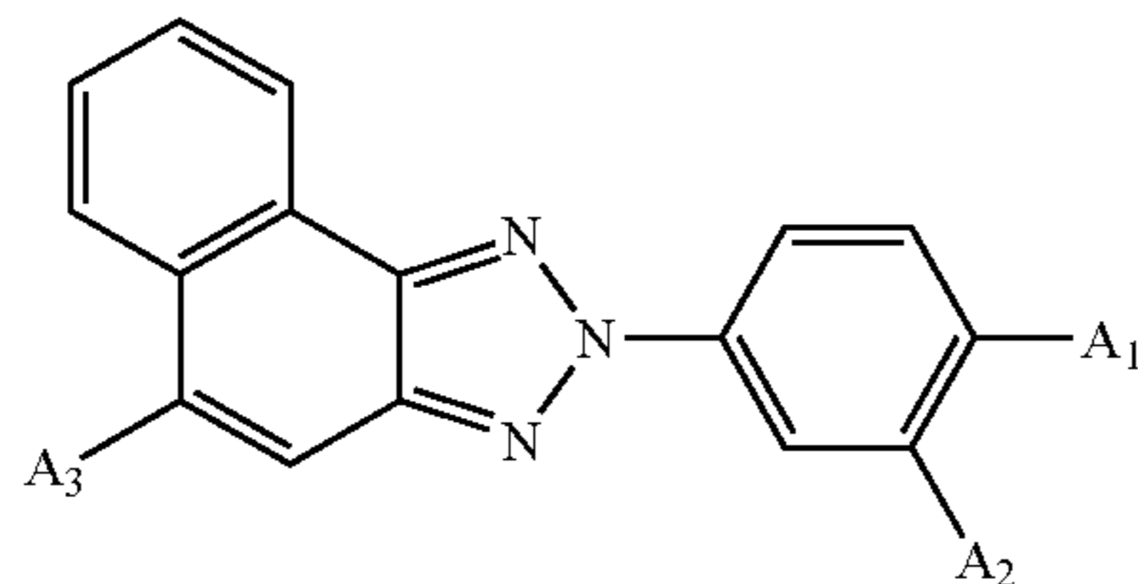
Monomer 5:
