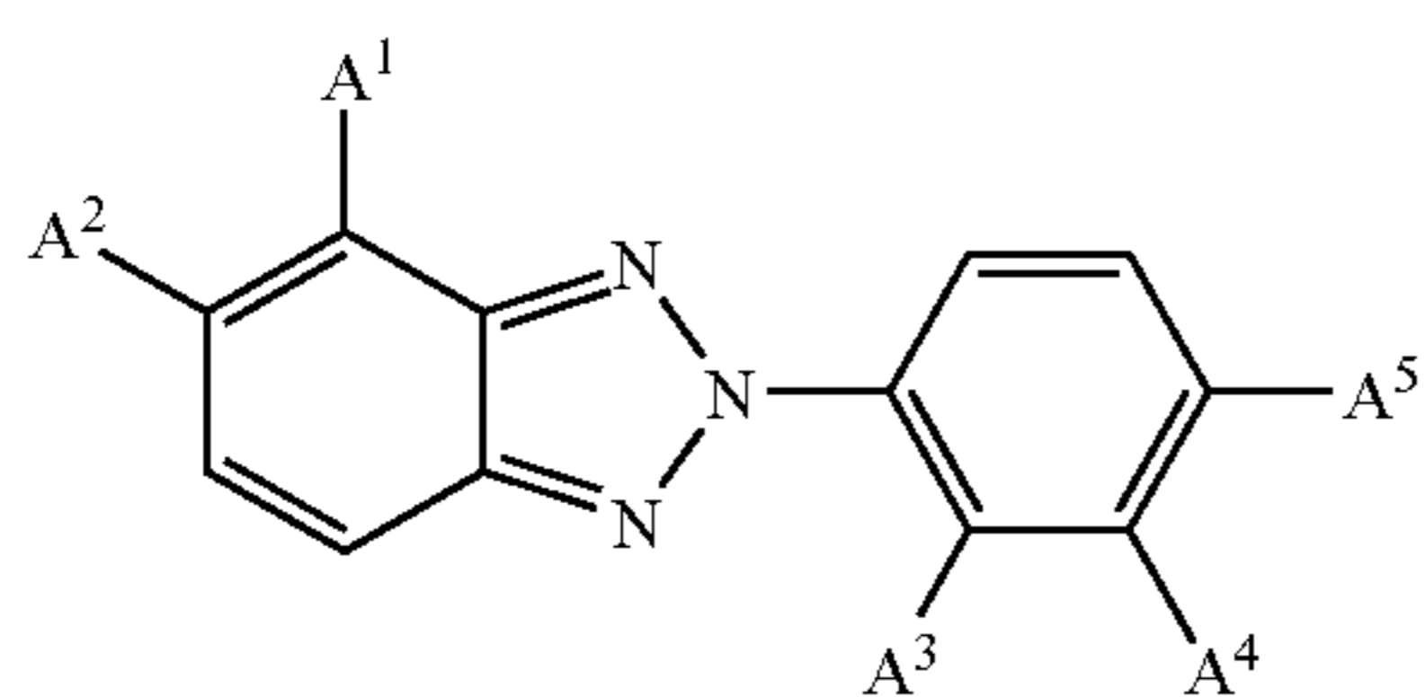
Monomer 1:
