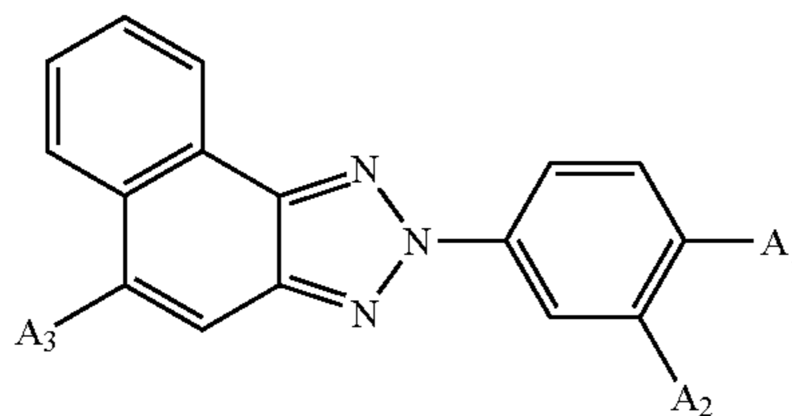
Monomer 5:
