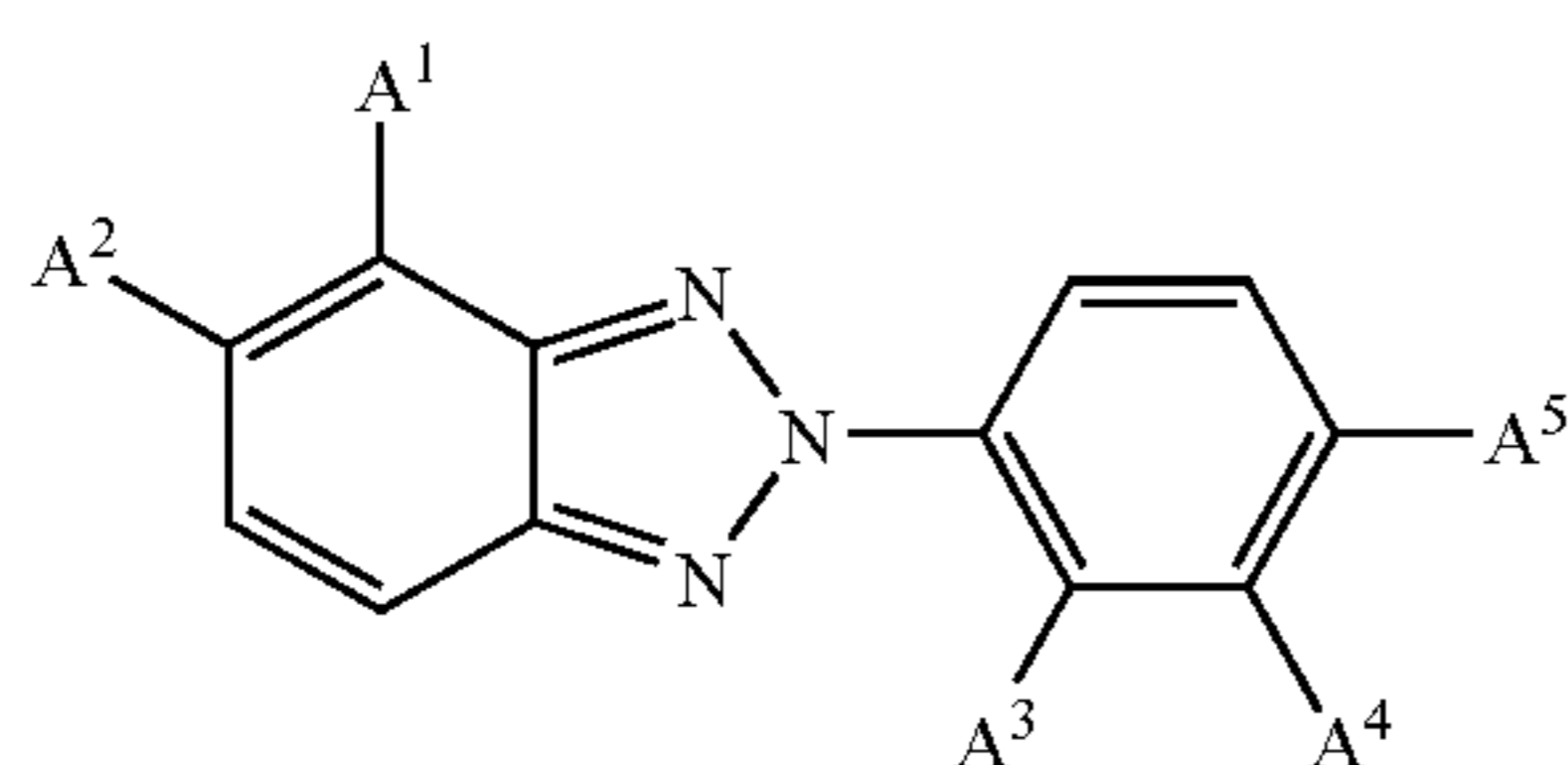
Monomer 3:
