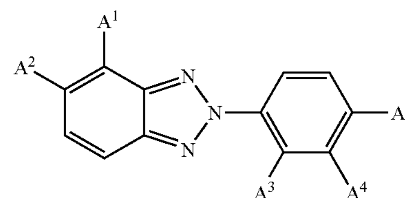
Monomer 3:
