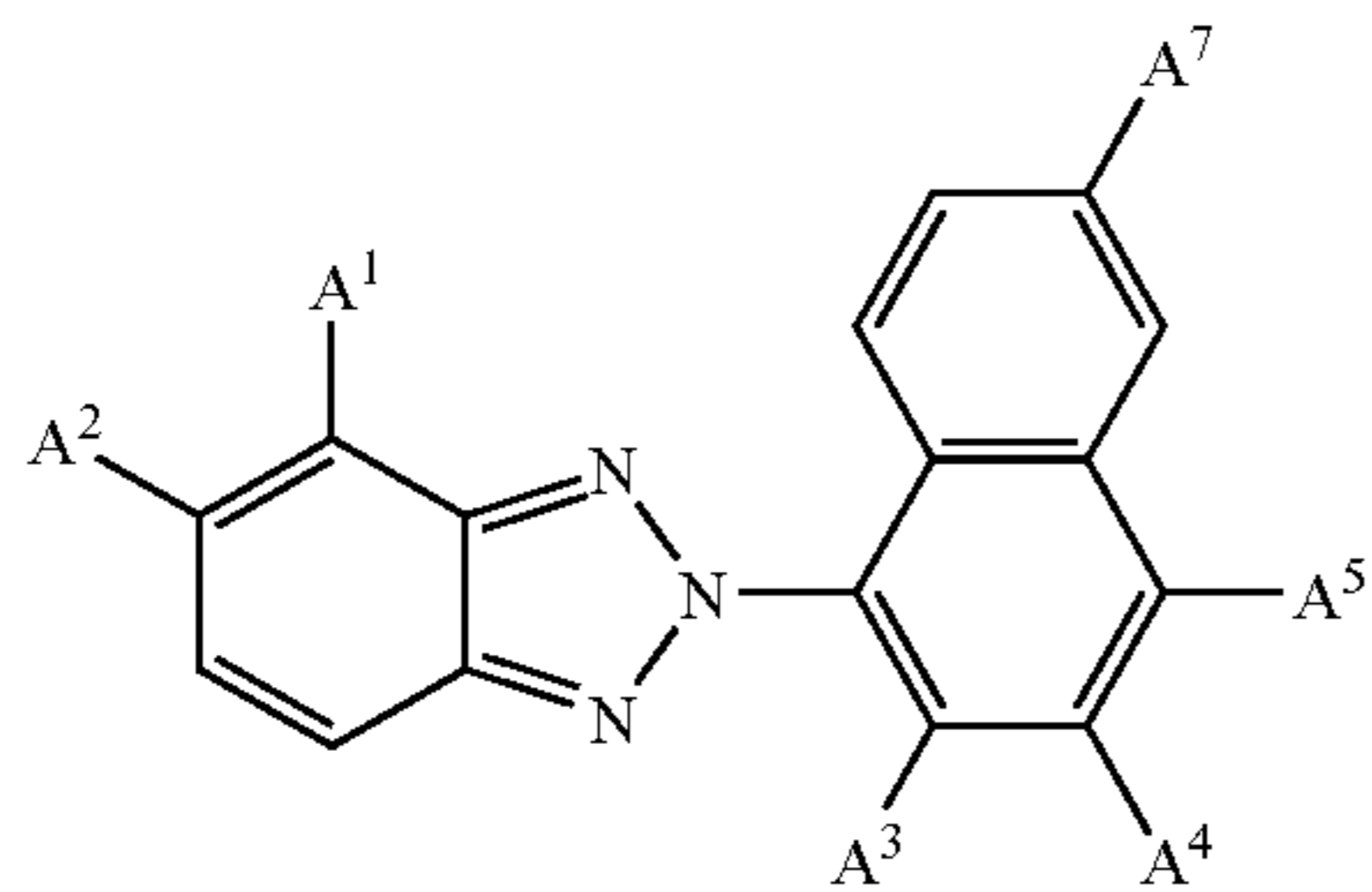
Monomer 3:
