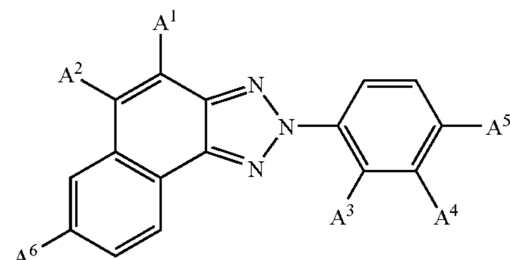
Monomer 1:
