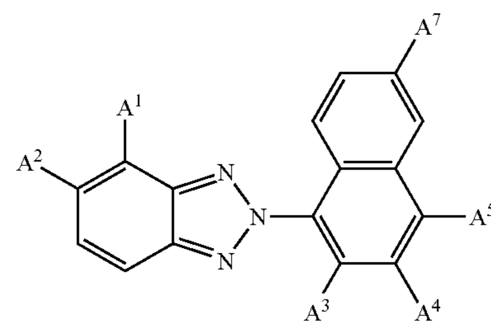
Monomer 1:
