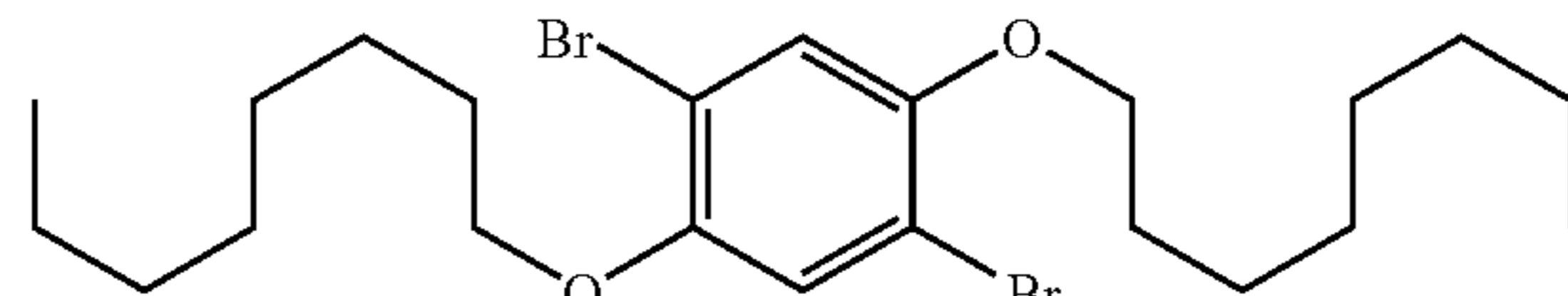
monomer 6
