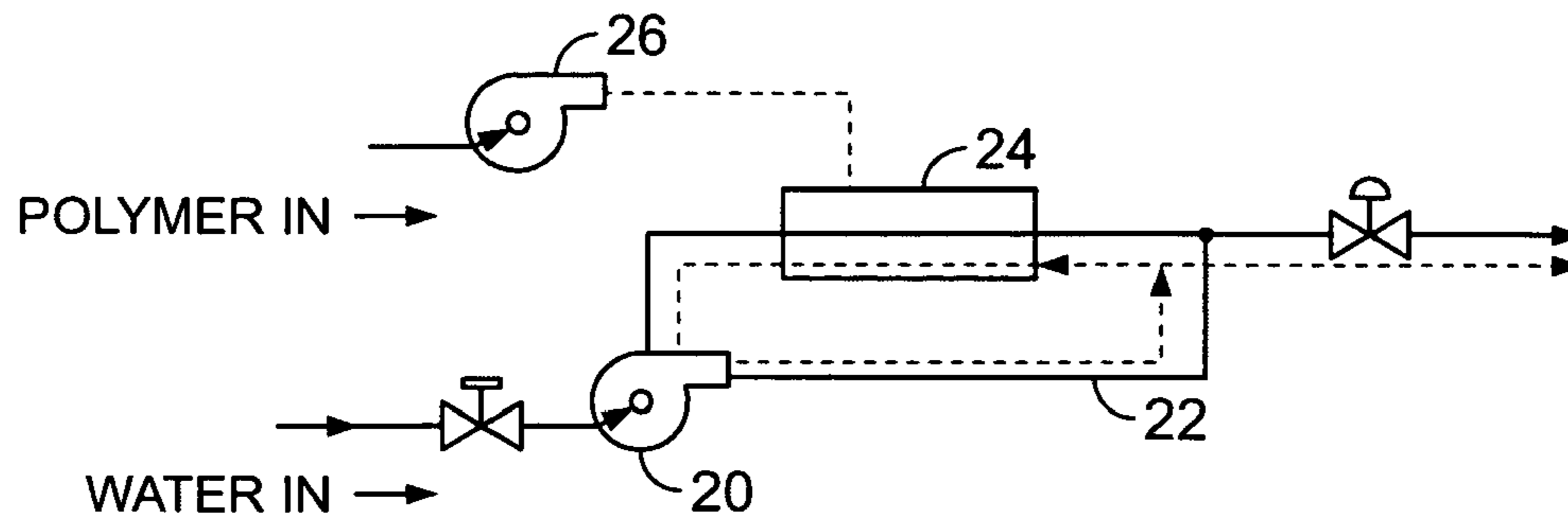
FIG. 1 (Prior Art)
