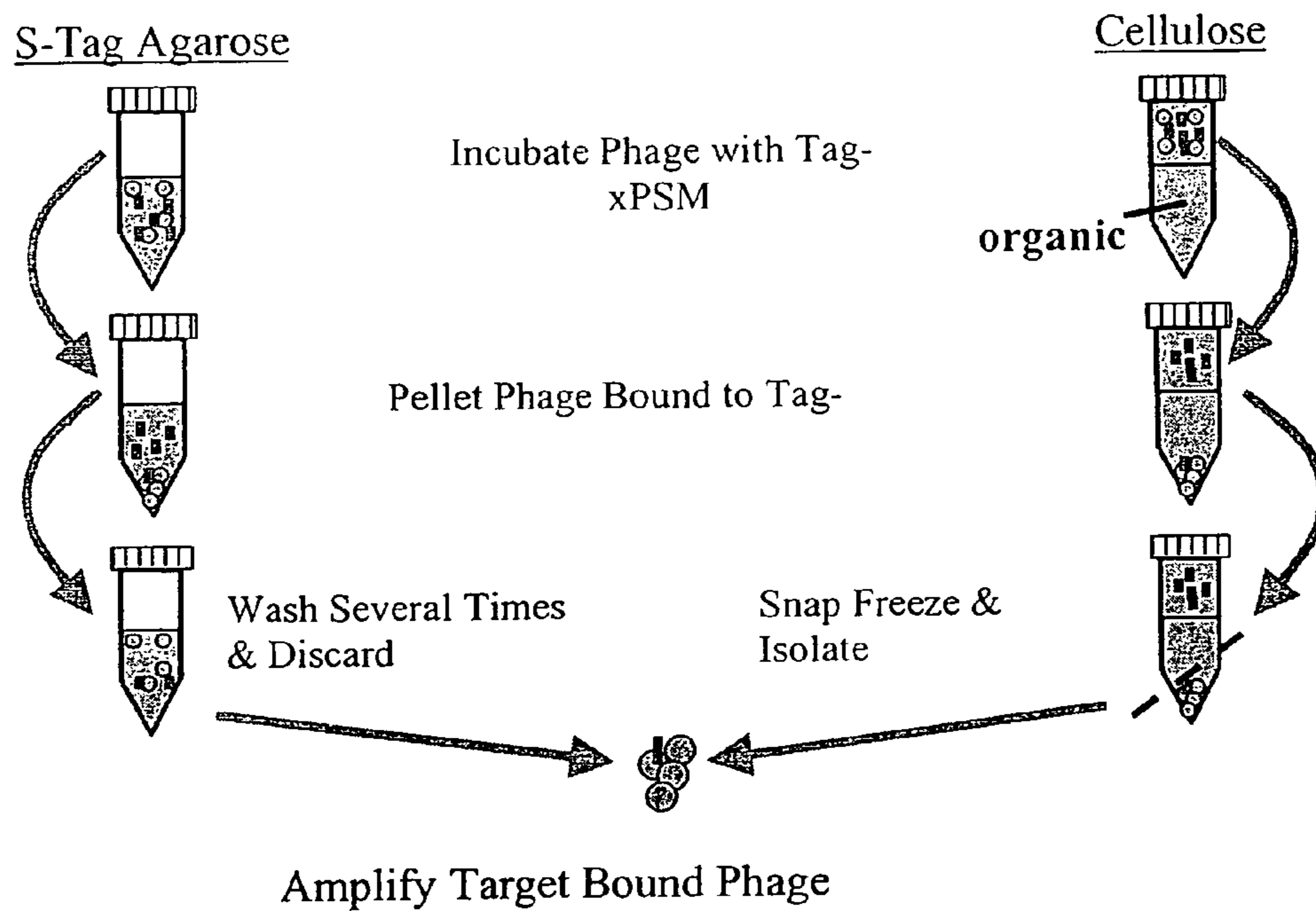
Figure 2: Schematic of Tag-xPSM Phage Display
