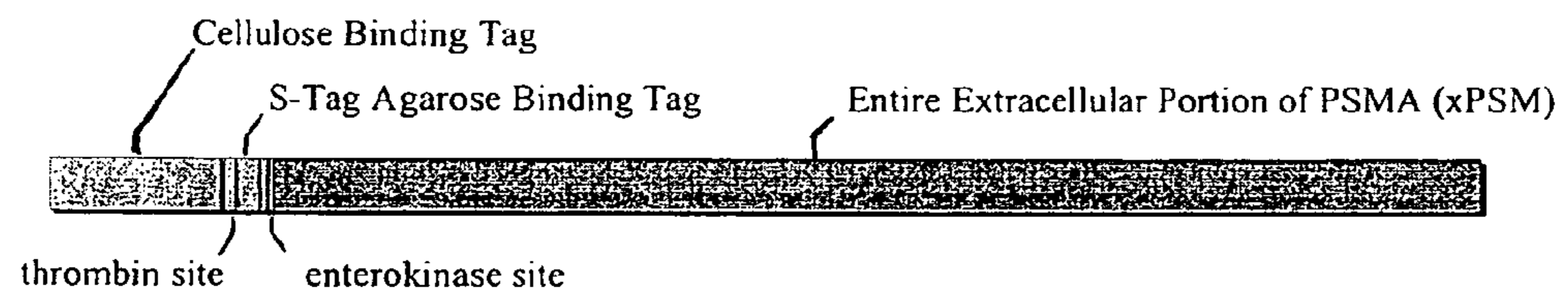
Figure 1. Target Protein: Tag-xPSM
