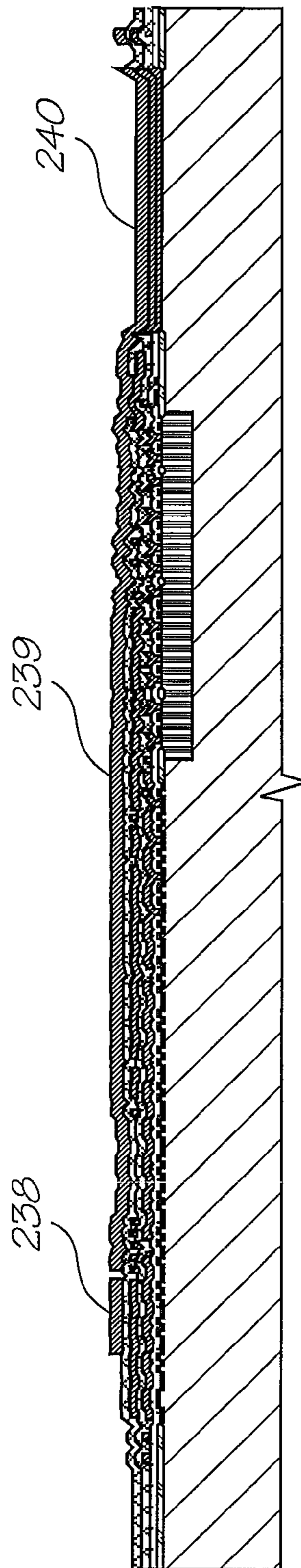
Deposit metal 3
