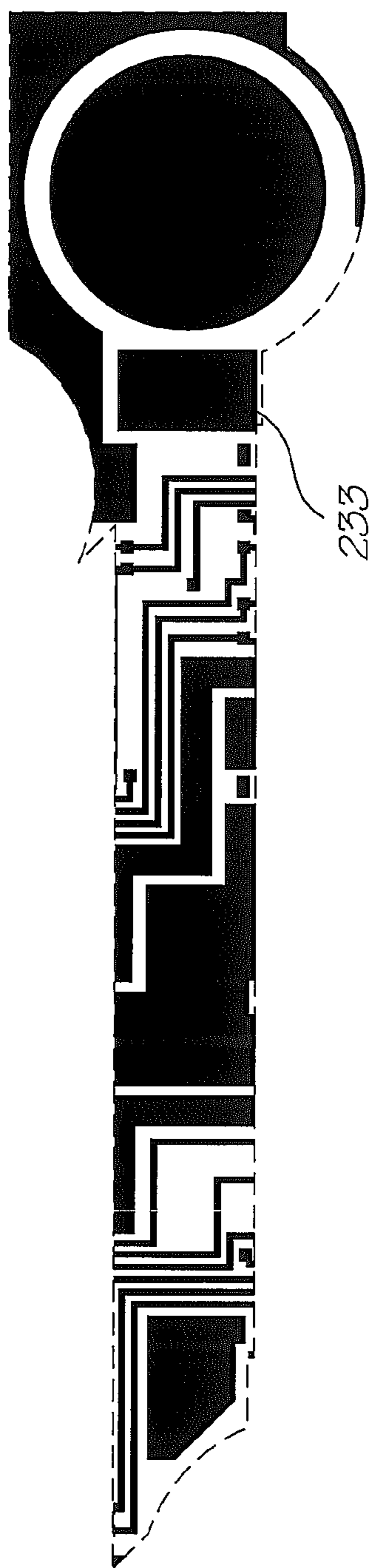
Metal 2 mask
