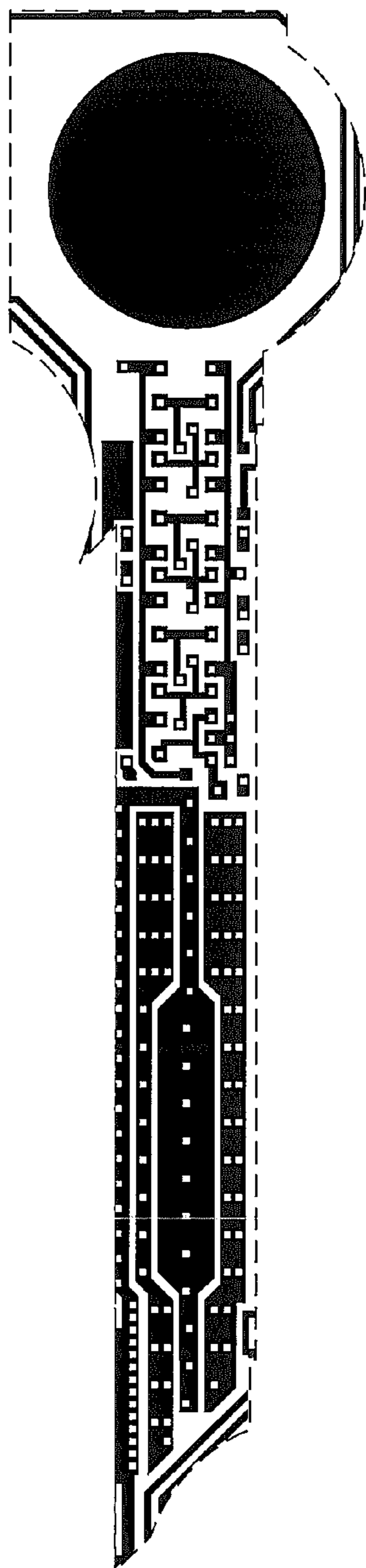
Metal 1 mask
