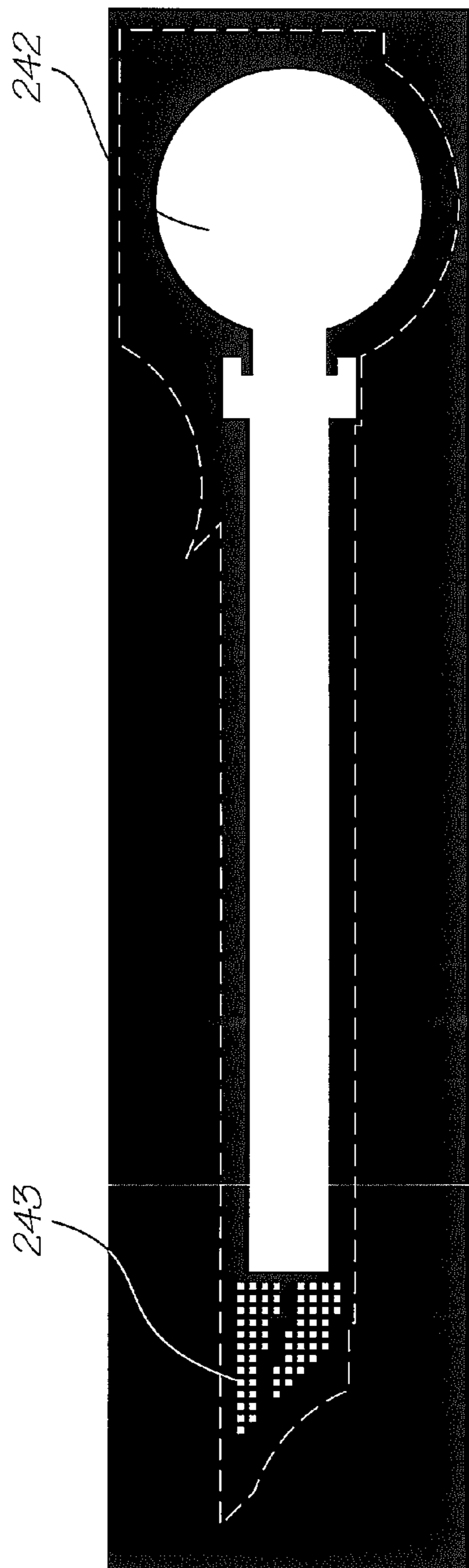
Via 3 / Passivation mask
