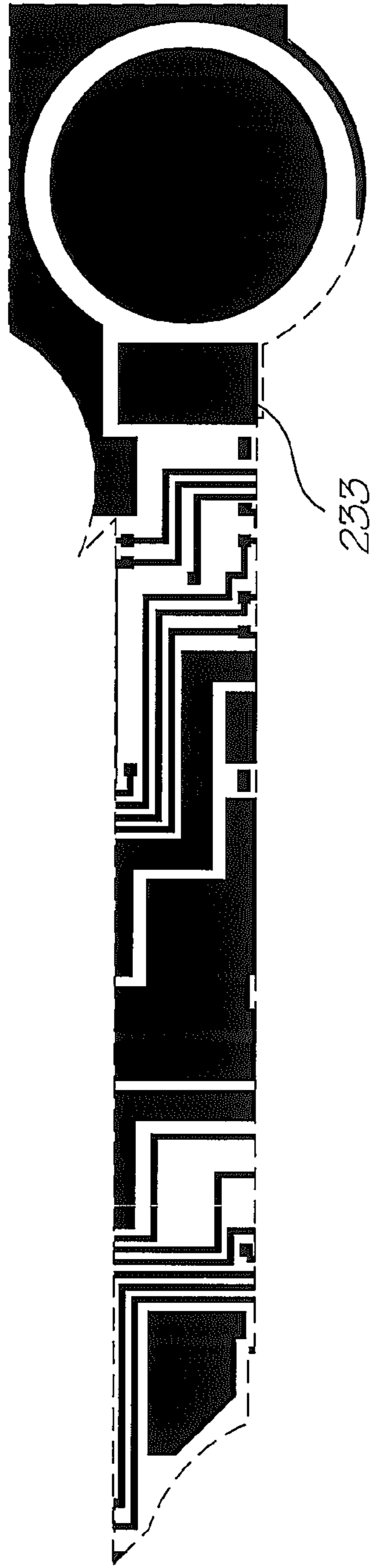
Metal 2 mask
