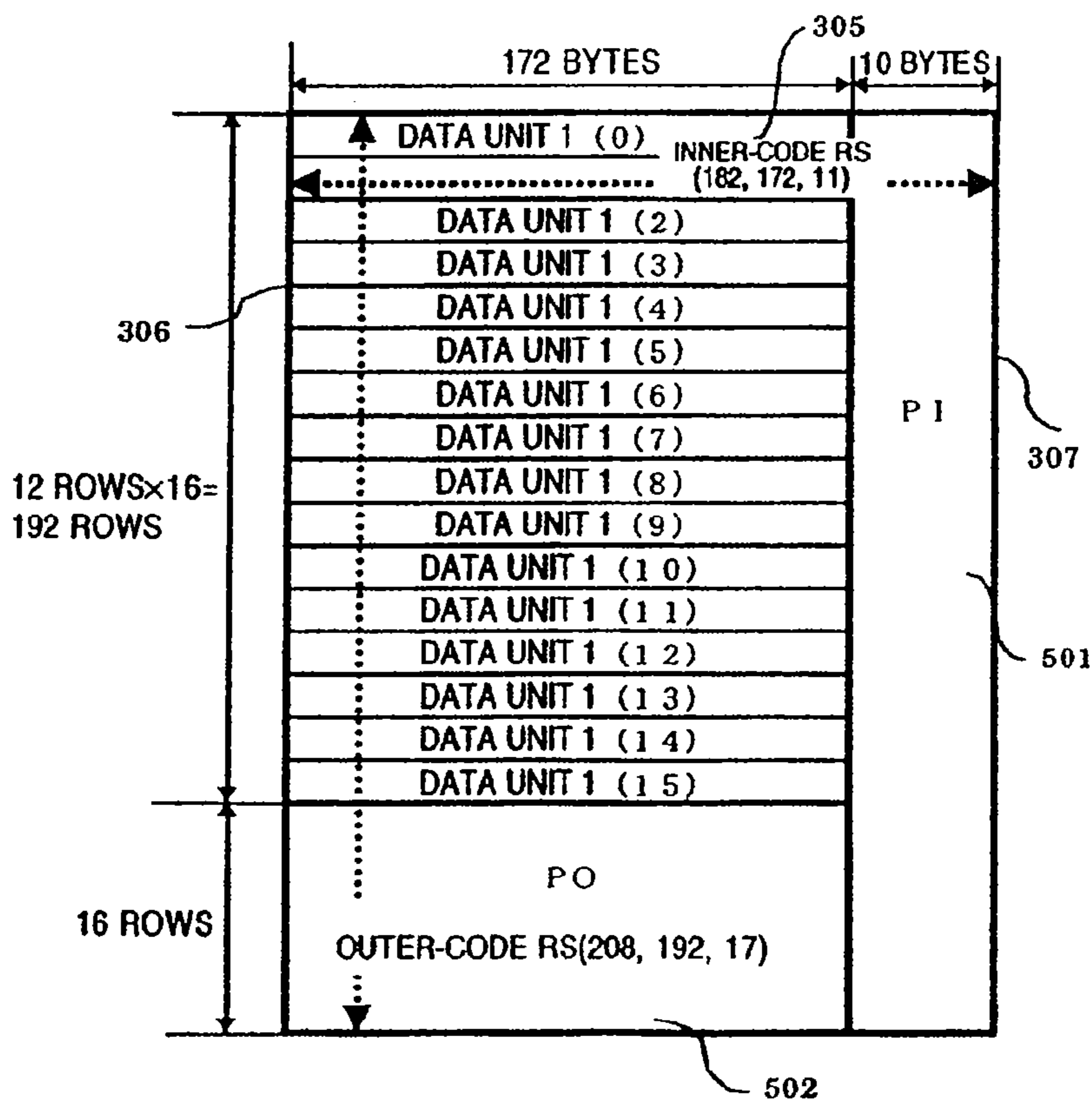
FIG. 6 (Prior Art)
