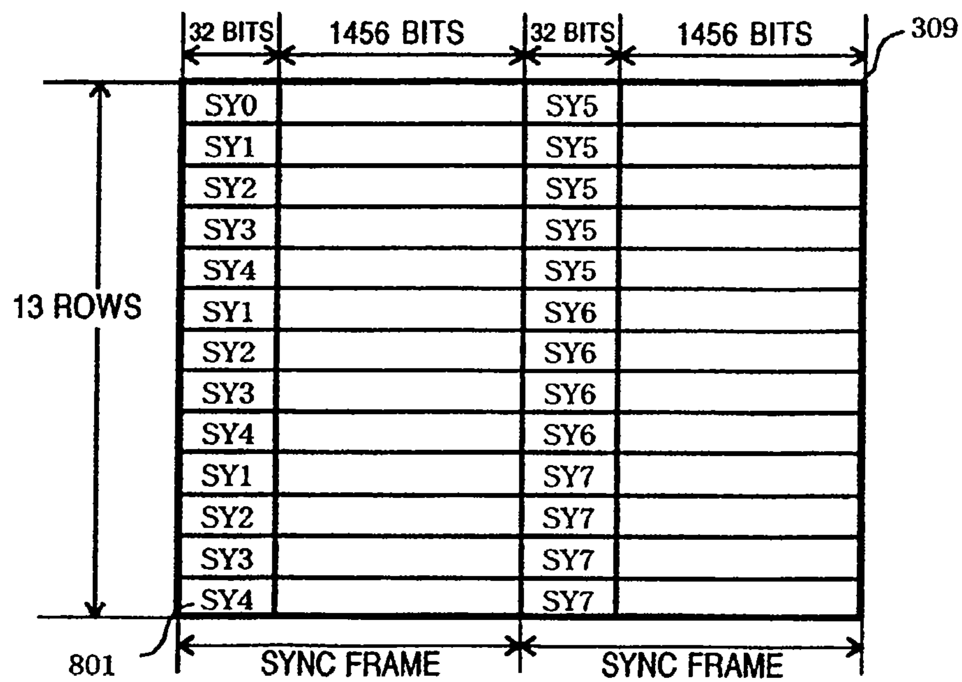
FIG. 8 (Prior Art)
