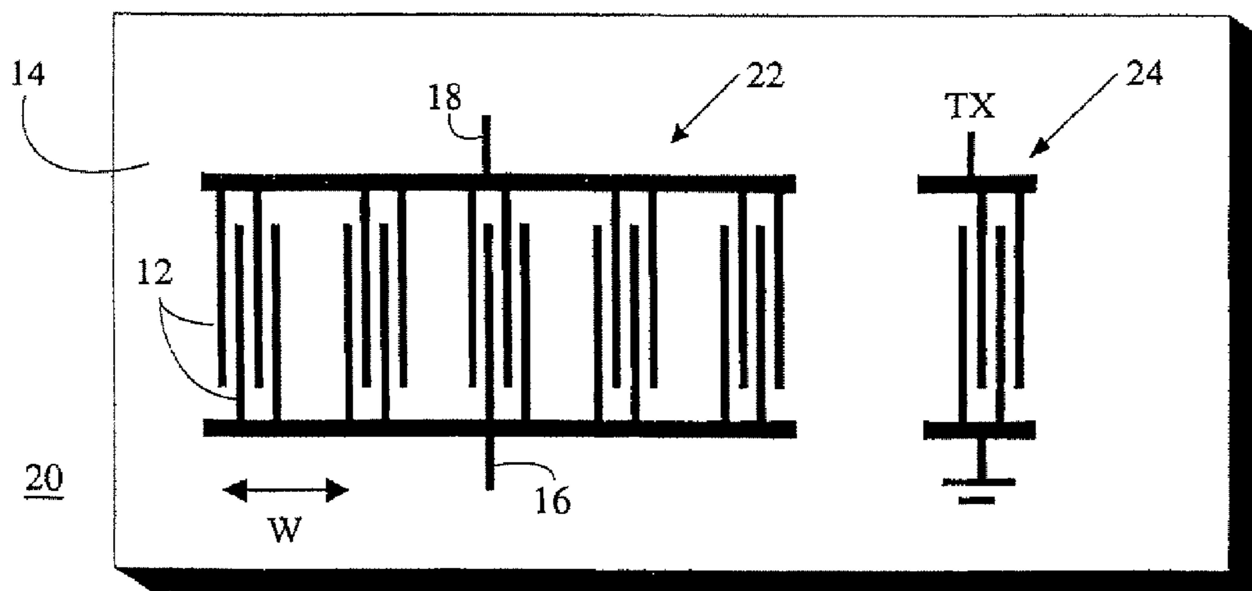
FIG. 2 - PRIOR ART
