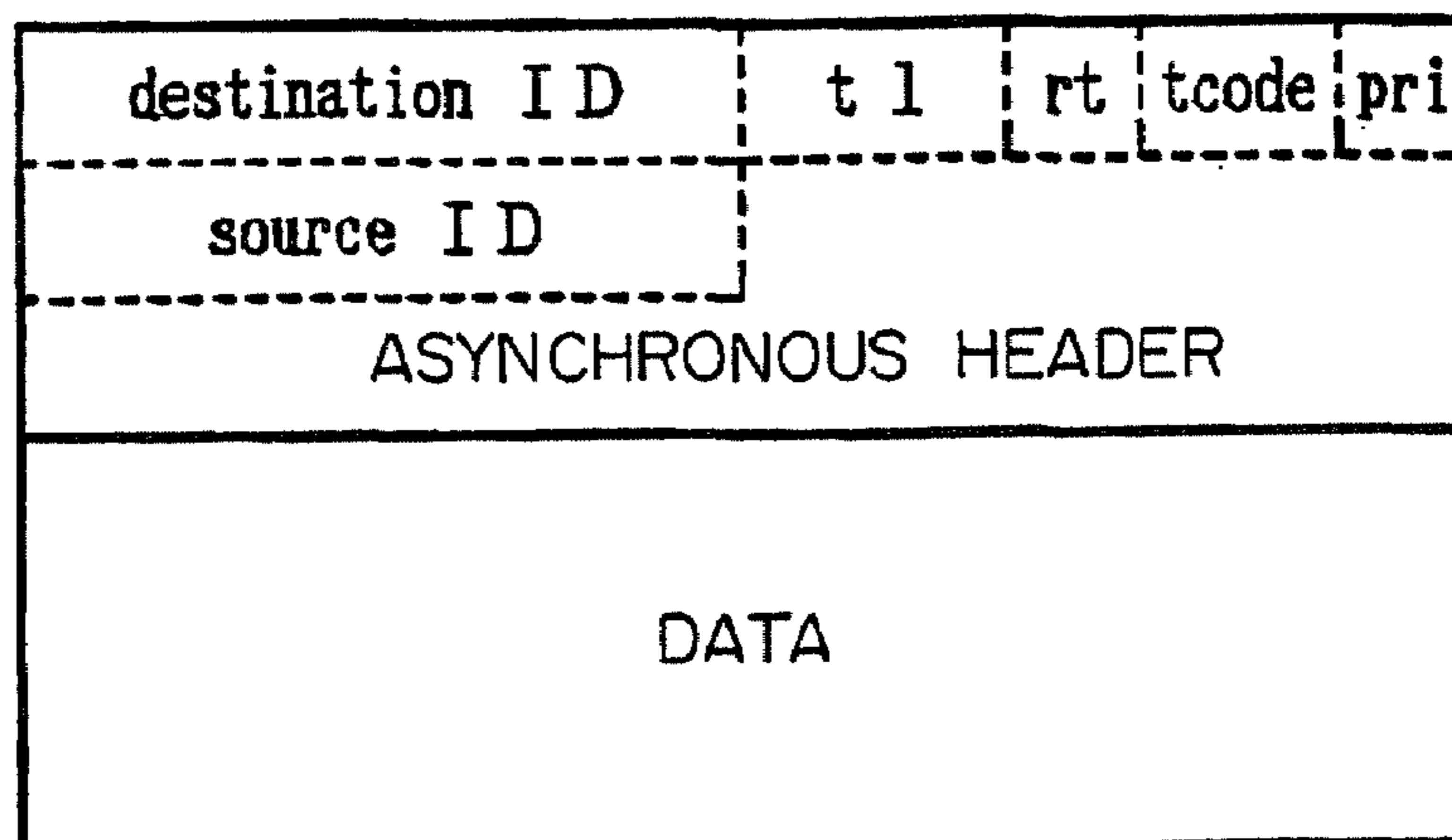
FIG. 6C PRIOR ART
