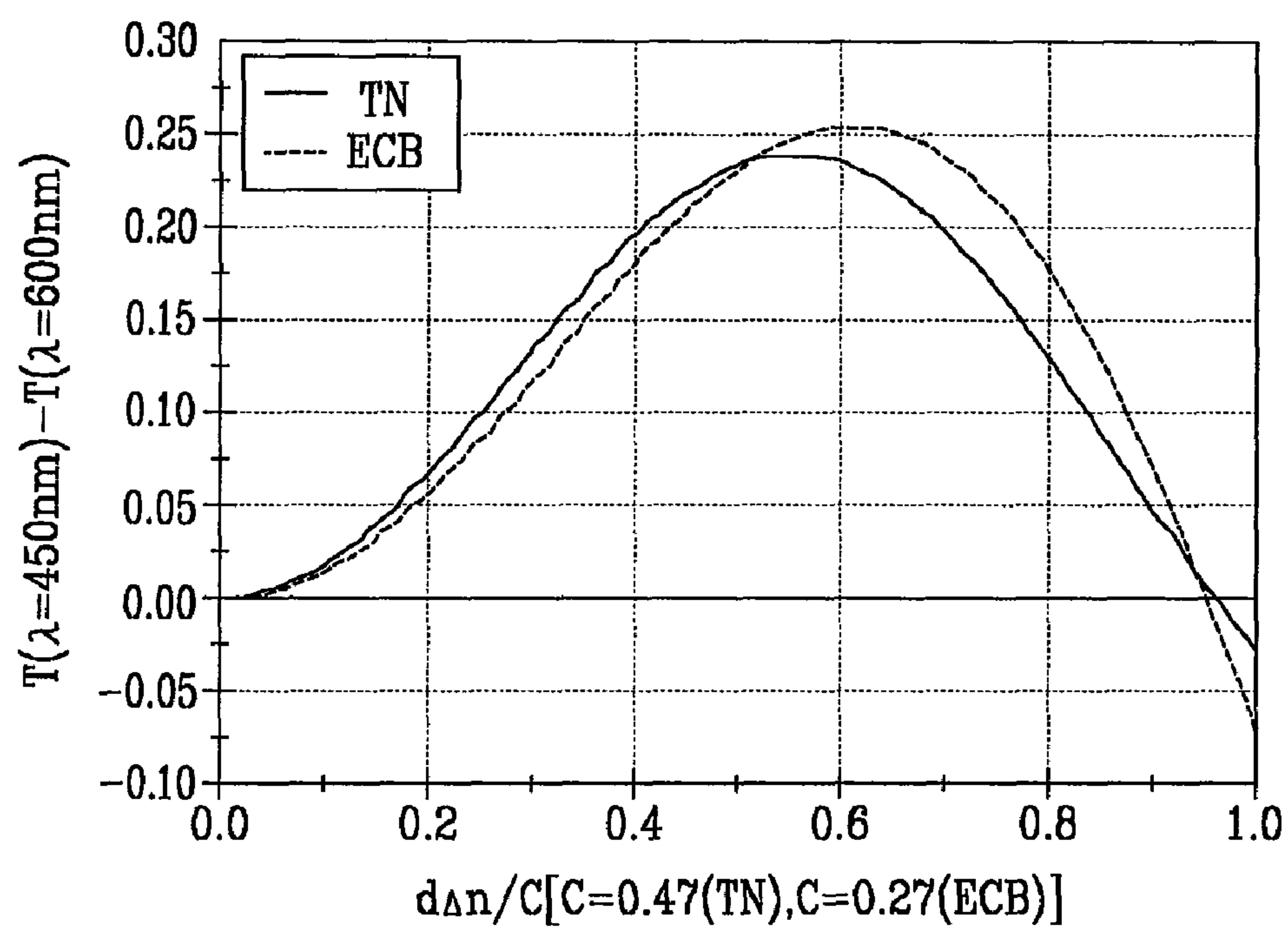
FIG.2(Prior Art)
