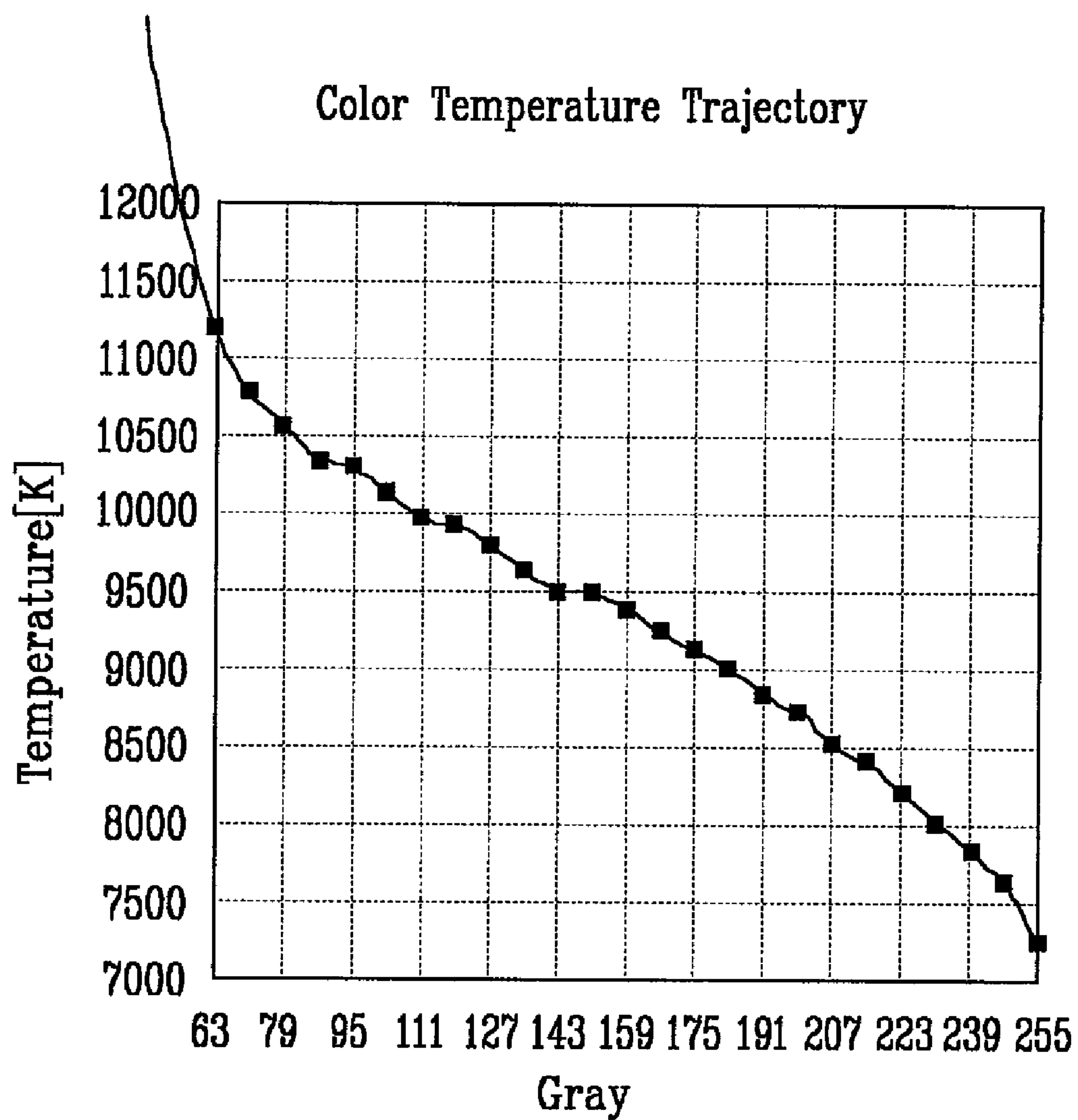
FIG.5(Prior Art)
