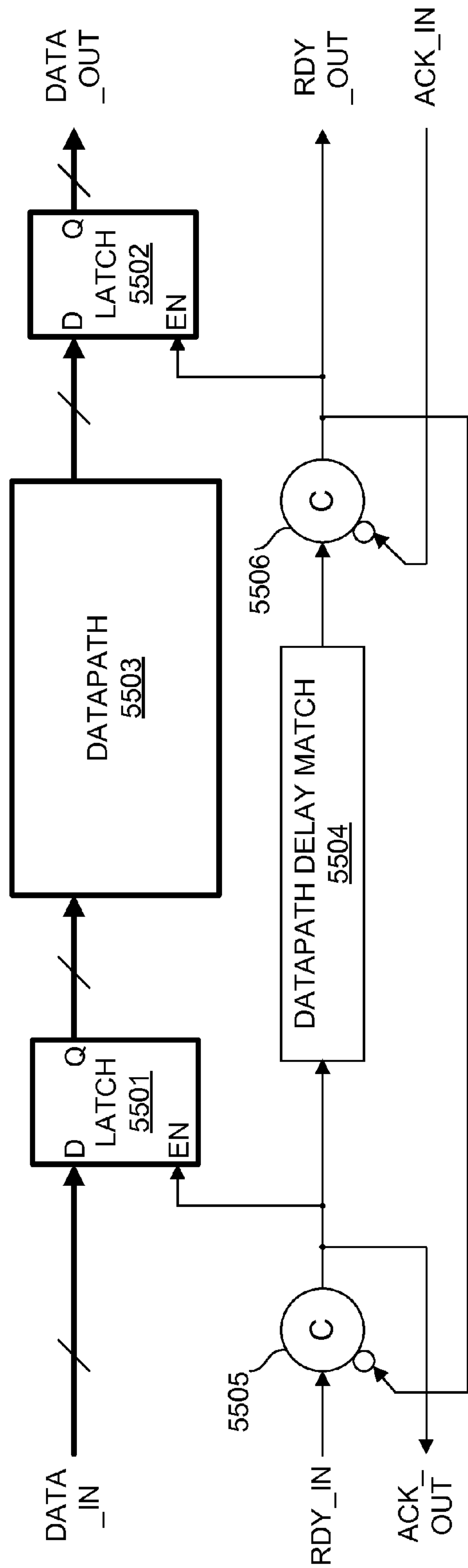
FIG. 55 (4-phase)
