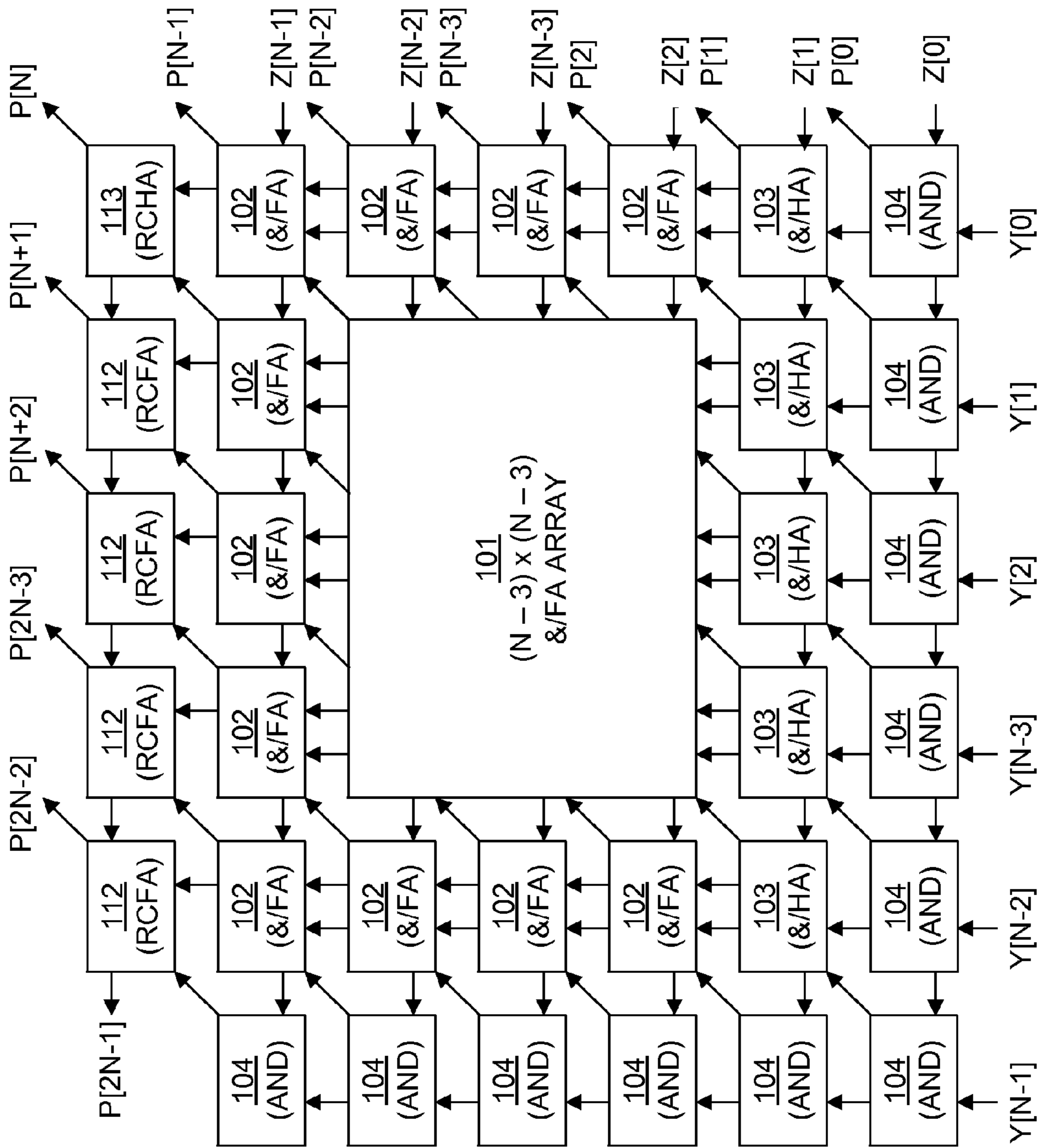
FIG. 1 (Prior Art)
