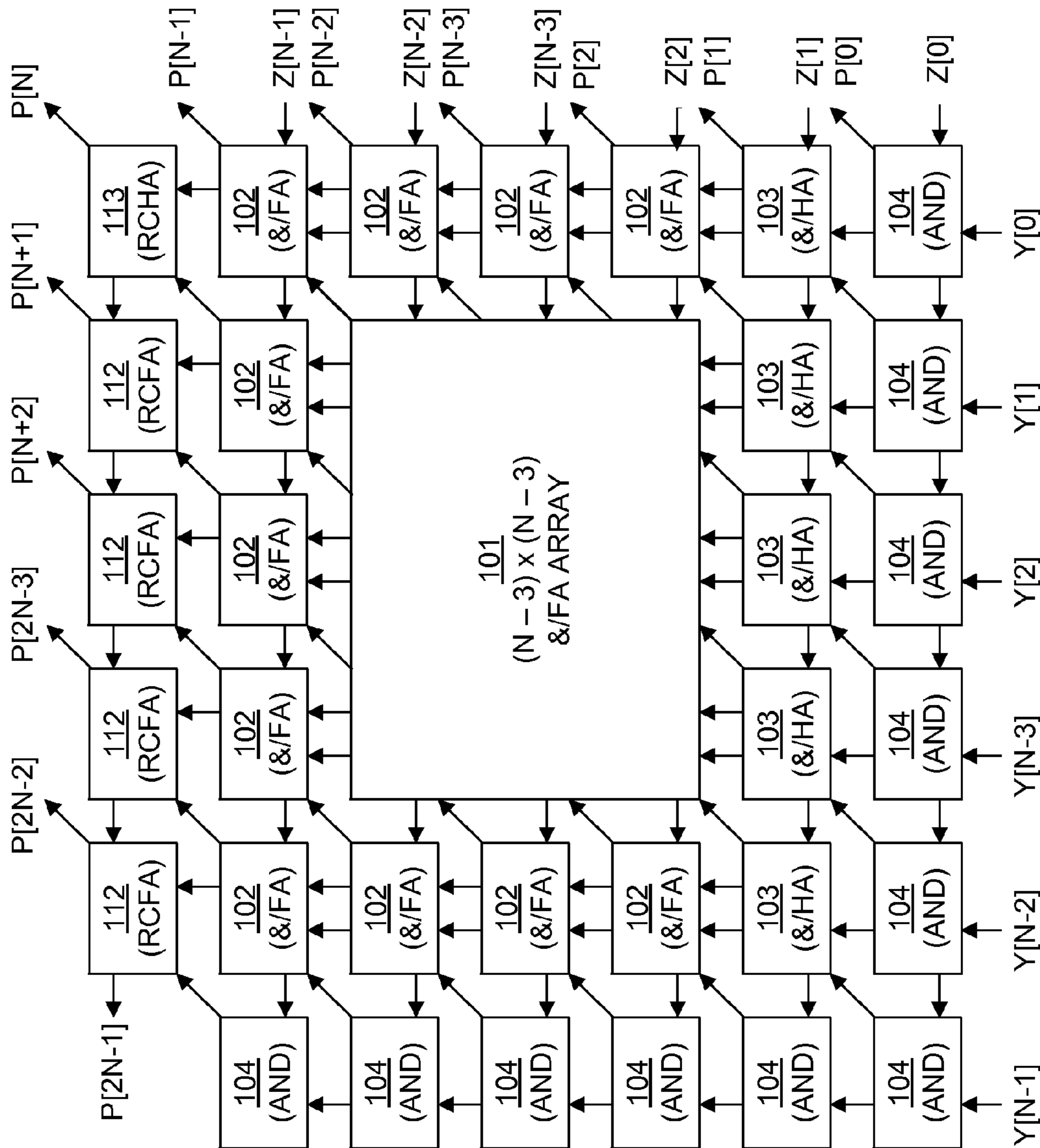
FIG. 1 (Prior Art)
