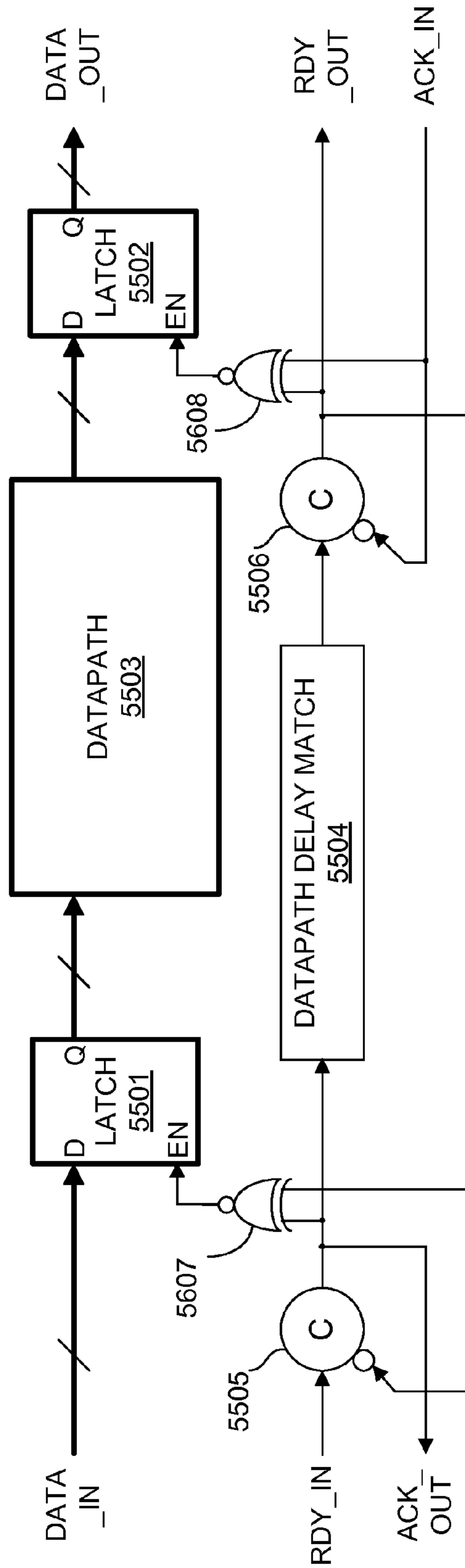
FIG. 56 (2-phase)
