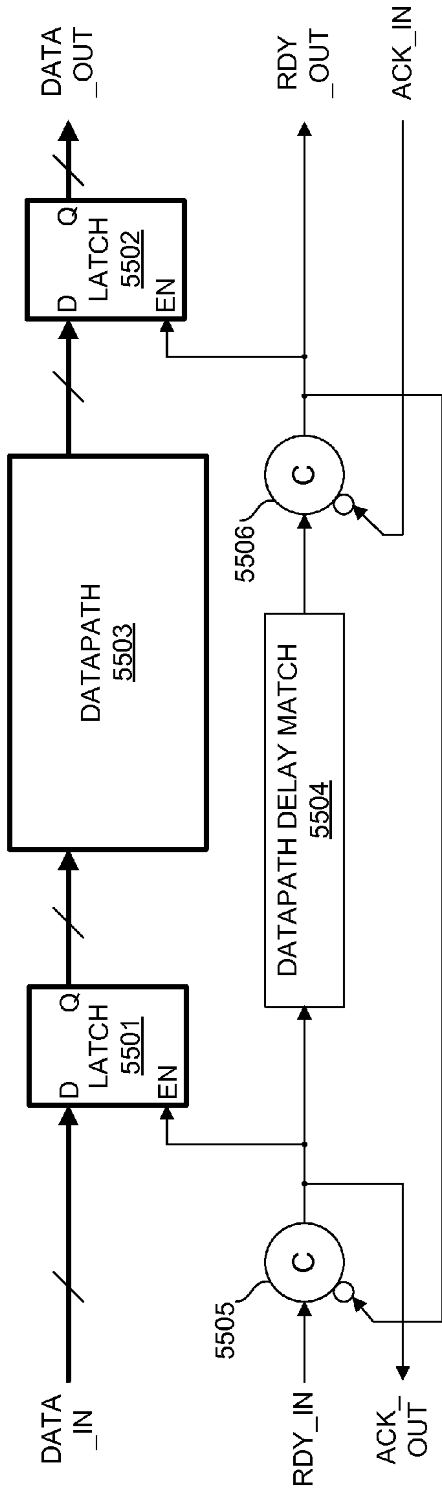
FIG. 55 (4-phase)
