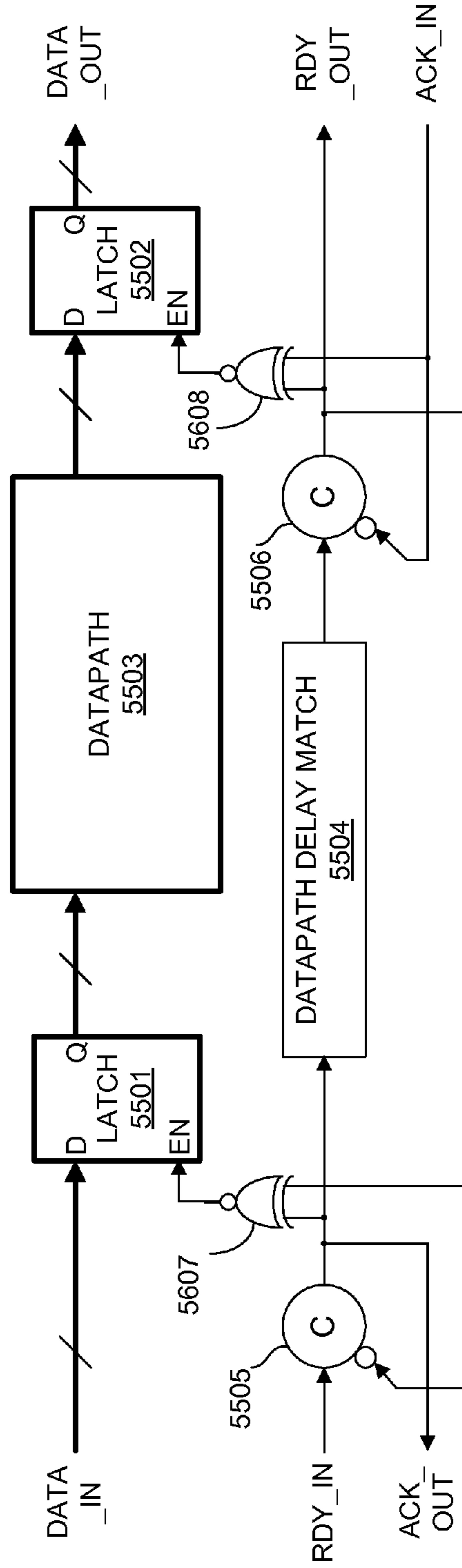
FIG. 56 (2-phase)
