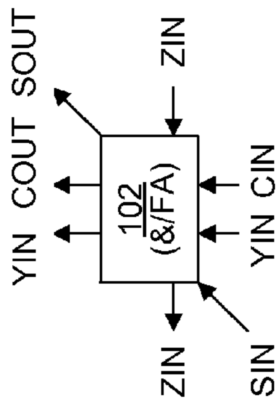
FIG. 2 (Prior Art)
