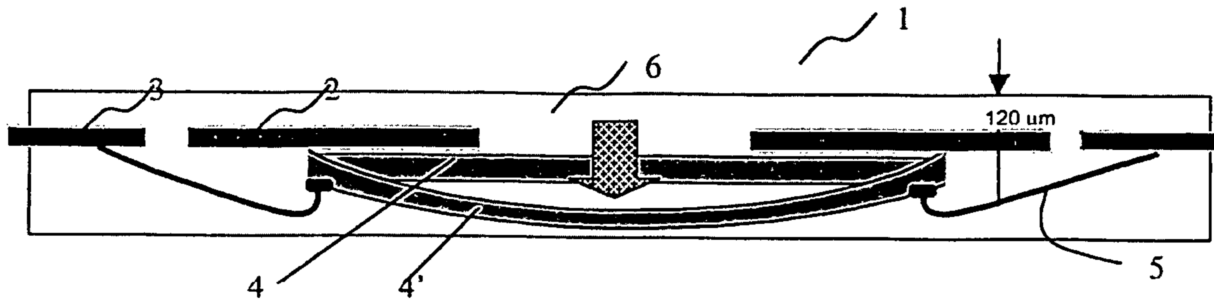
FIG 1 (Prior art)
