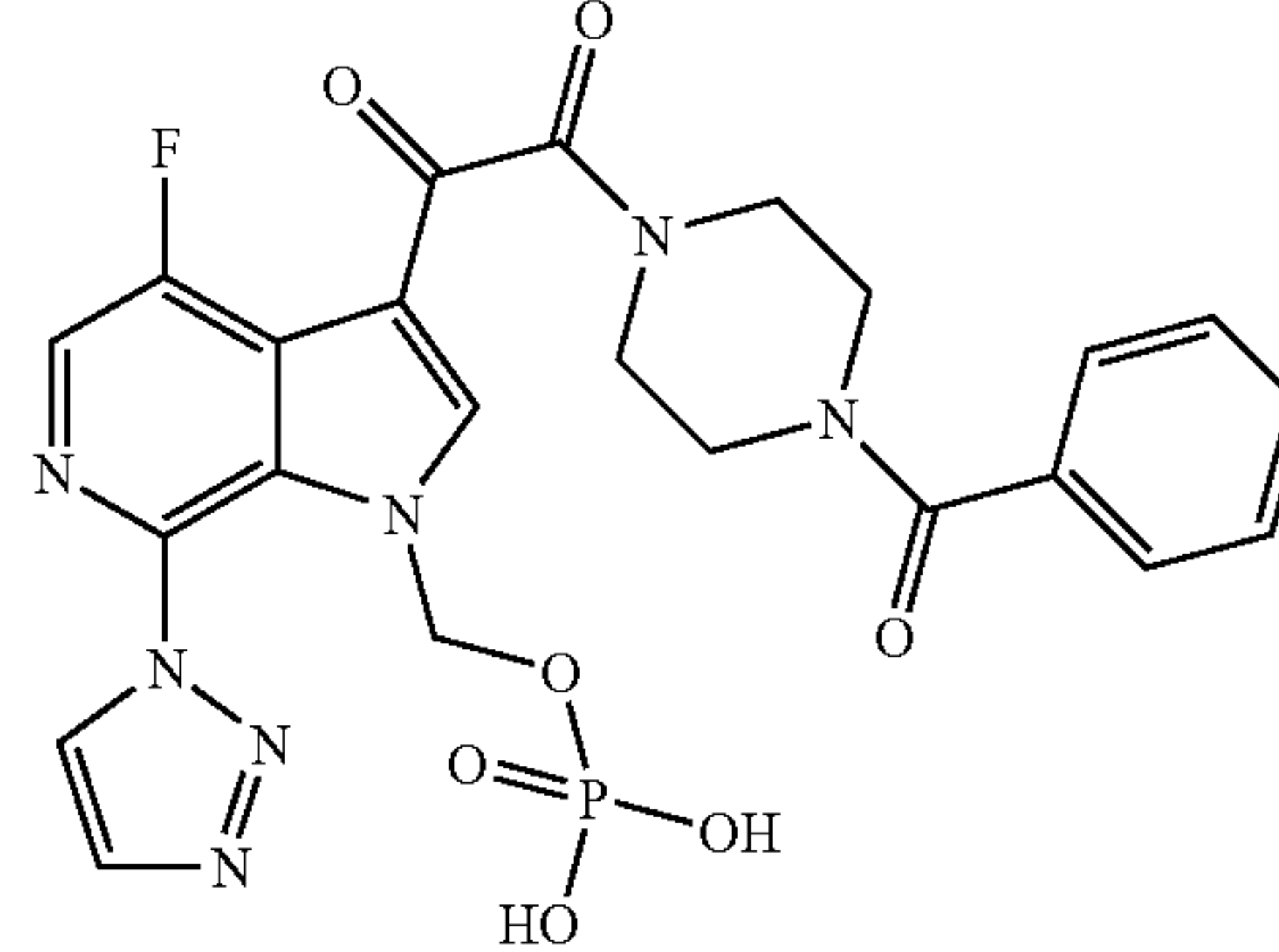
Ibc Mol. Wt. = 557.43
