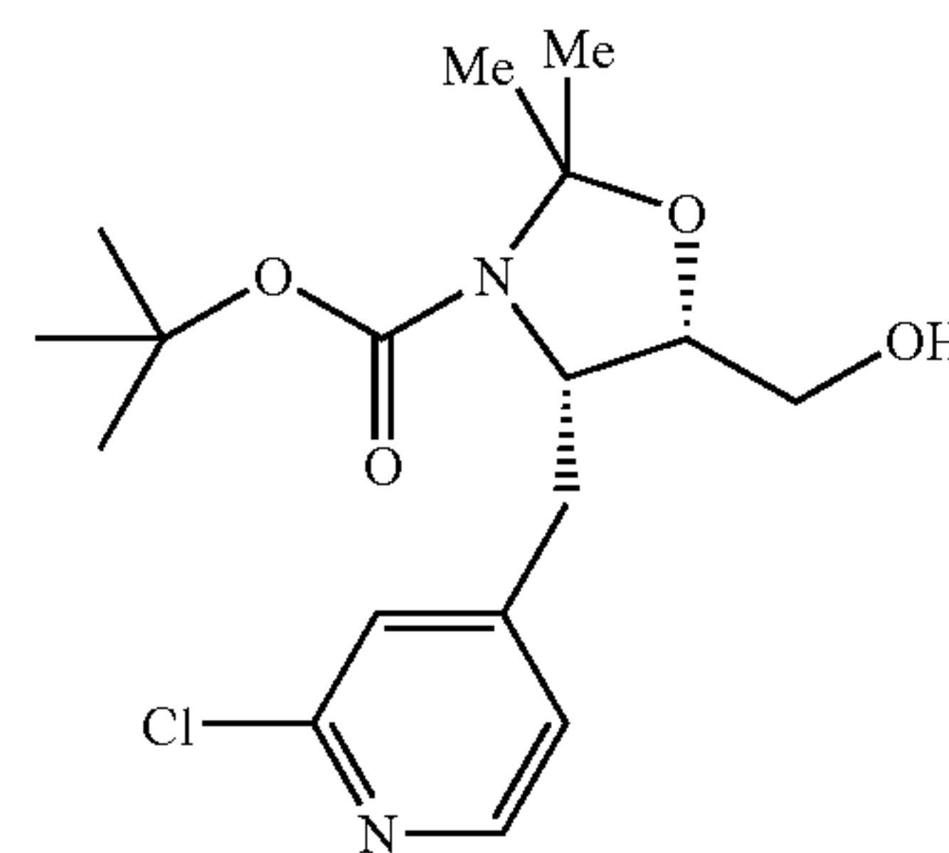
(4S,5S)-tert-butyl 4-((2-chloropyridin-4-yl)methyl)-5-(hydroxymethyl)-2,2-dimethyloxazolidine-3-carboxylate
