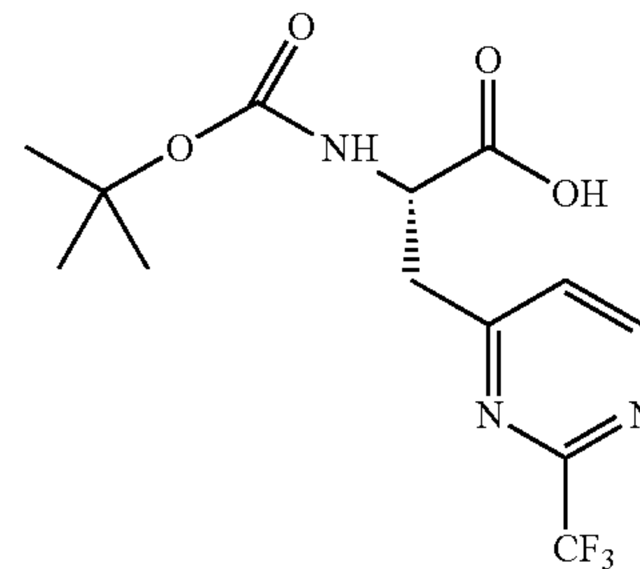
(S)-methyl 2-(tert-butoxycarbonyl)-3-(2-(trifluoromethyl)pyrimidin-4-yl)propanoate
