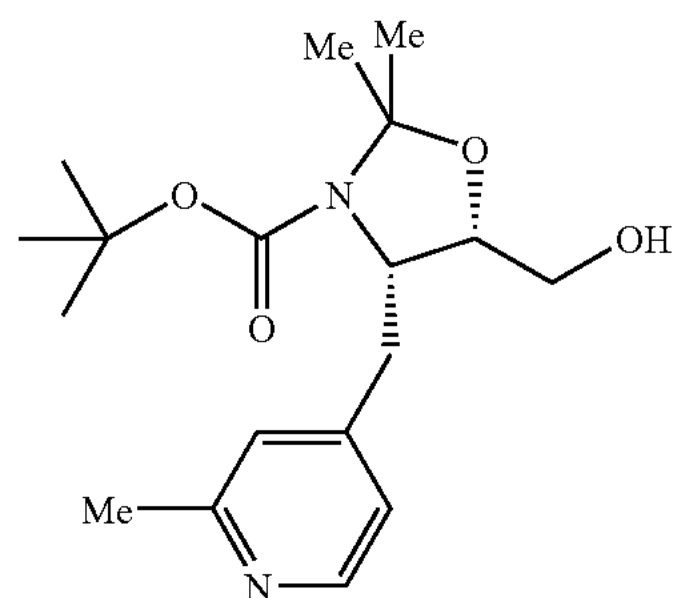
(4S,5S)-tert-butyl 5-(hydroxymethyl)-2,2-dimethyl-4-((2-methylpyridin-4-yl)methyl)oxazolidine-3-carboxylate
