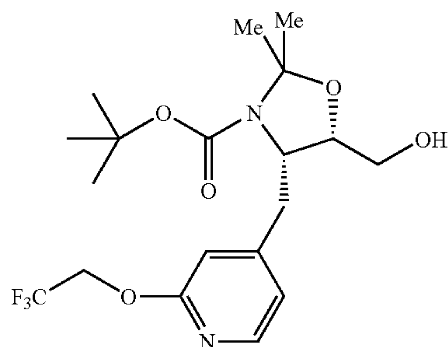
(4S,5S)-tert-butyl 5-((2-(2,2,2-trifluoroethoxy)pyridin-4-yl)methyl)-2,2-dimethyl-4-oxazolidine-3-carboxylate
