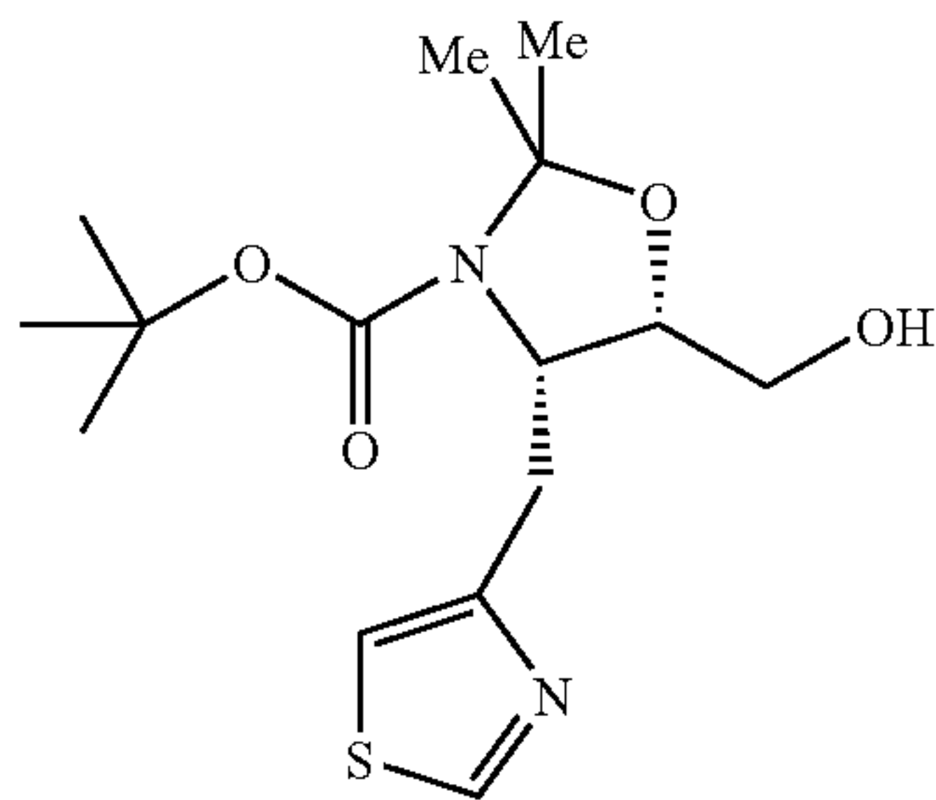
(4S,5S)-tert-butyl 5-(hydroxymethyl)-2,2-dimethyl-4-(thiazol-4-ylmethyl)oxazolidine-3-carboxylate
