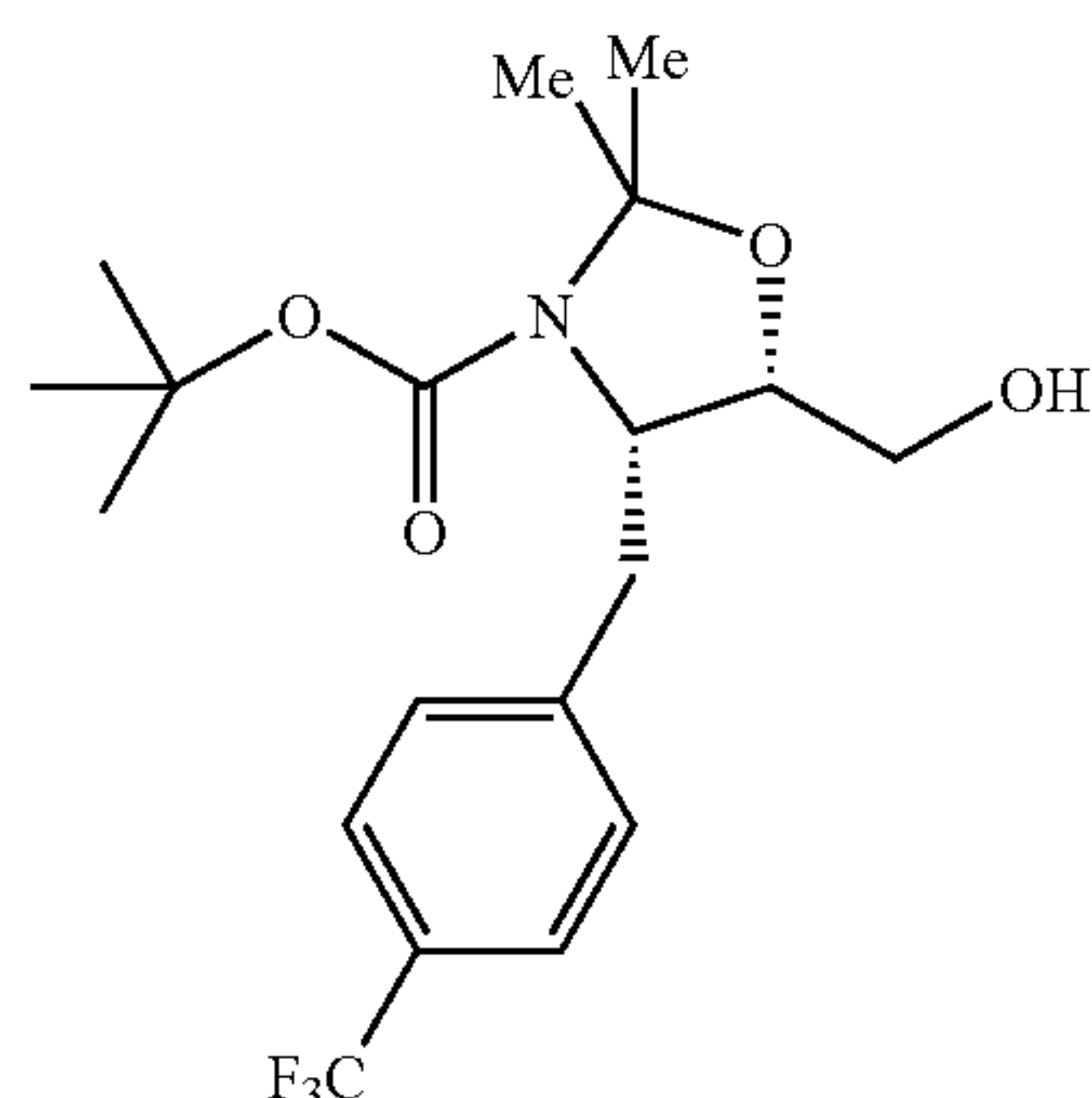
(4S,5S)-tert-butyl 4-(4-(trifluoromethyl)benzyl)-5-(hydroxymethyl)-2,2-dimethyloxazolidine-3-carboxylate
