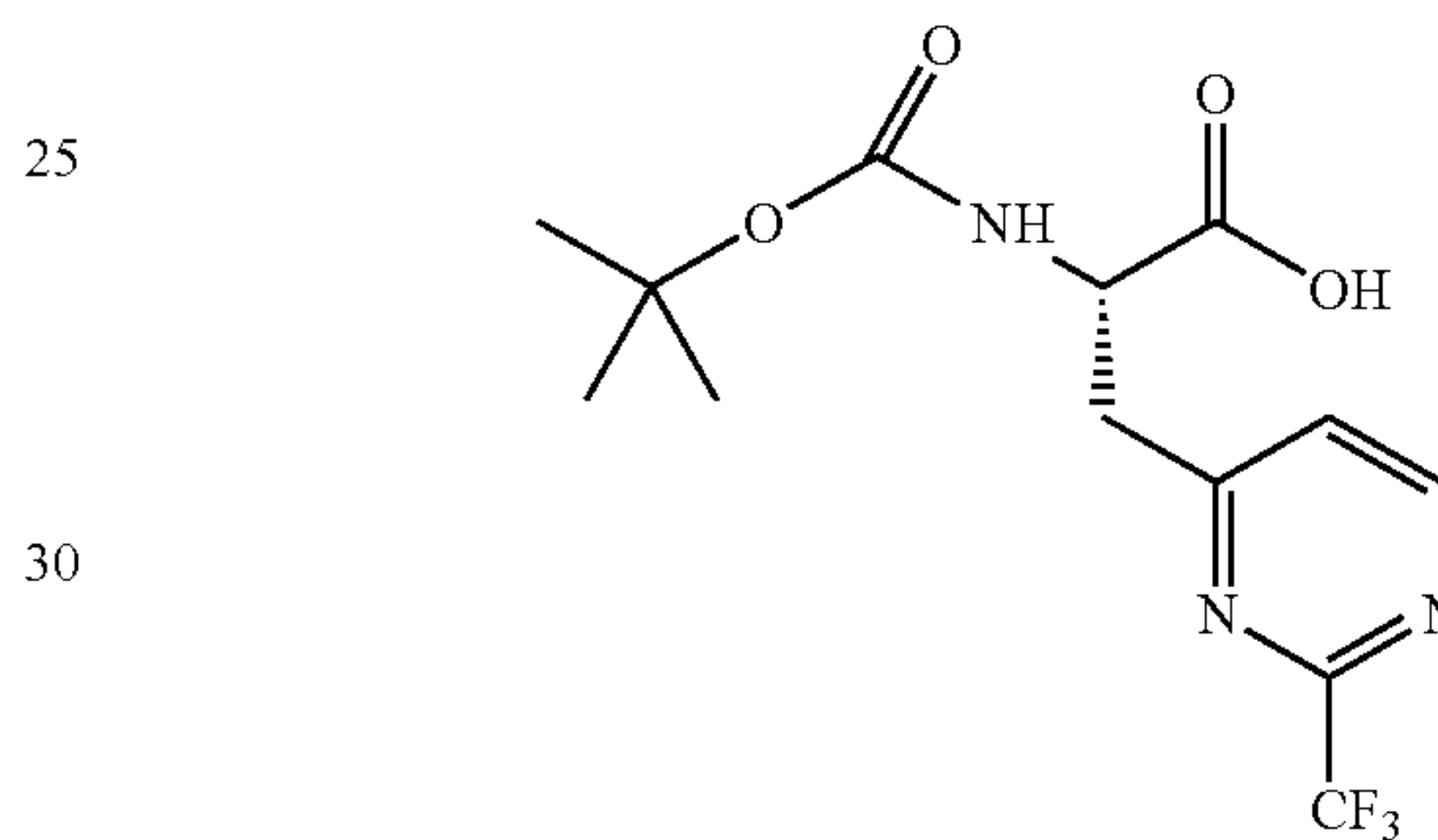
(S)-methyl 2-(tert-butoxycarbonyl)-3-(2-(trifluoromethyl)pyrimidin-4-yl)propanoate
