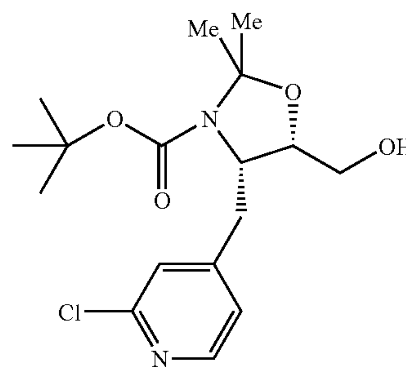
(4S,5S)-tert-butyl 4-((2-chloropyridin-4-yl)methyl)-5-(hydroxymethyl)-2,2-dimethyloxazolidine-3-carboxylate
