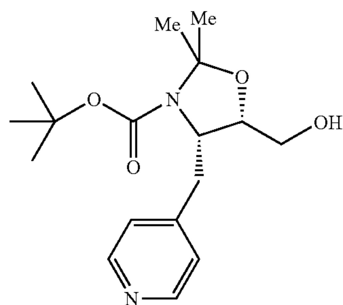
(4S,5S)-tert-butyl 5-(hydroxymethyl)-2,2-dimethyl-4-(pyridin-4-ylmethyl)oxazolidine-3-carboxylate
