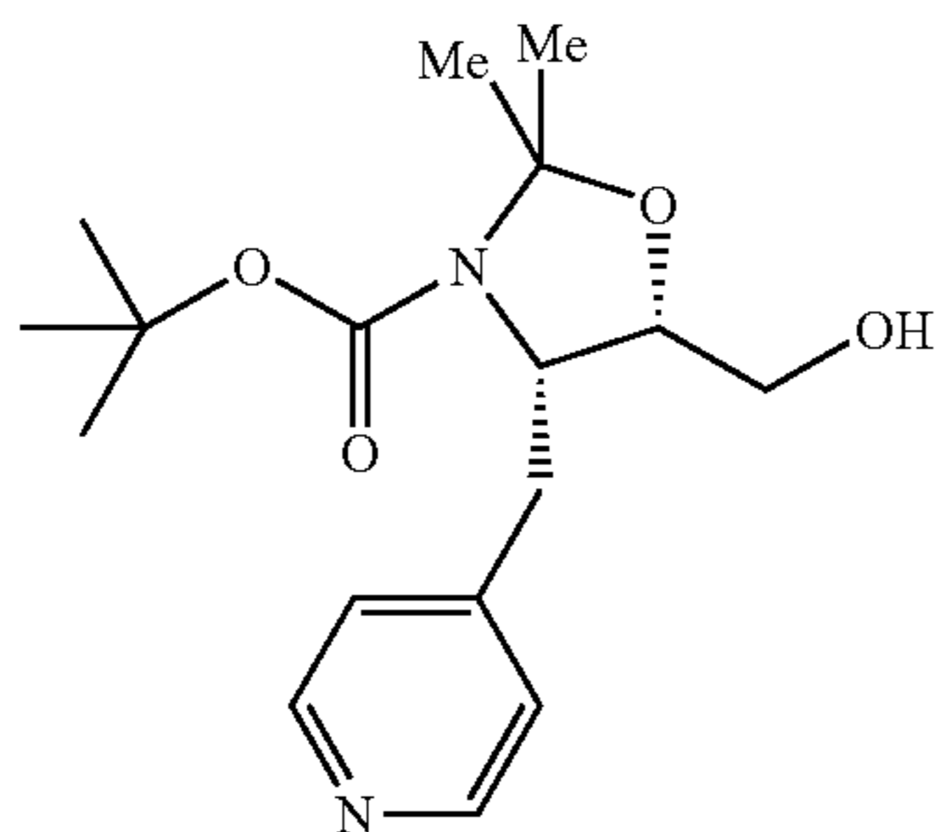
(4S,5S)-tert-butyl 5-(hydroxymethyl)-2,2-dimethyl-4-(pyridin-4-ylmethyl)oxazolidine-3-carboxylate
