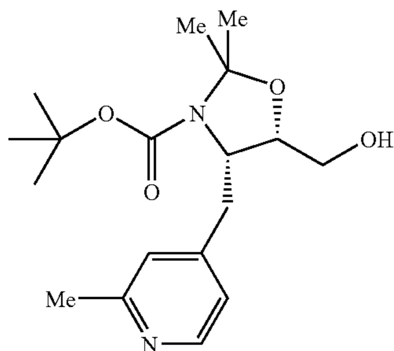
(4S,5S)-tert-butyl 5-(hydroxymethyl)-2,2-dimethyl-4-((2-methylpyridin-4-yl)methyl)oxazolidine-3-carboxylate
