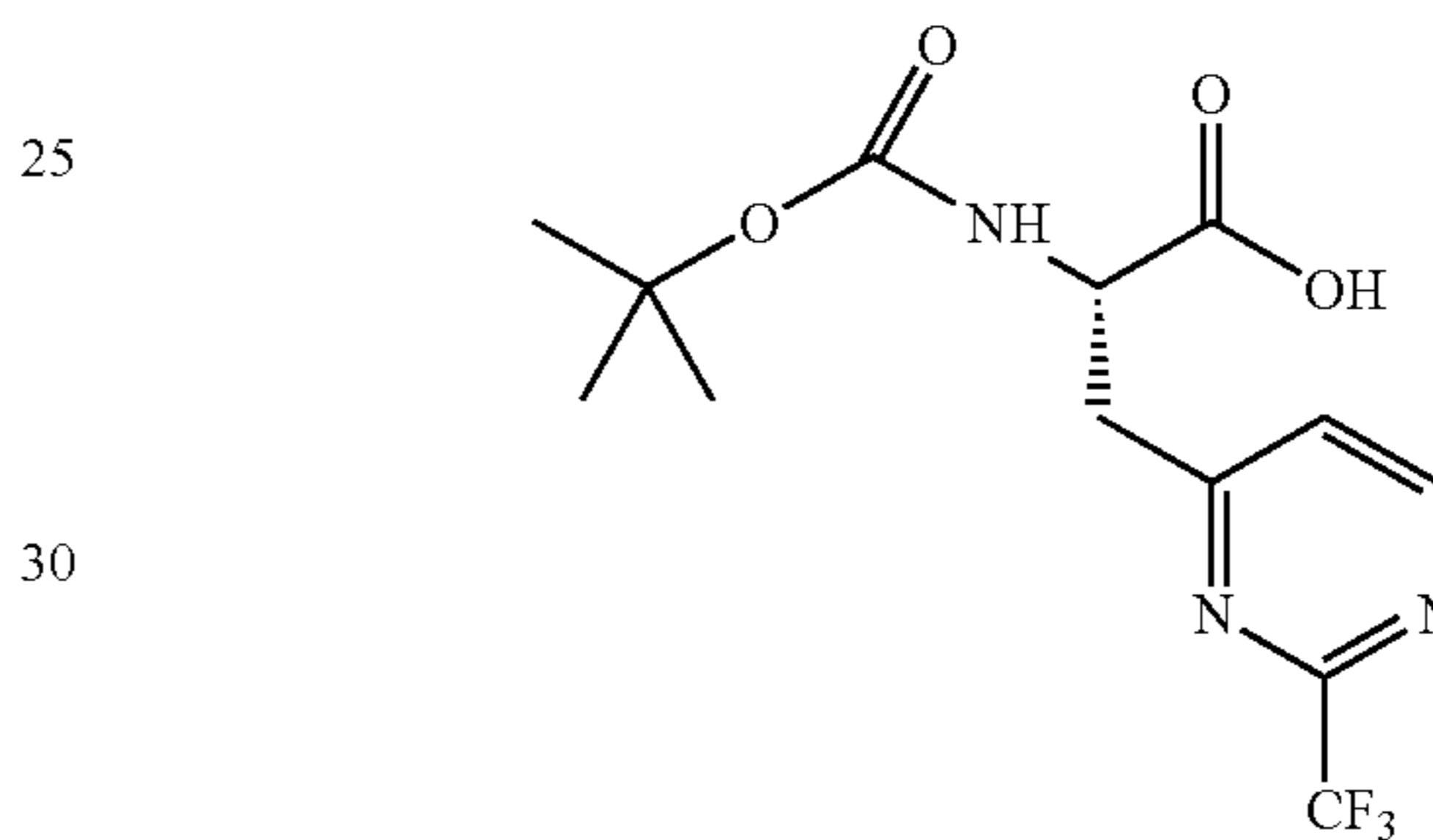
(S)-methyl 2-(tert-butoxycarbonyl)-3-(2-(trifluoromethyl)pyrimidin-4-yl)propanoate
