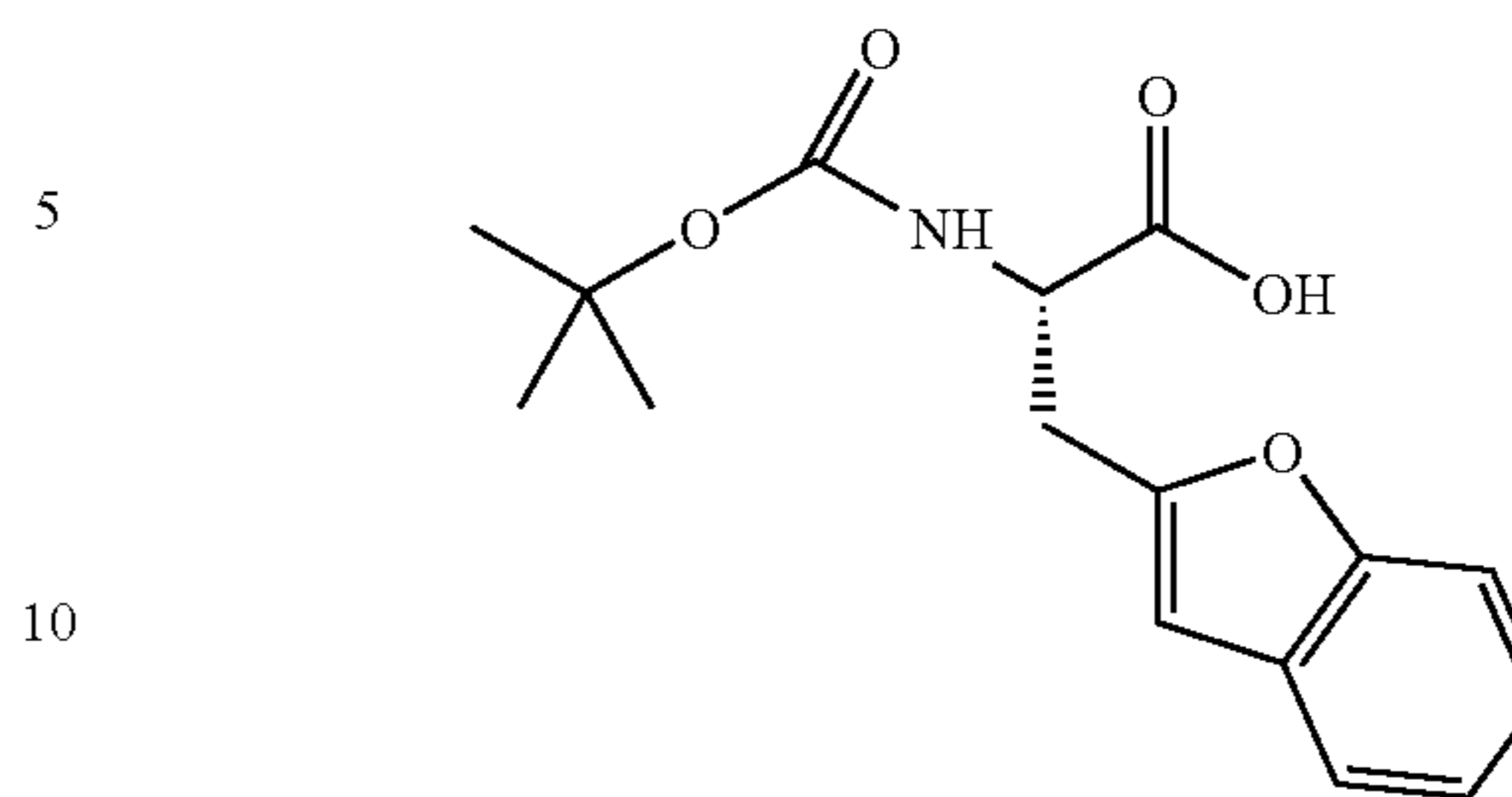
(S)-methyl 3-(benzofuran-2-yl)-2-(tert-butoxycarbonyl)propanoate
