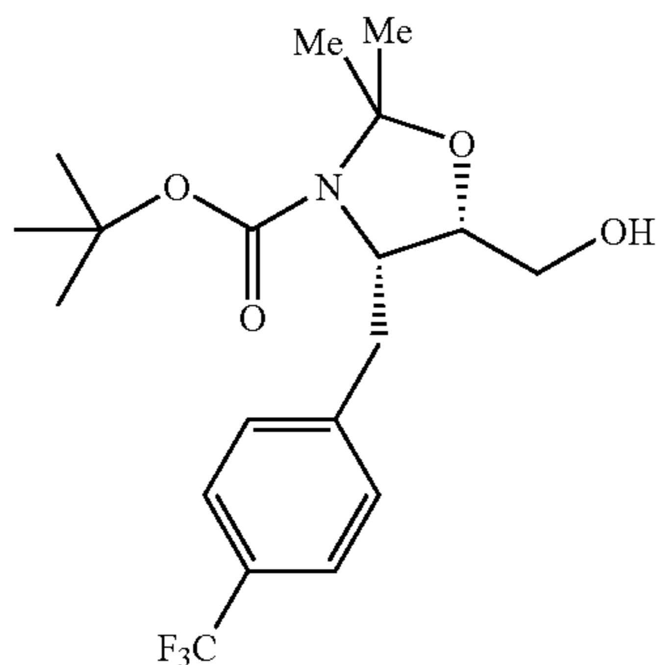
(4S,5S)-tert-butyl 4-(4-(trifluoromethyl)benzyl)-5-(hydroxymethyl)-2,2-dimethyloxazolidine-3-carboxylate
