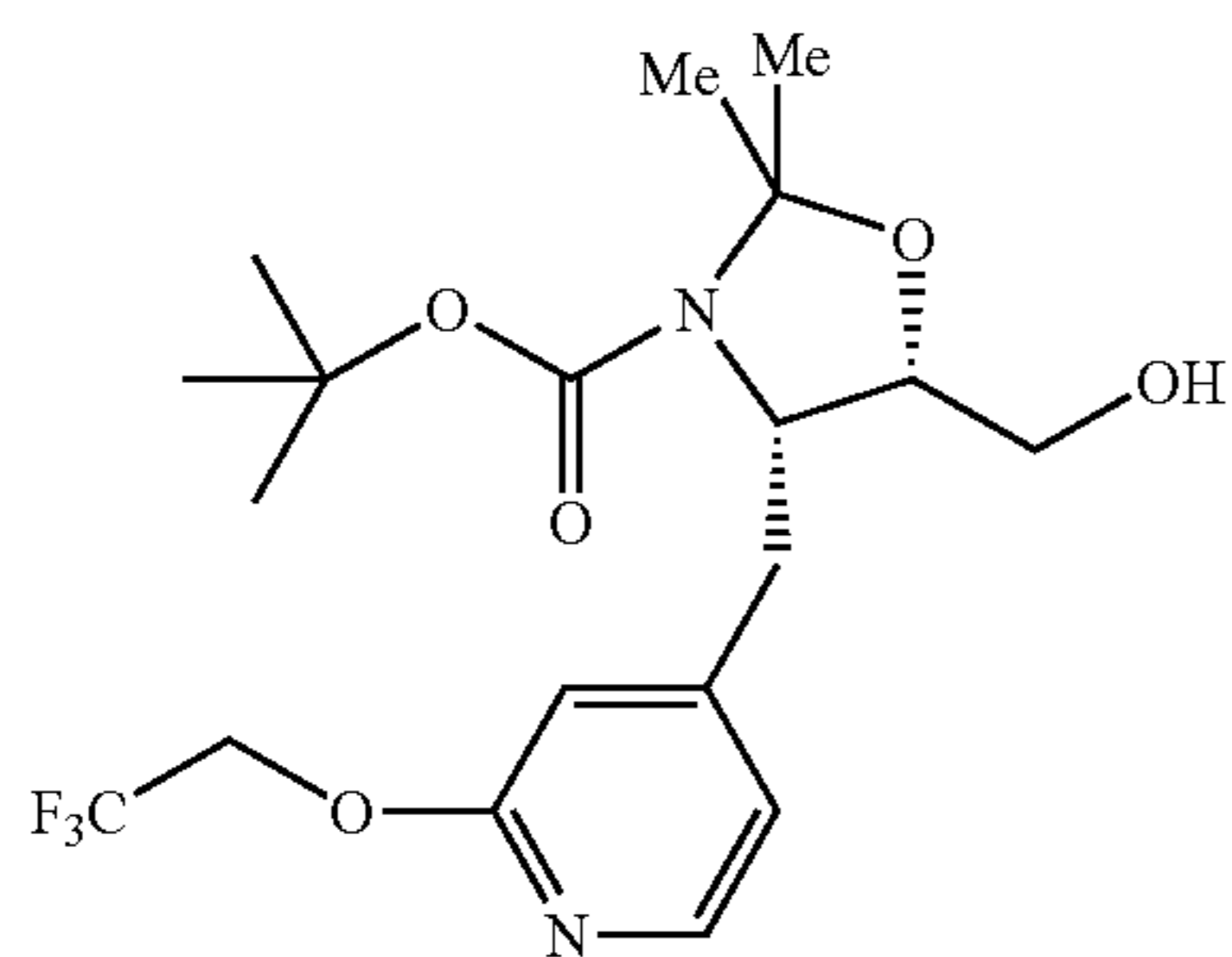
(4S,5S)-tert-butyl 5-(hydroxymethyl)-2,2-dimethyl-4-((2-(2,2,2-trifluoroethoxy)pyridin-4-yl)methyl)oxazolidine-3-carboxylate
