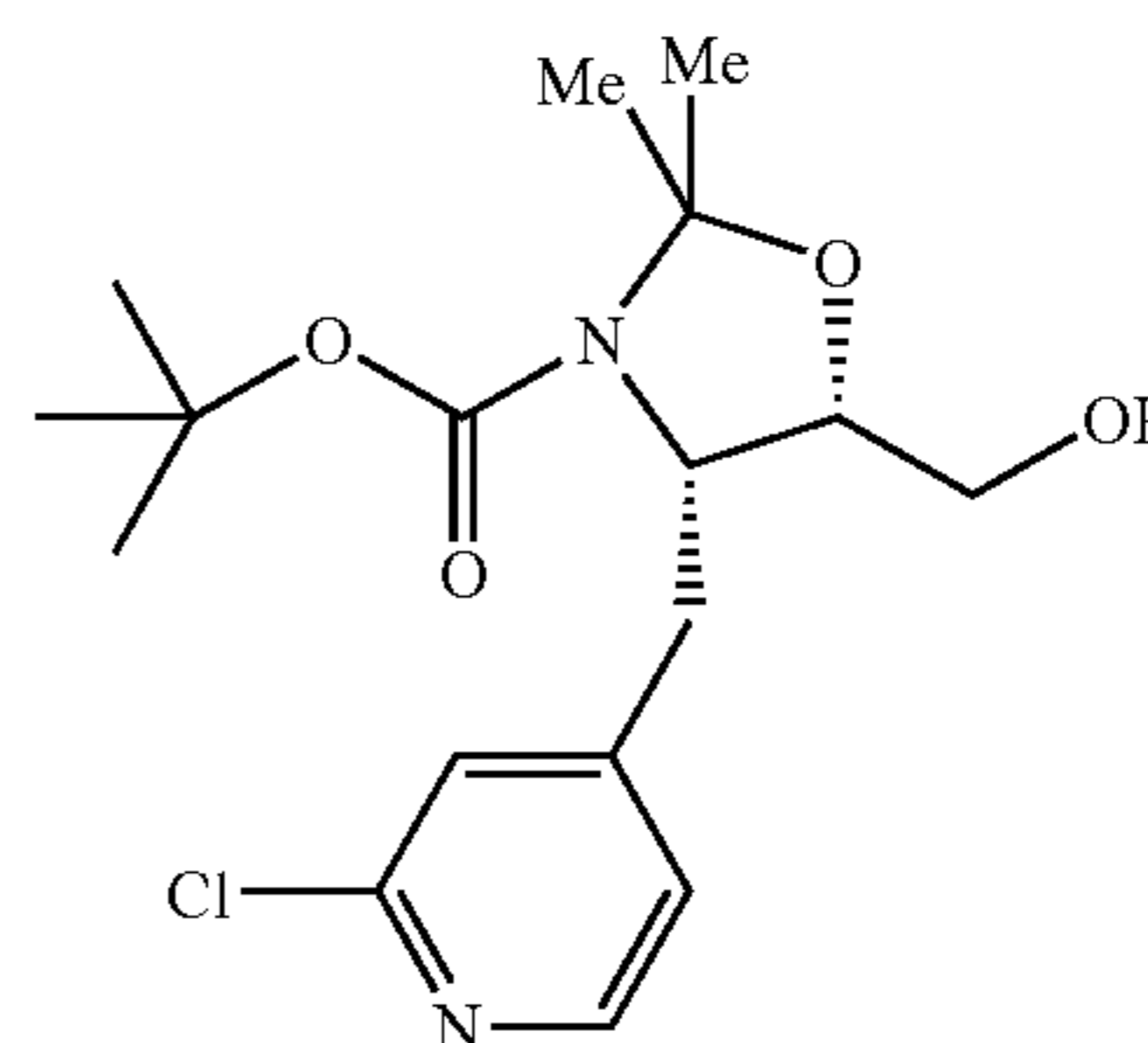
(4S,5S)-tert-butyl 4-((2-chloropyridin-4-yl)methyl)-5-(hydroxymethyl)-2,2-dimethyloxazolidine-3-carboxylate
