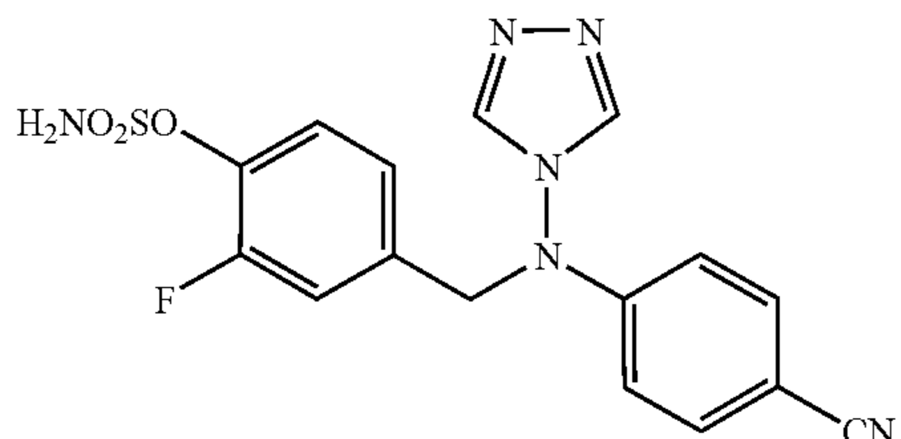
Sulfamic acid-4-[[4-cyano-phenyl]-[1,2,4]triazol-4-yl-amino]-methyl]-2-fluoro-phenyl ester (CAB03021, STX700)
