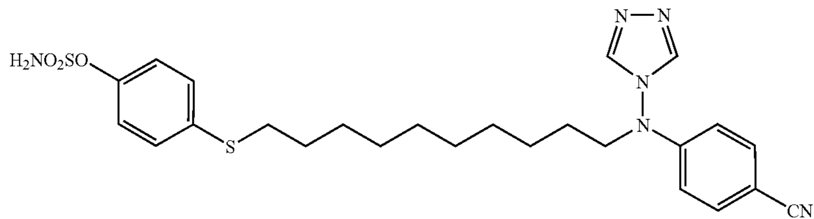
Sulfamic acid 4-{10-[(4-cyano-phenyl)-[1,2,4]triazole-4-yl-amino]-decylsulfanyl}-phenyl ester (CAB03012, STX655)
