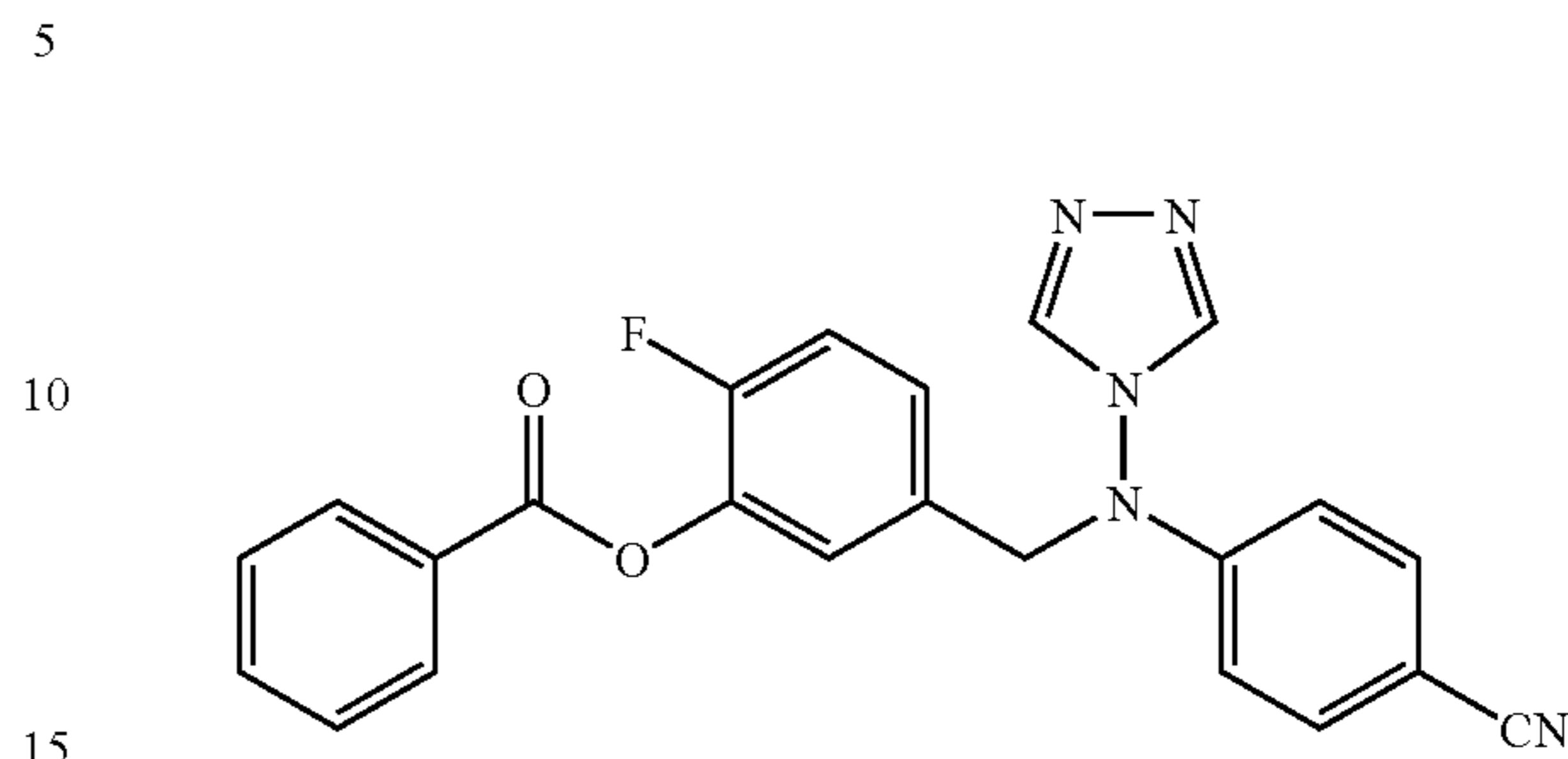
Benzoic Acid 5-[[4-(4-cyano-phenyl)-[1,2,4]triazol-4-yl-amino]methyl]-2-fluoro-phenyl Ester (CAB02147)
