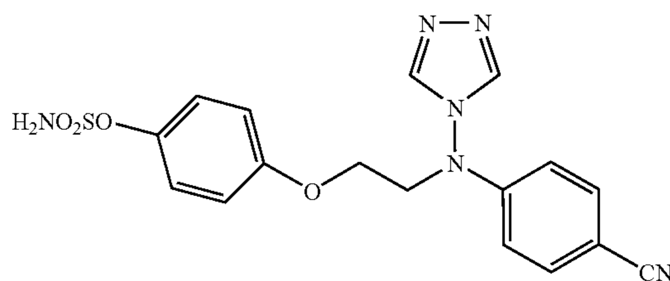
Sulfamic acid 4-[[2-(4-cyanophenyl)-[1,2,4]triazol-4-yl-amino]ethyl]phenyl ester (LWO02066, STX273)
