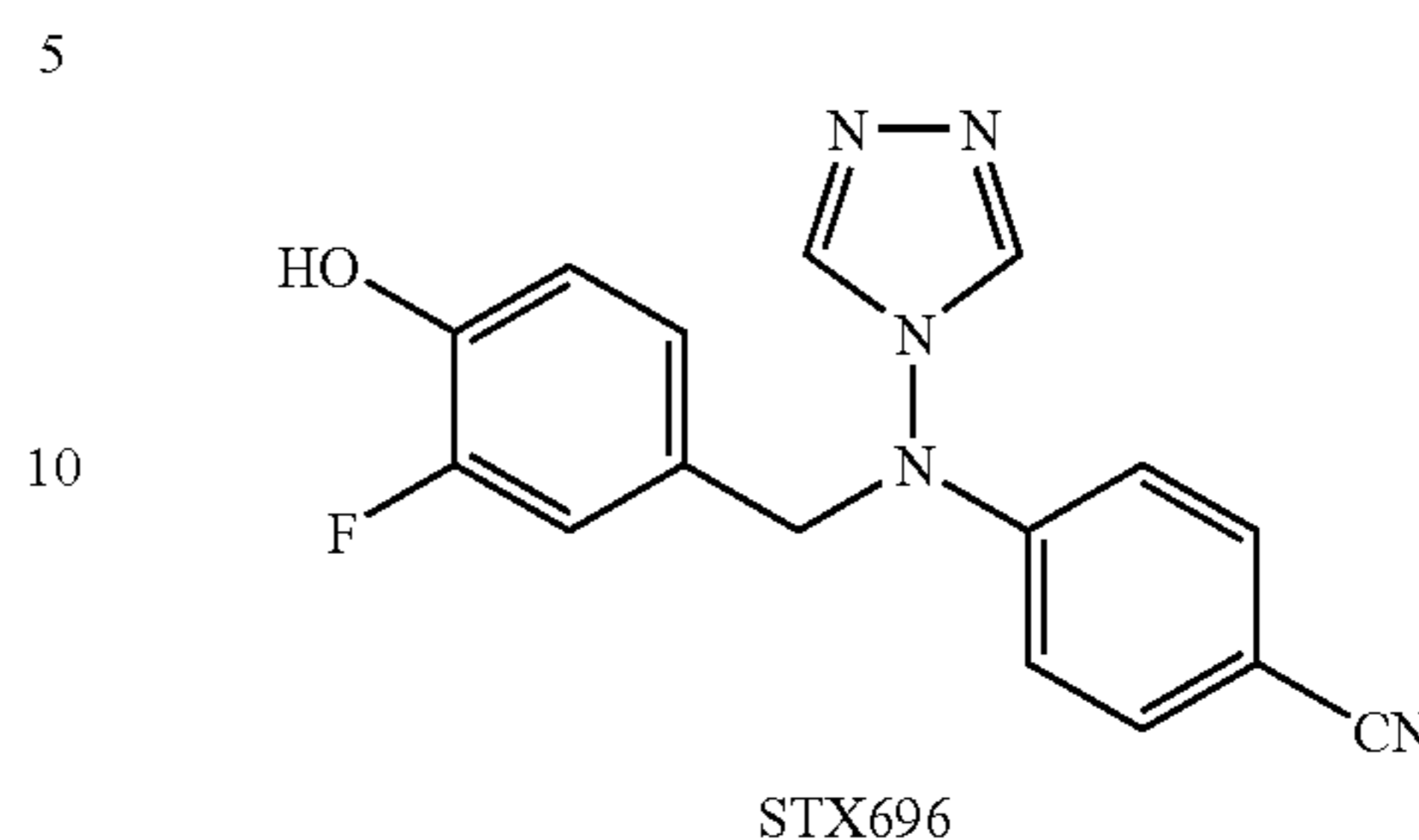
4-[(3-Fluoro-4-hydroxy-benzyl)-[1,2,4]triazol-4-yl-amino]-benzotrile (CAB03020, STX696)
