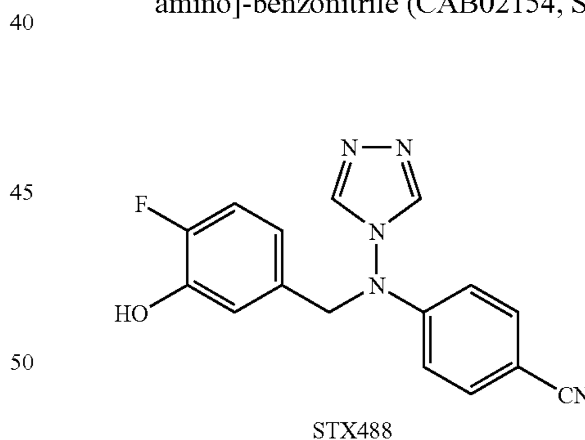
4-[(4-Fluoro-3-hydroxy-benzyl)-[1,2,4]triazol-4-yl-amino]-benzonitrile (CAB02154, STX488)
