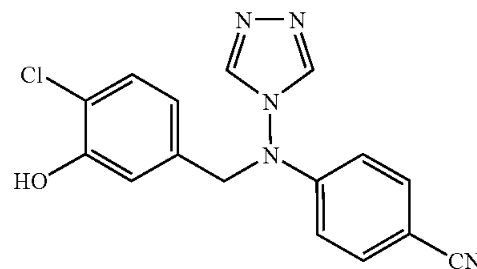
4-[(4-Chloro-3-hydroxy-benzyl)-[1,2,4]triazol-4-yl-amino]-benzonitrile (CAB02141, STX483)
