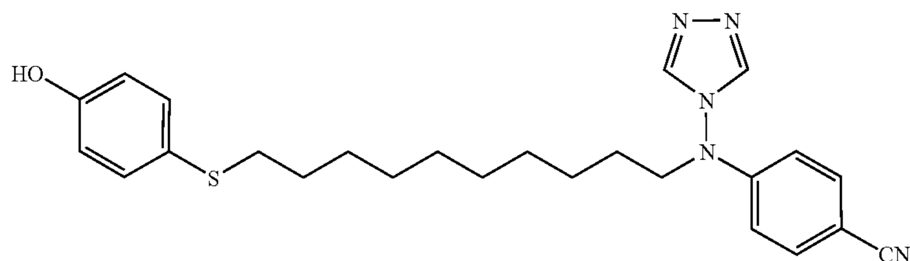
4-[[10-(4-Hydroxy-phenylsulfanyl)-decyl]-[1,2,4]triazole-4-yl-amino]-benzonitrile (CAB03011, STX625)
