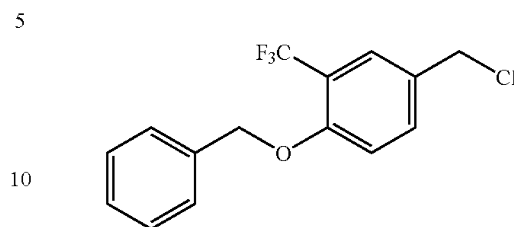
1-Benzyloxy-4-chloromethyl-2-trifluoromethyl-benzene (CAB03050)
