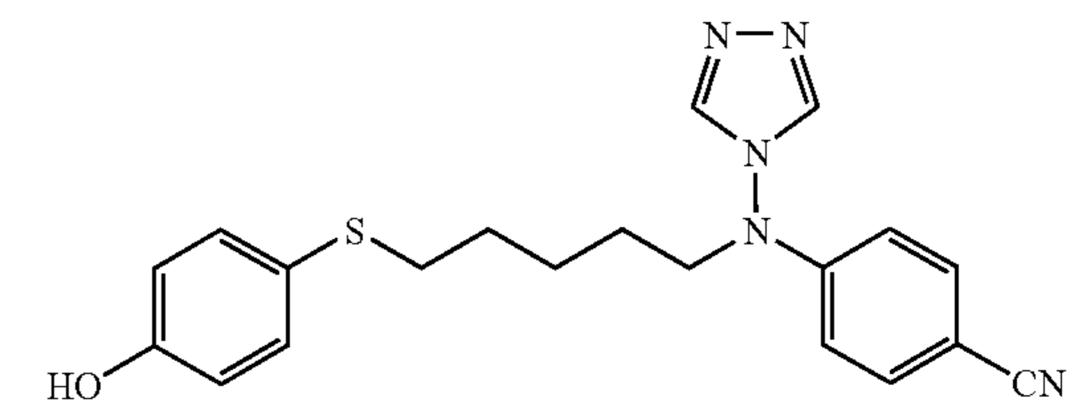
4-[[5-(4-Hydroxy-phenylsulfanyl)-pentyl]-[1,2,4]triazole-4-yl-amino]-benzonitrile (CAB03014, STX698)
