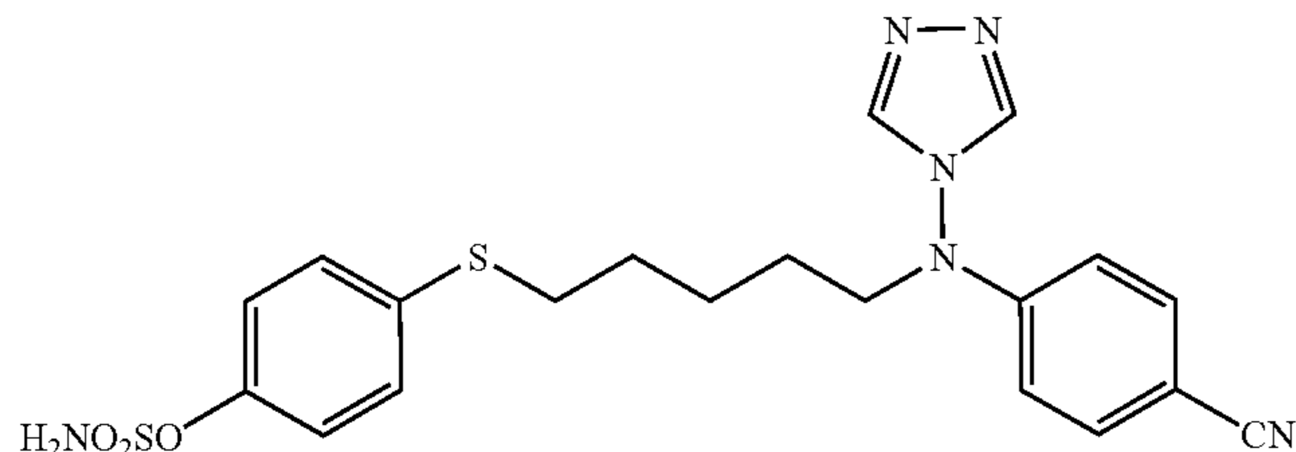
Sulfamic acid 4-[[5-[(4-cyano-phenyl)-[1,2,4]triazole-4-yl-amino]pentylsulfanyl]-phenyl ester (CAB03025, STX699)
