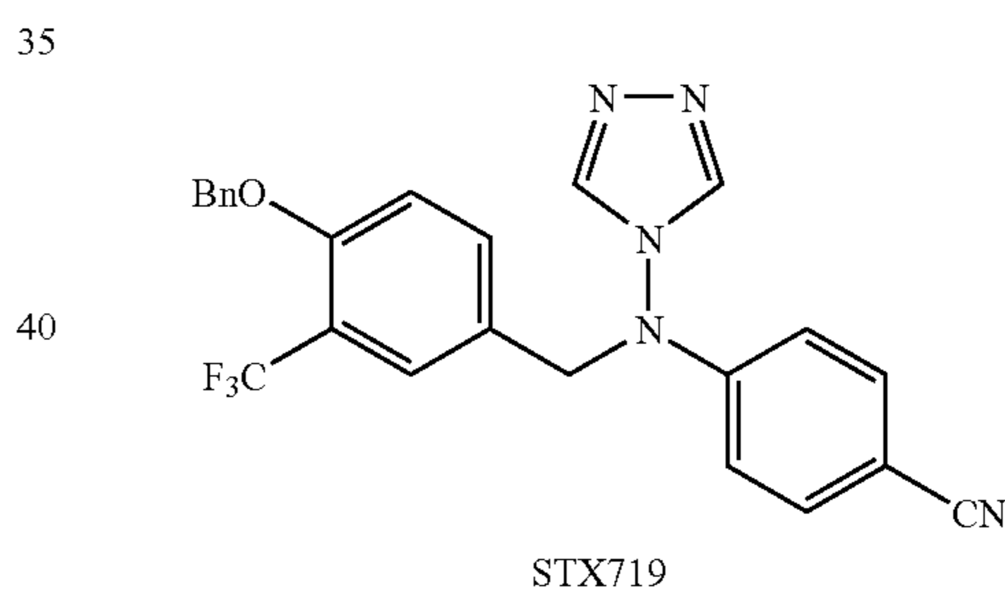
4-[(4-Benzyloxy-3-trifluoromethyl-benzyl)-[1,2,4]triazol-4-yl-amino]-benzonitrile (CAB03054, STX719)
