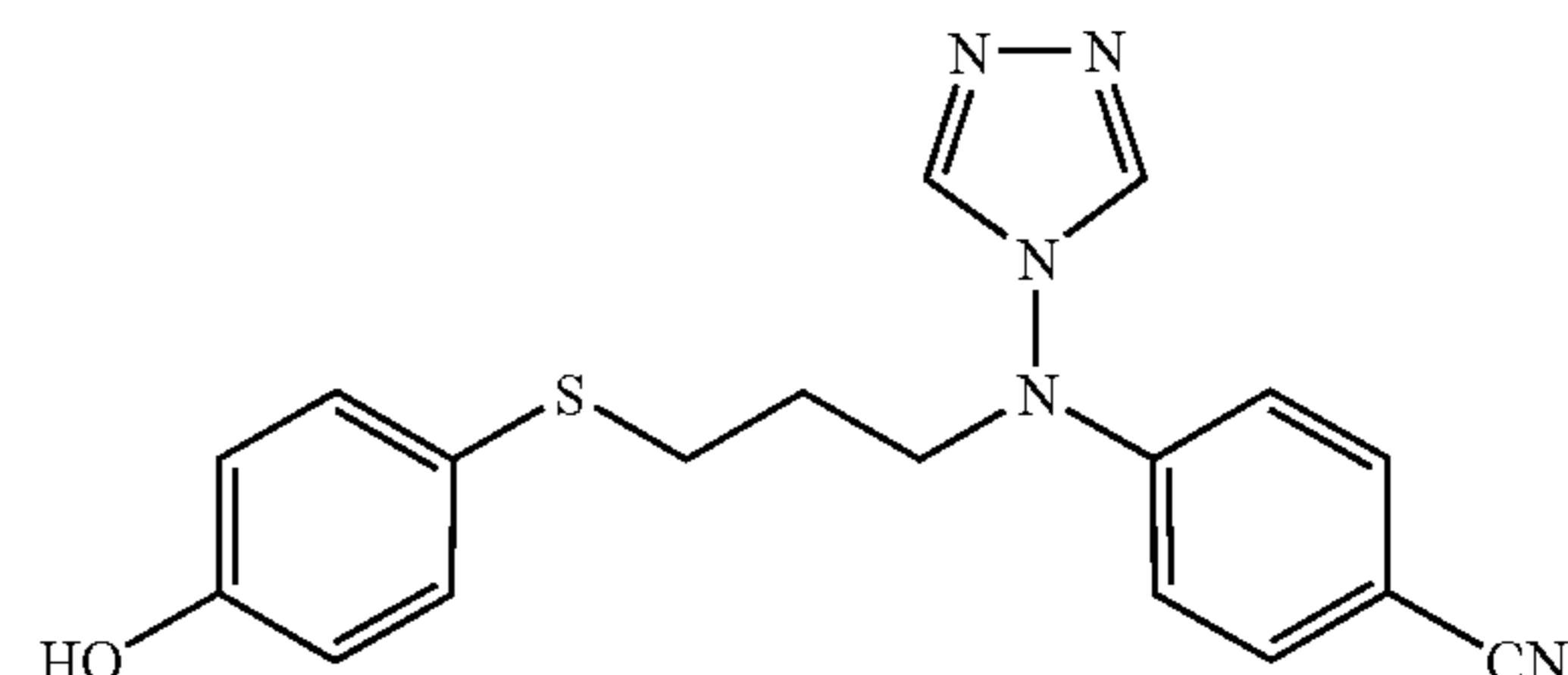
4-[[3-(4-Hydroxy-phenylsulfanyl)-propyl]-[1,2,4]triazole-4-yl-amino]-benzonitrile (CAB0182, STX596)
