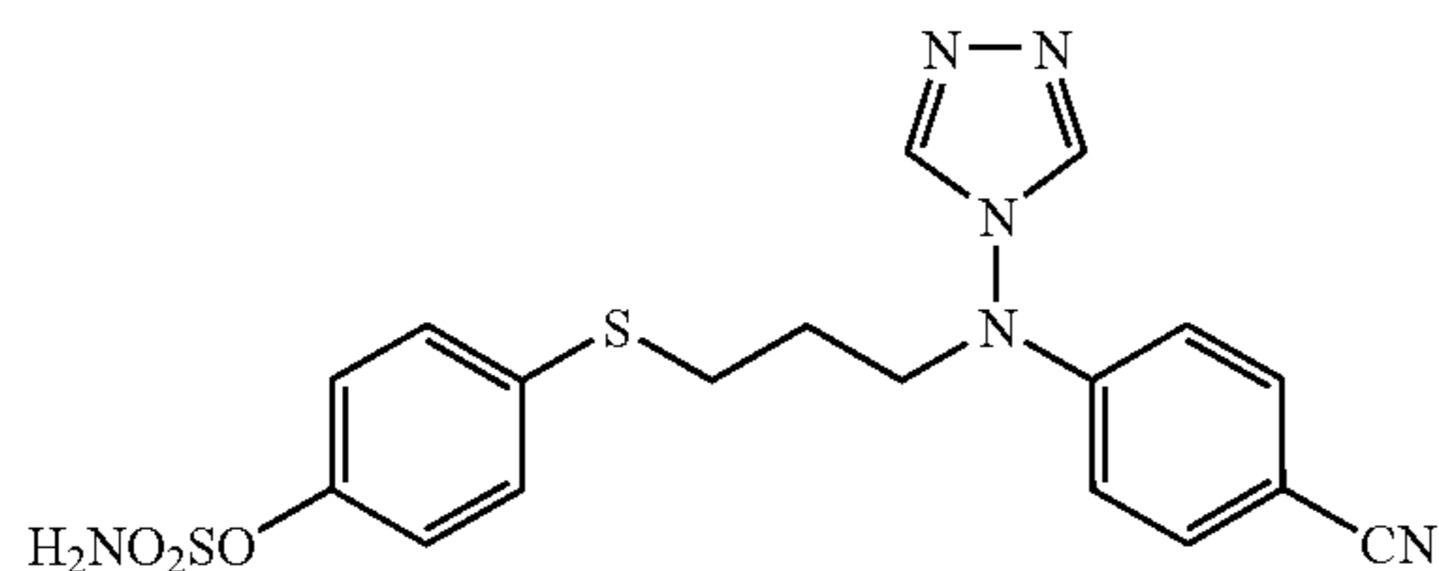
Sulfamic acid 4-[[3-[(4-cyano-phenyl)-[1,2,4]triazole-4-yl-amino]propylsulfanyl]-phenyl ester (CAB02184, STX597)
