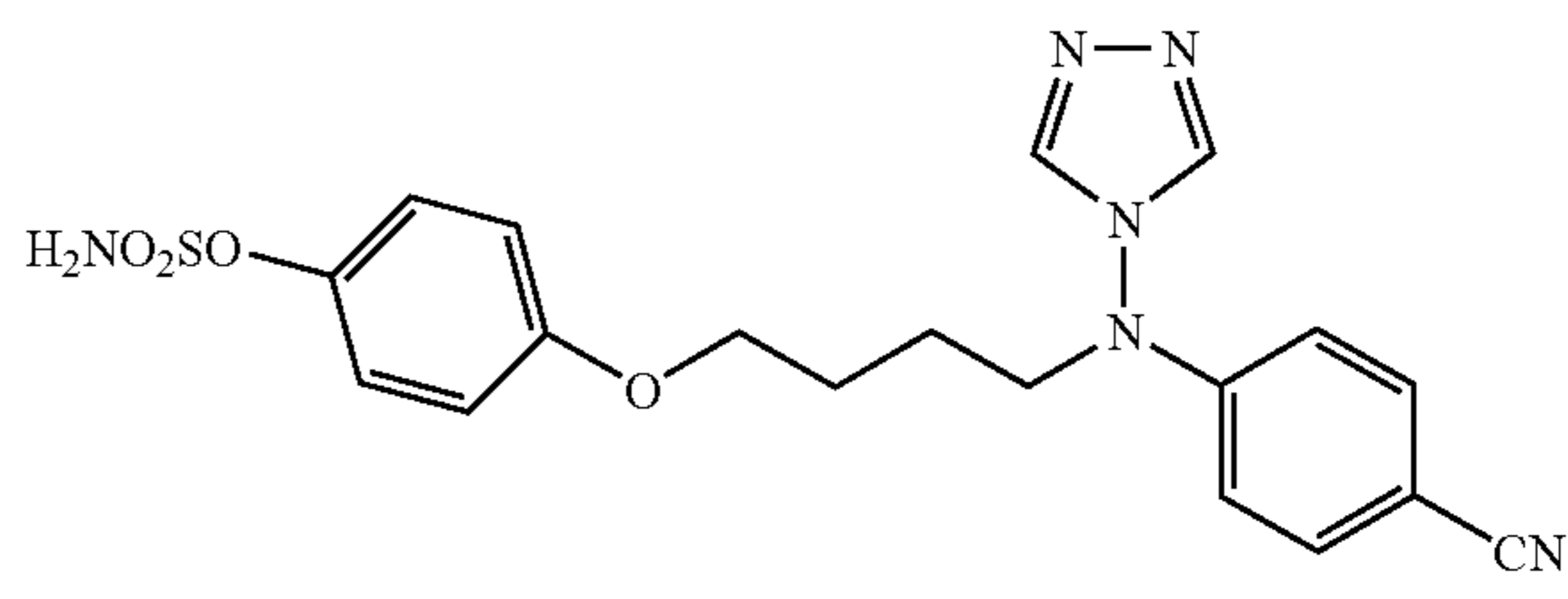
Sulfamic acid 4-[[4-(4-cyanophenyl)-[1,2,4]triazol-4-ylamino]butyl]phenyl ester (LWO02078, STX293)
