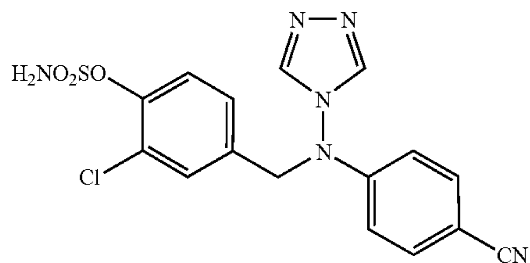
Sulfamic acid 2-chloro-4-[[4-cyano-phenyl]-[1,2,4]triazol-4-yl-amino]-methyl}-phen (CAB02140, STX694)
