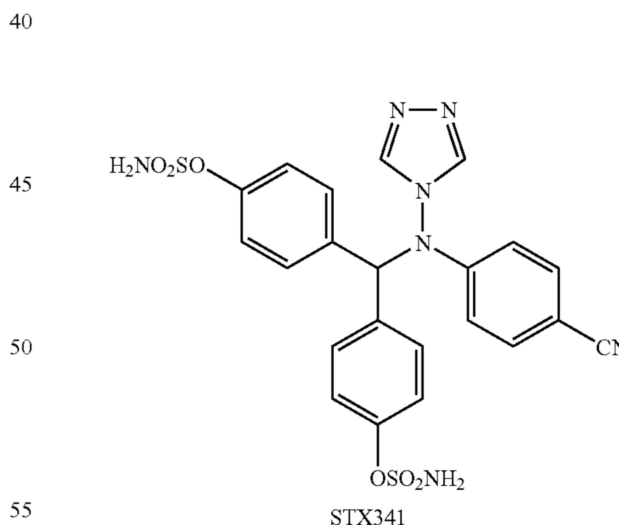
4-[[Bis-(4-sulphamoyloxy-phenyl)-methyl]-[1,2,4]triazol-4-yl-amino]-benzonitrile (CAB02075)
