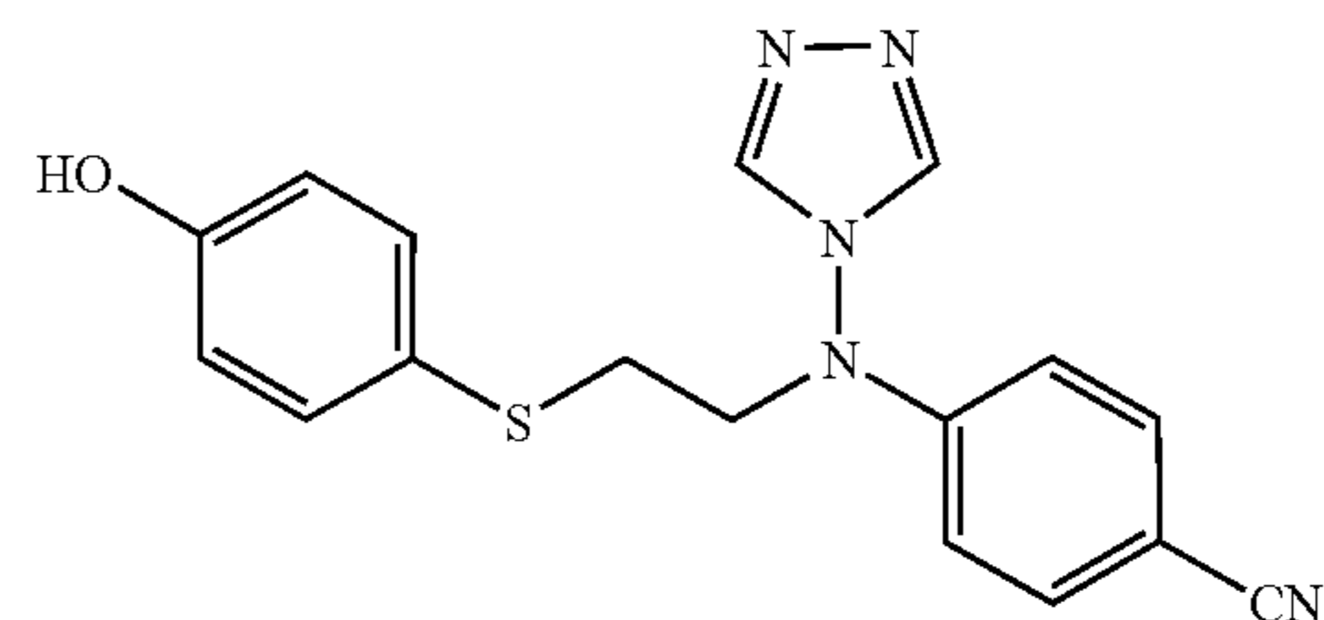
4-[[2-(4-Hydroxy-phenylsulfanyl)-ethyl]-[1,2,4]triazole-4-yl-amino]-benzonitrile (CAB02137, STX465)
