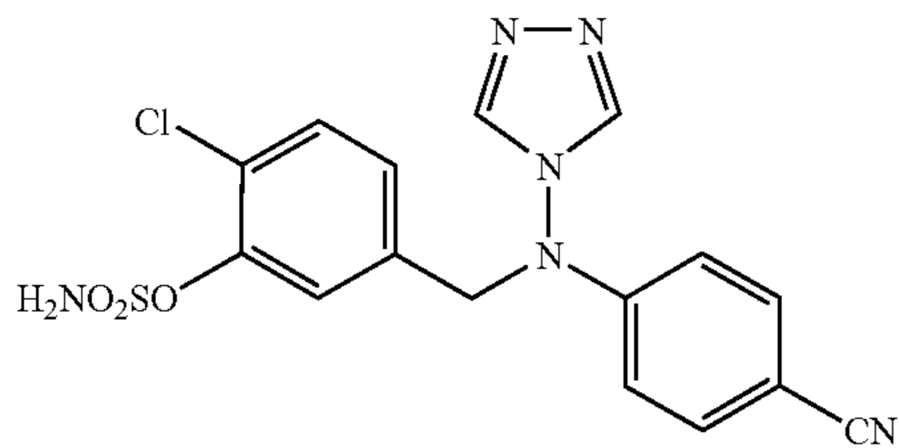
Sulfamic acid 2-chloro-5-[[4-cyano-phenyl]-[1,2,4]triazol-4-yl-amino]-methyl}-phenyl ester (CAB02176, STX559)
