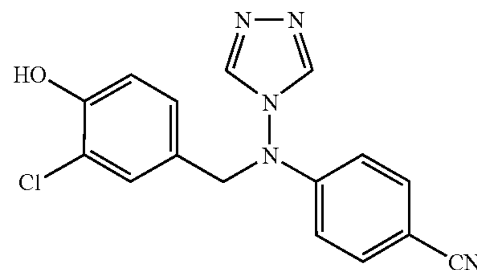
4-[(3-Chloro-4-hydroxy-benzyl)-[1,2,4]triazol-4-yl-amino]-benzonitrile (CAB02130, STX447)
