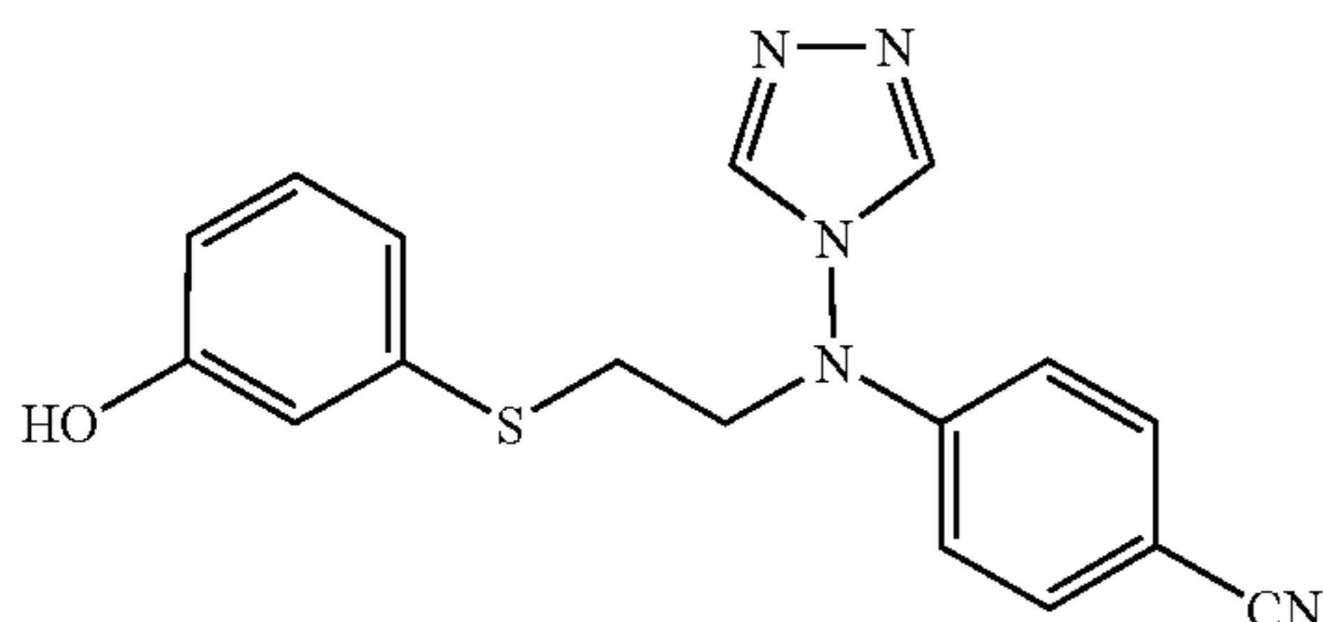
4-[[2-(3-Hydroxy-phenylsulfanyl)-ethyl]-[1,2,4]triazole-4-yl-amino]-benzonitrile (CAB02149, STX512)
