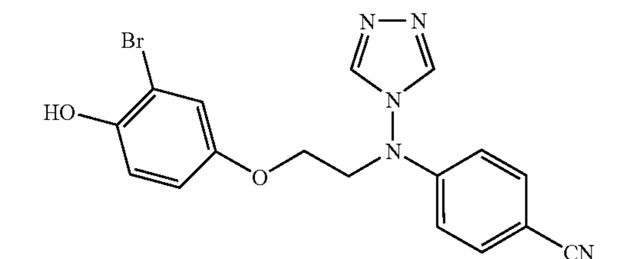
4-[[2-(3-Bromo-4-hydroxyphenoxy)ethyl]-[1,2,4]triazol-4-ylamino]benzonitrile (STX300)
