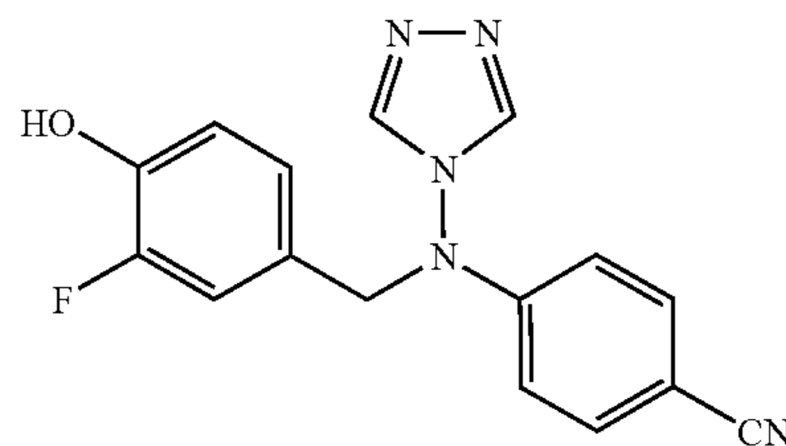
4-[(3-Fluoro-4-hydroxy-benzyl)-[1,2,4]triazol-4-yl-amino]-benzonitrile (CAB03020, STX696)
