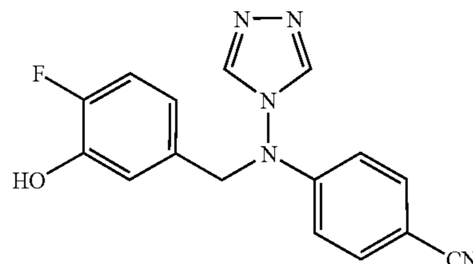
4-[(4-Fluoro-3-hydroxy-benzyl)-[1,2,4]triazol-4-yl-amino]-benzonitrile (CAB02154, STX488)
