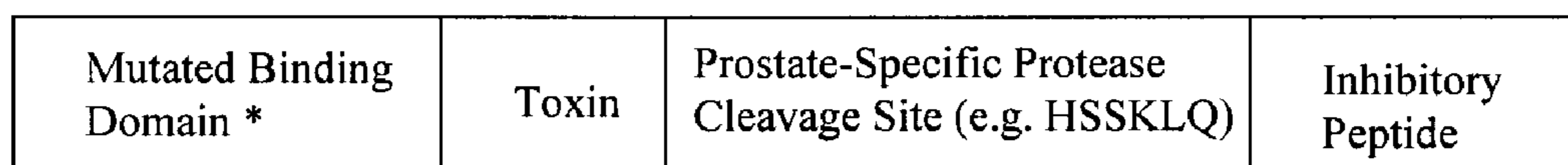
FIG. 5D Example of a Variant Proaerolysin with a Functionally Deleted Binding Domain
