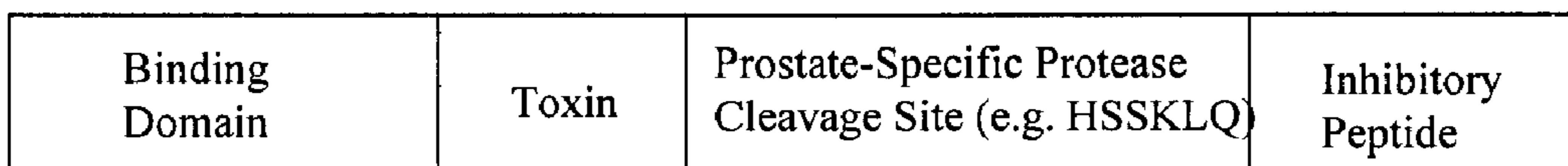
FIG. 5B: Example of a Variant Proaerolysin (SEQ ID NOS: 3 and 4)
