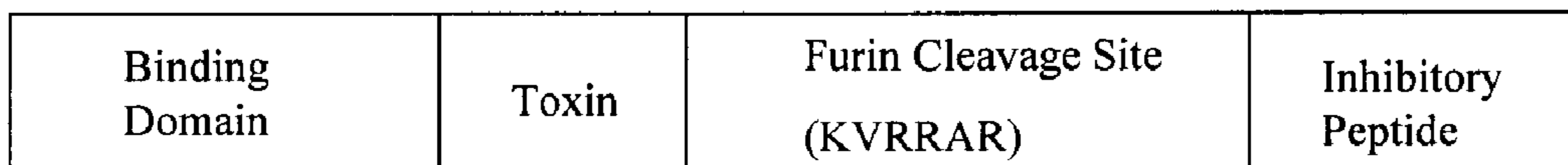
FIG. 5A: Wild-type Proaerolysin (SEQ ID NOS: 1 and 2)
