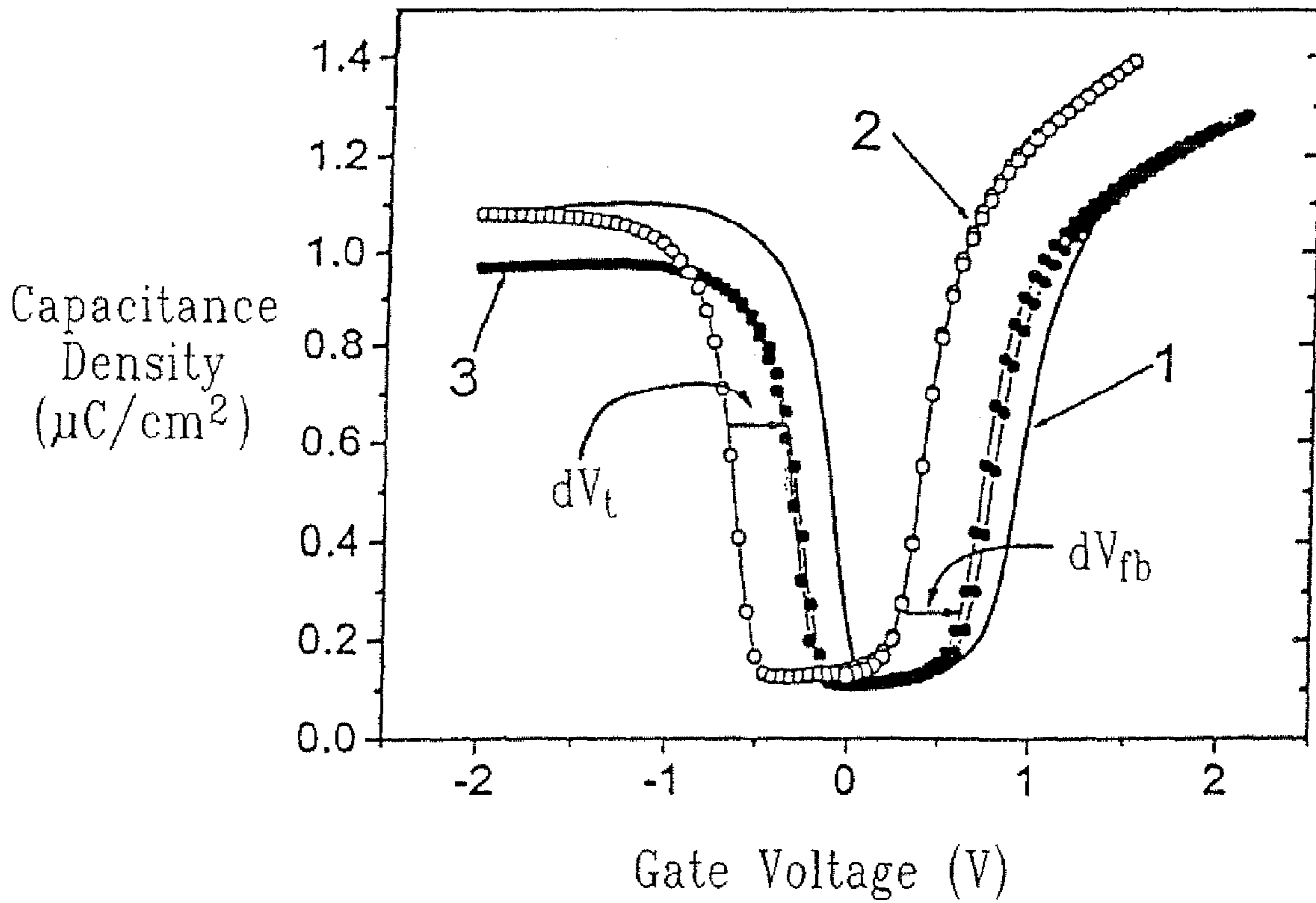
FIG. 2 (PRIOR ART)
