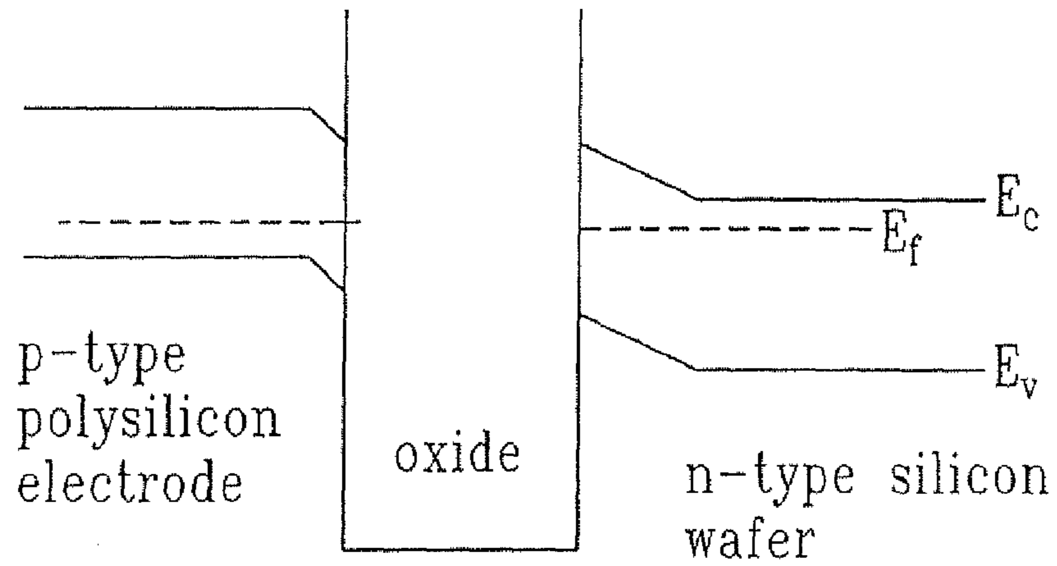
FIG. 1 (PRIOR ART)
