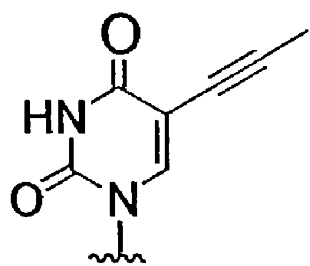
5-propynyl-U
