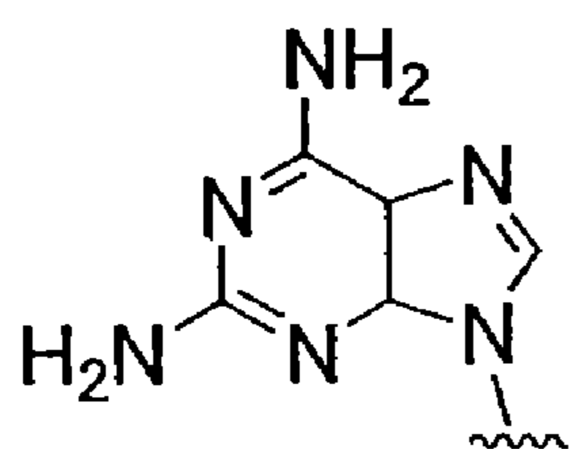
N9-(2,6,-diaminopurine)
