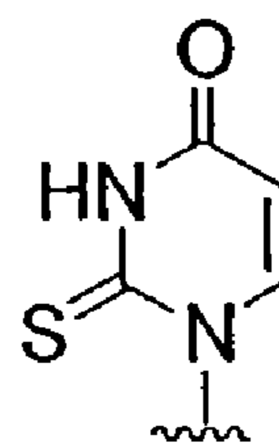
2-thio-U
