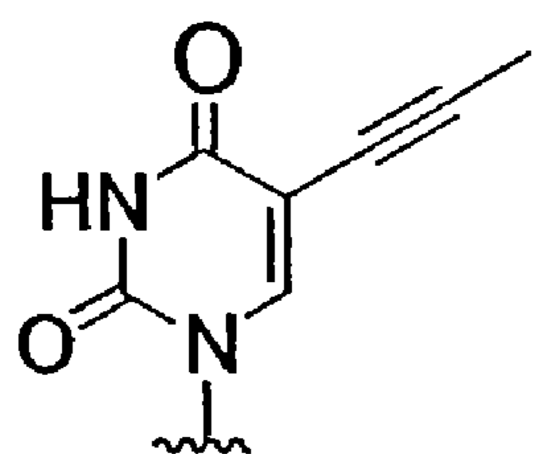
5-propynyl-U
