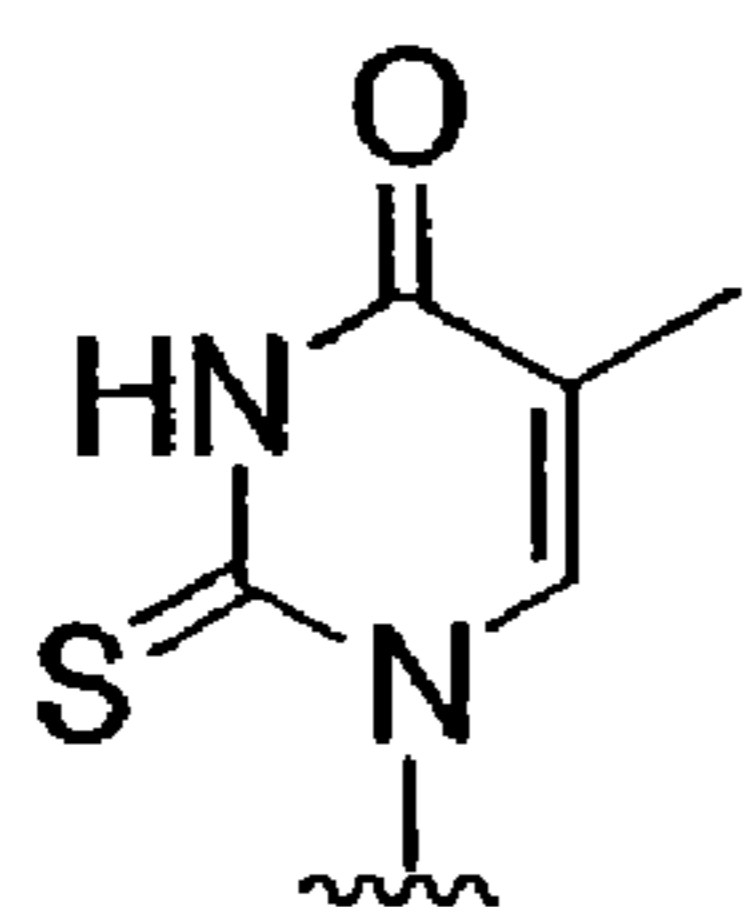
2-thio-T
