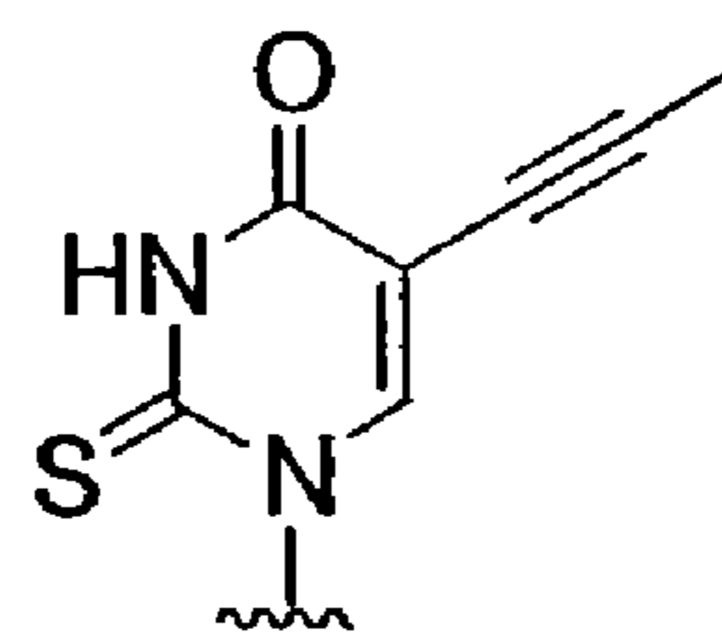
2-thio-5-propynyl-U
