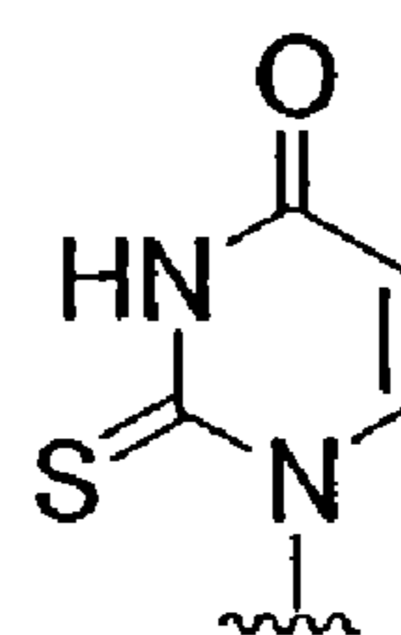
2-thio-U
