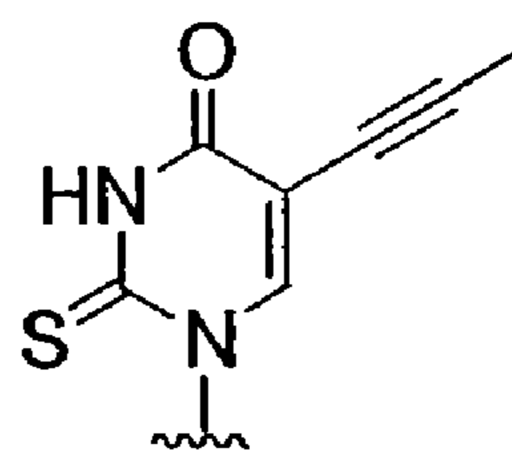
2-thio-5-propynyl-U
