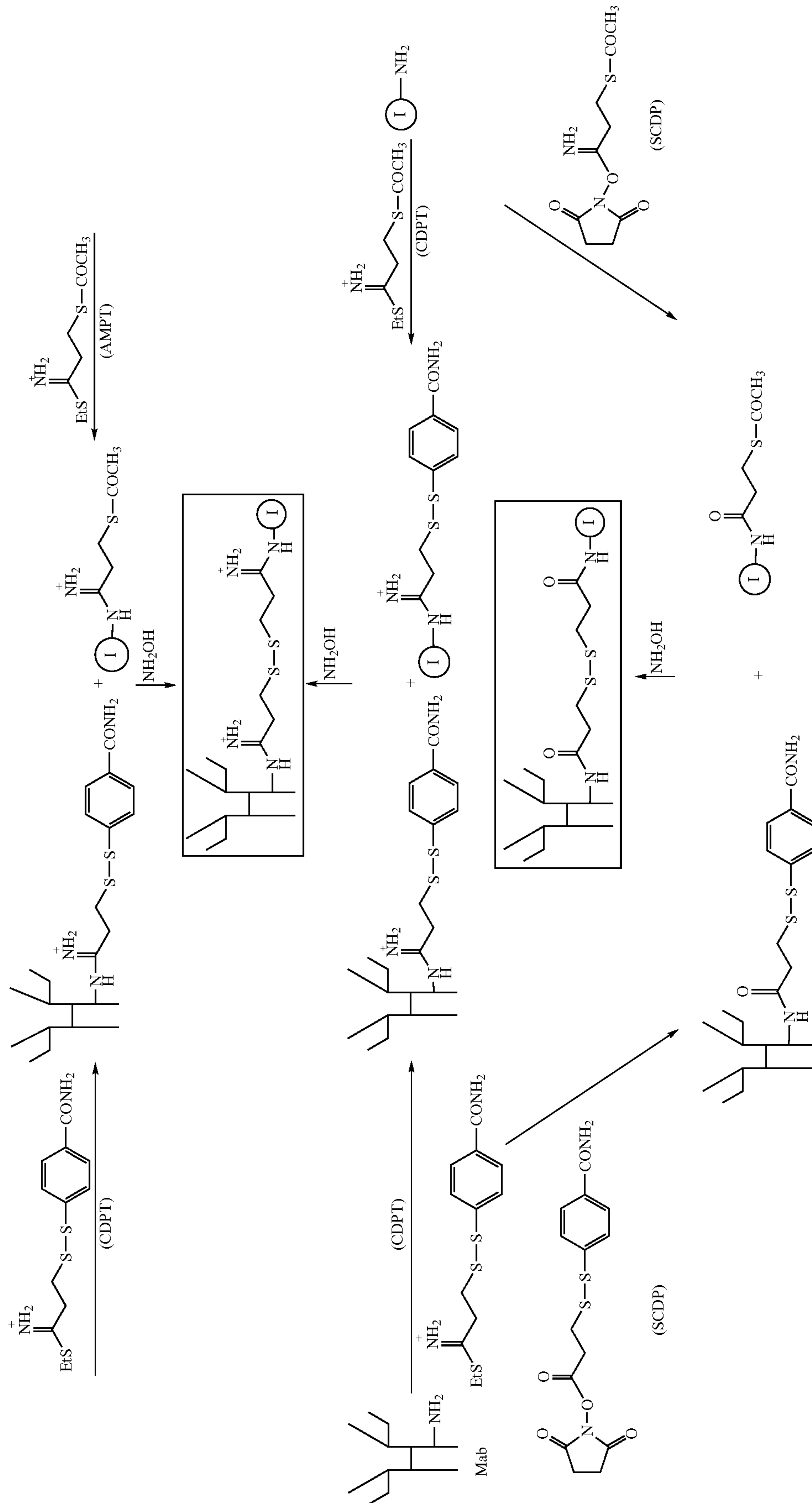
Scheme 13
