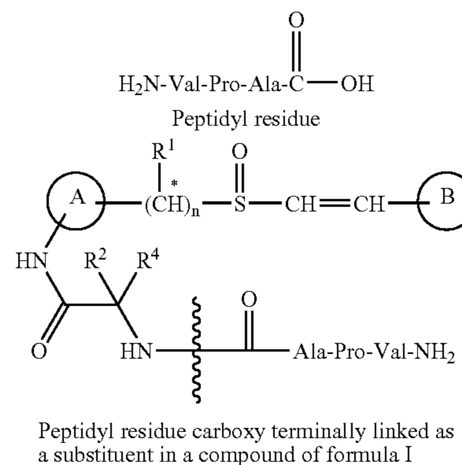
Scheme 1
