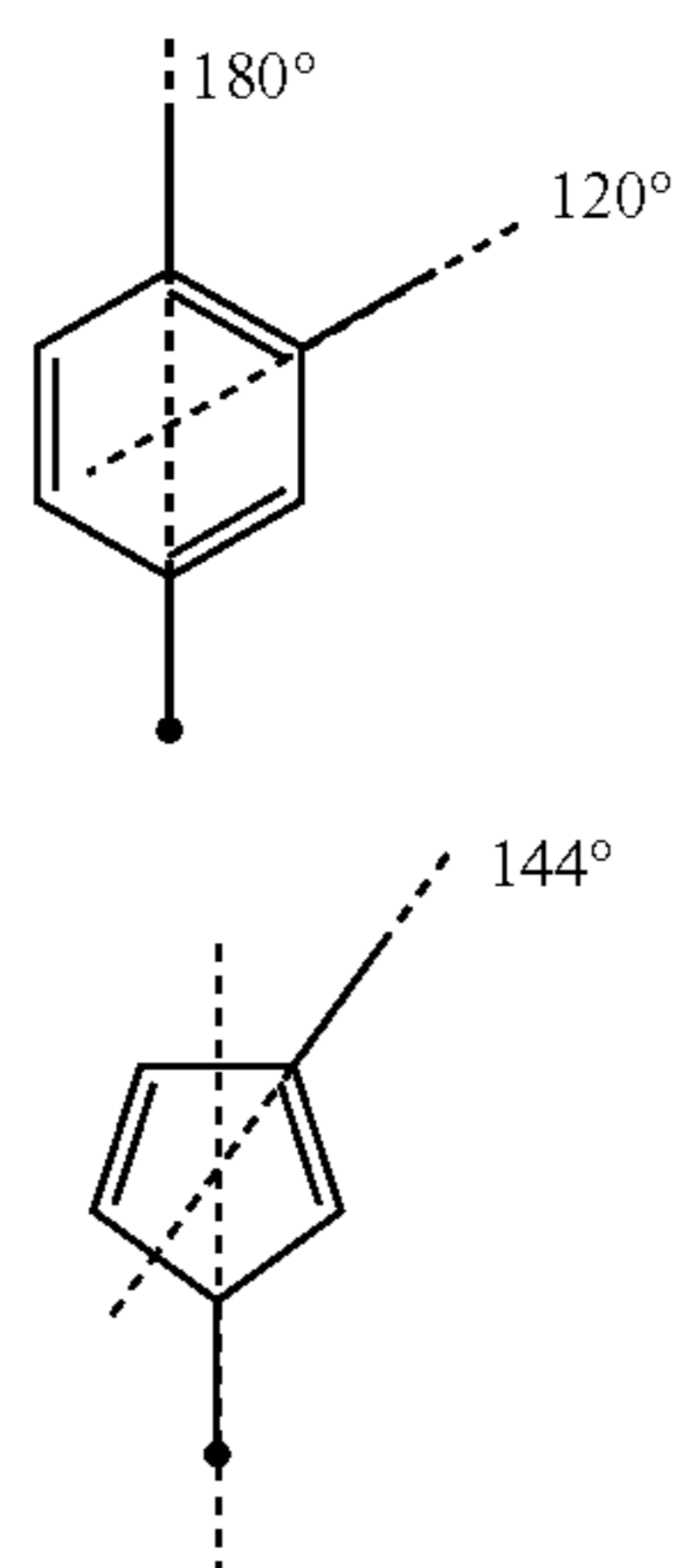
Scheme 4
