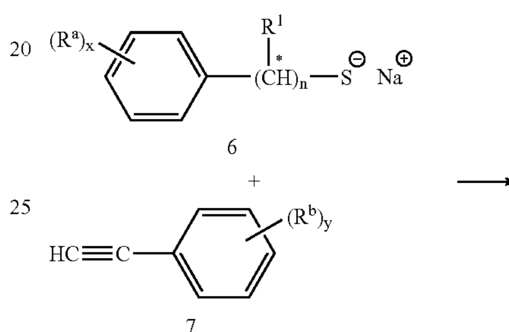
Scheme 10
