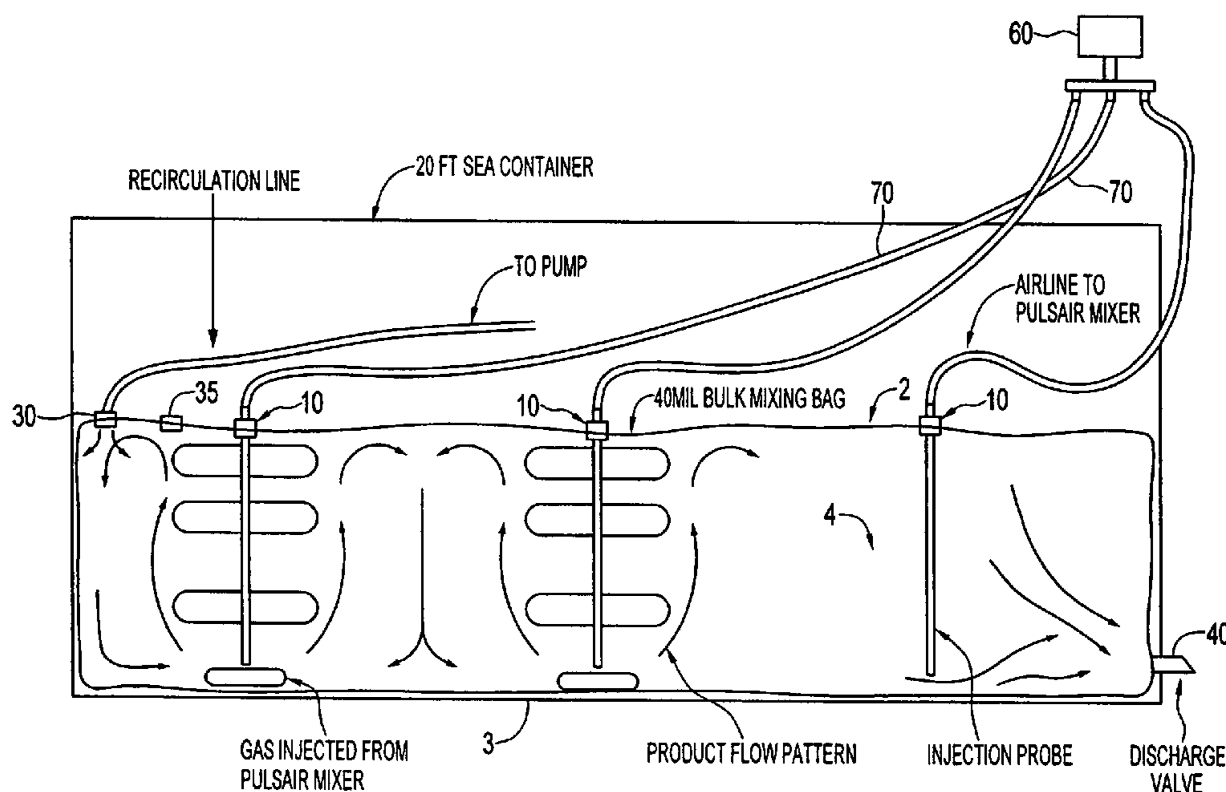
# OF INJECTION POINTS DEPENDENT ON SIZE OF BAG AND THICKNESS OF PRODUCT
