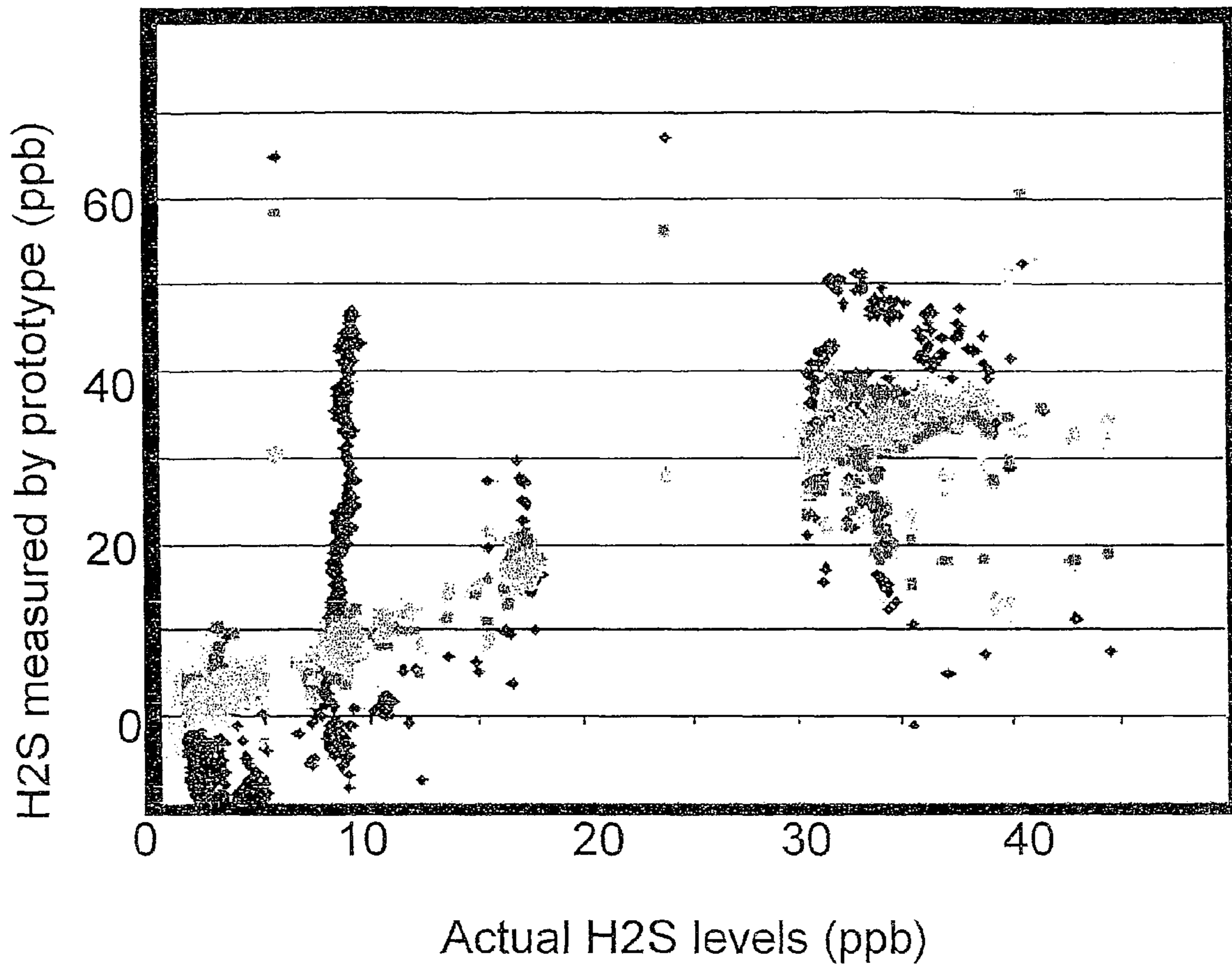
Figure 4: Multiple sensors
