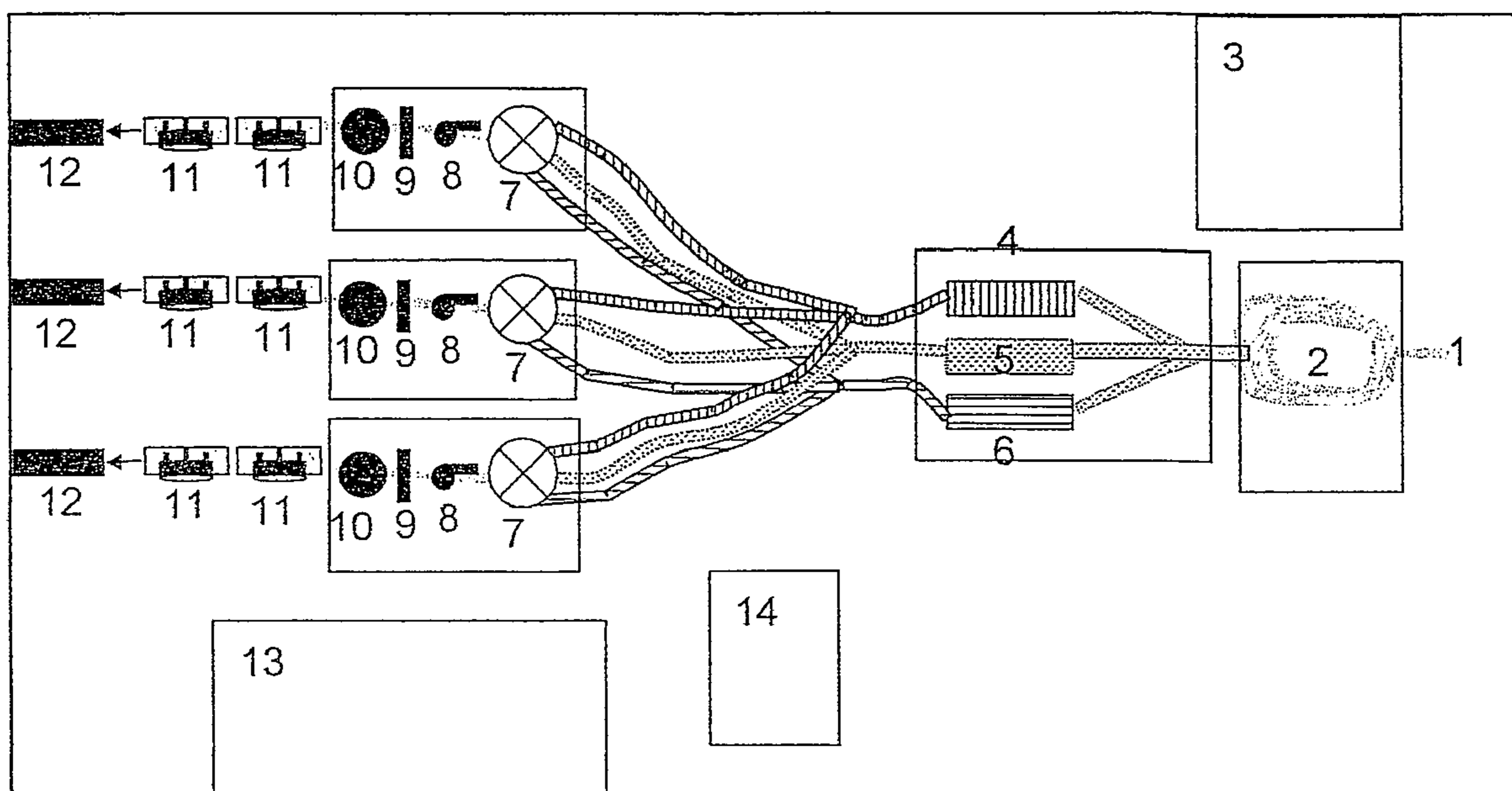
Figure 11: Schematic layout of monitor
