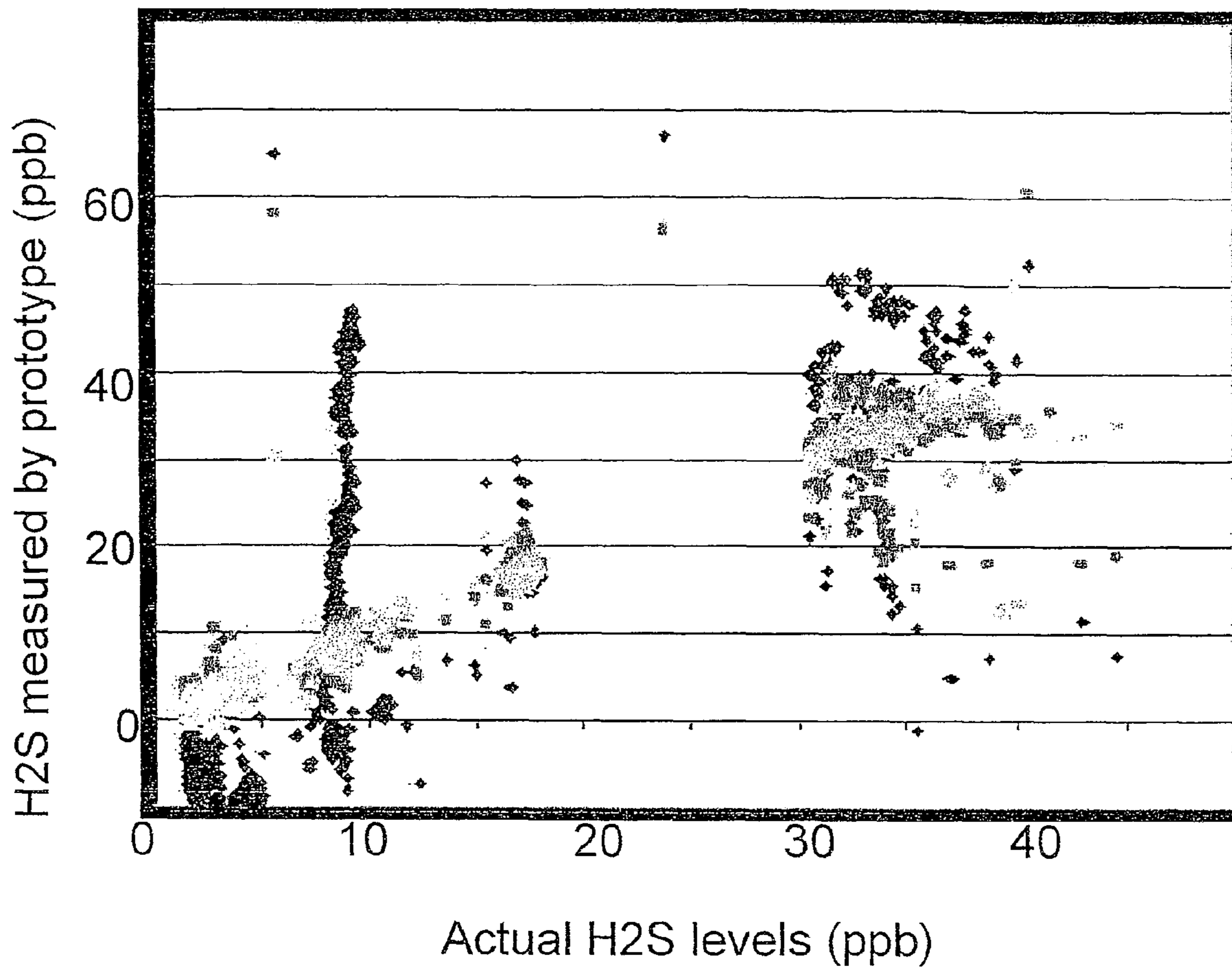
Figure 3: Sensitivity corrected output
