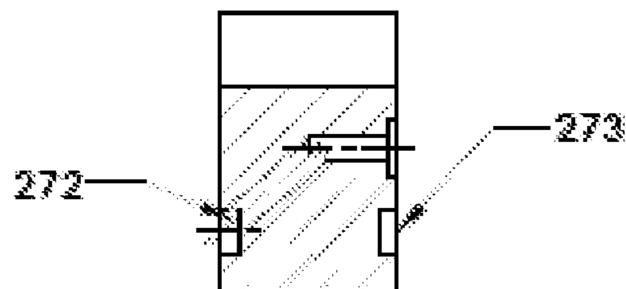
SECTION B-B
