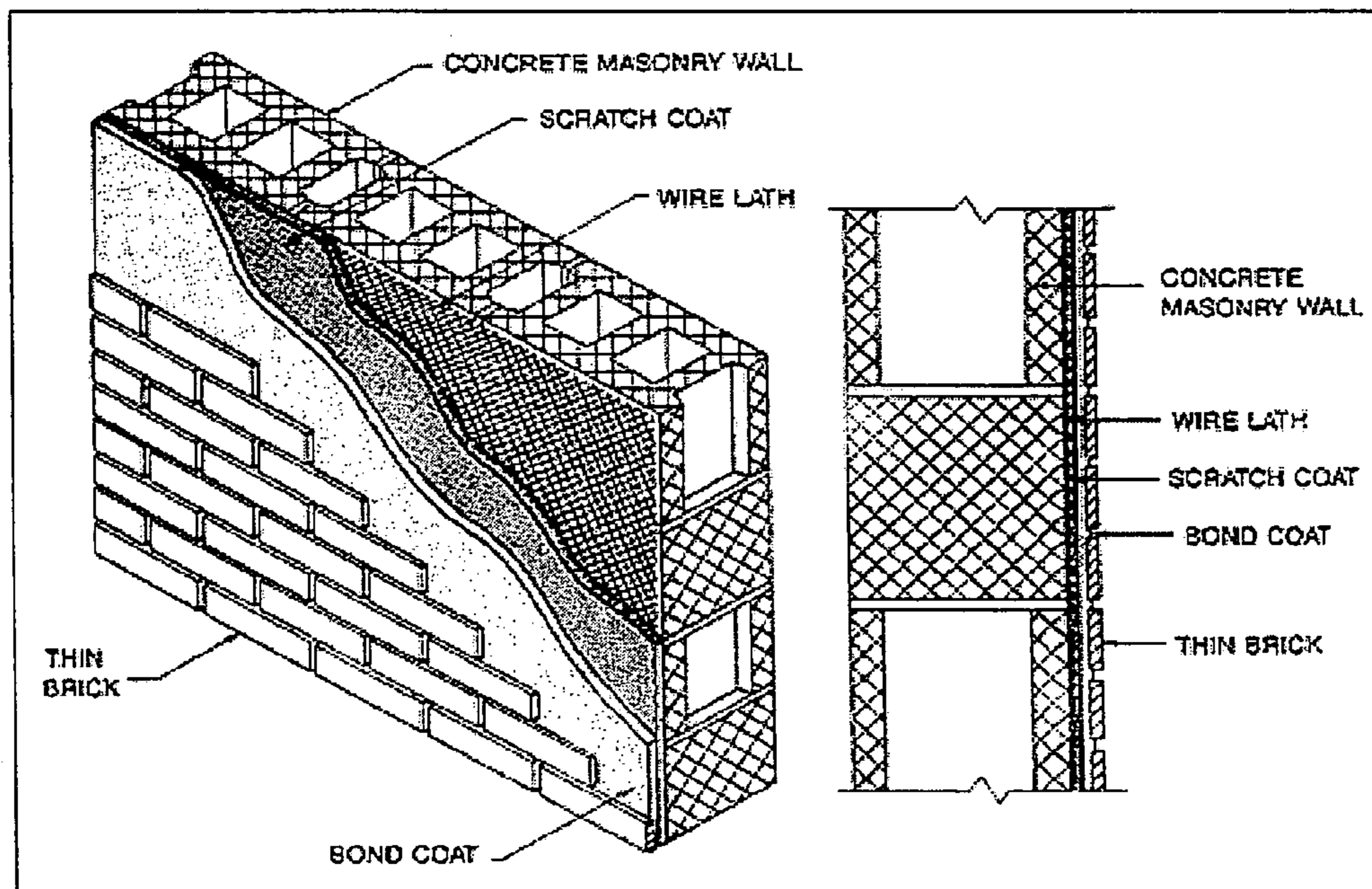
Prior Art Thick Set Method Over Masonry
