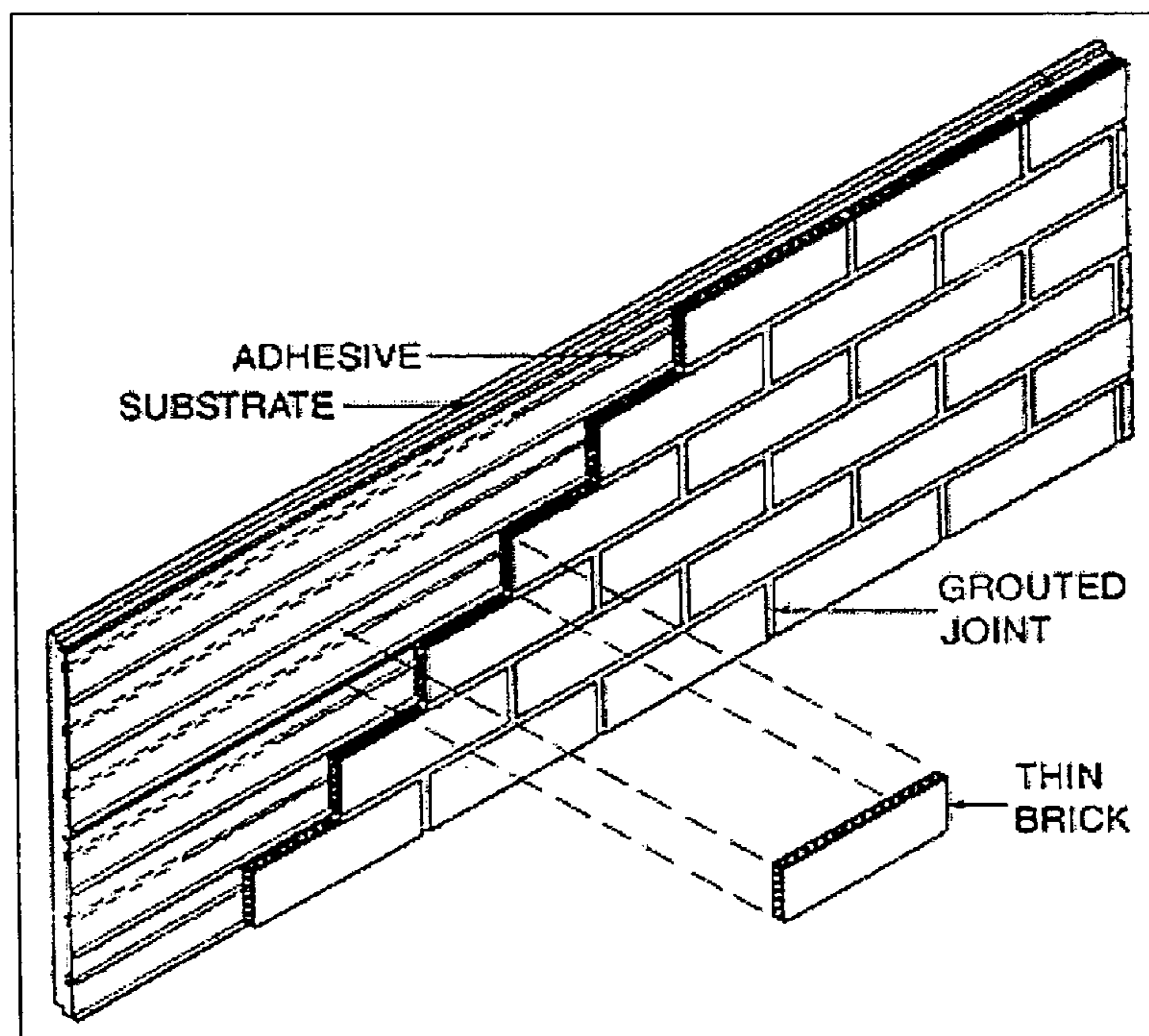
Prior Art Thin Brick Panel
