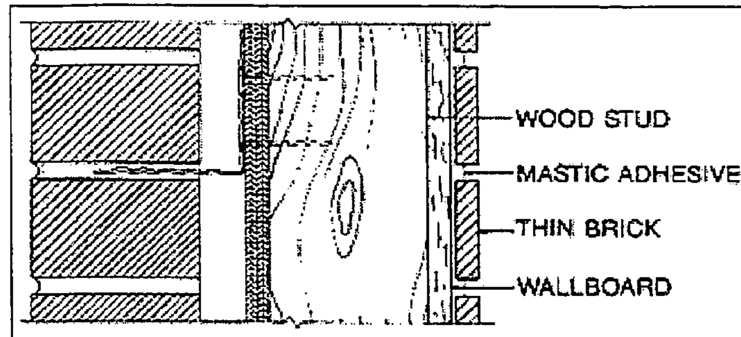
Prior Art Thin Set Interior Finish Over Wallboard
