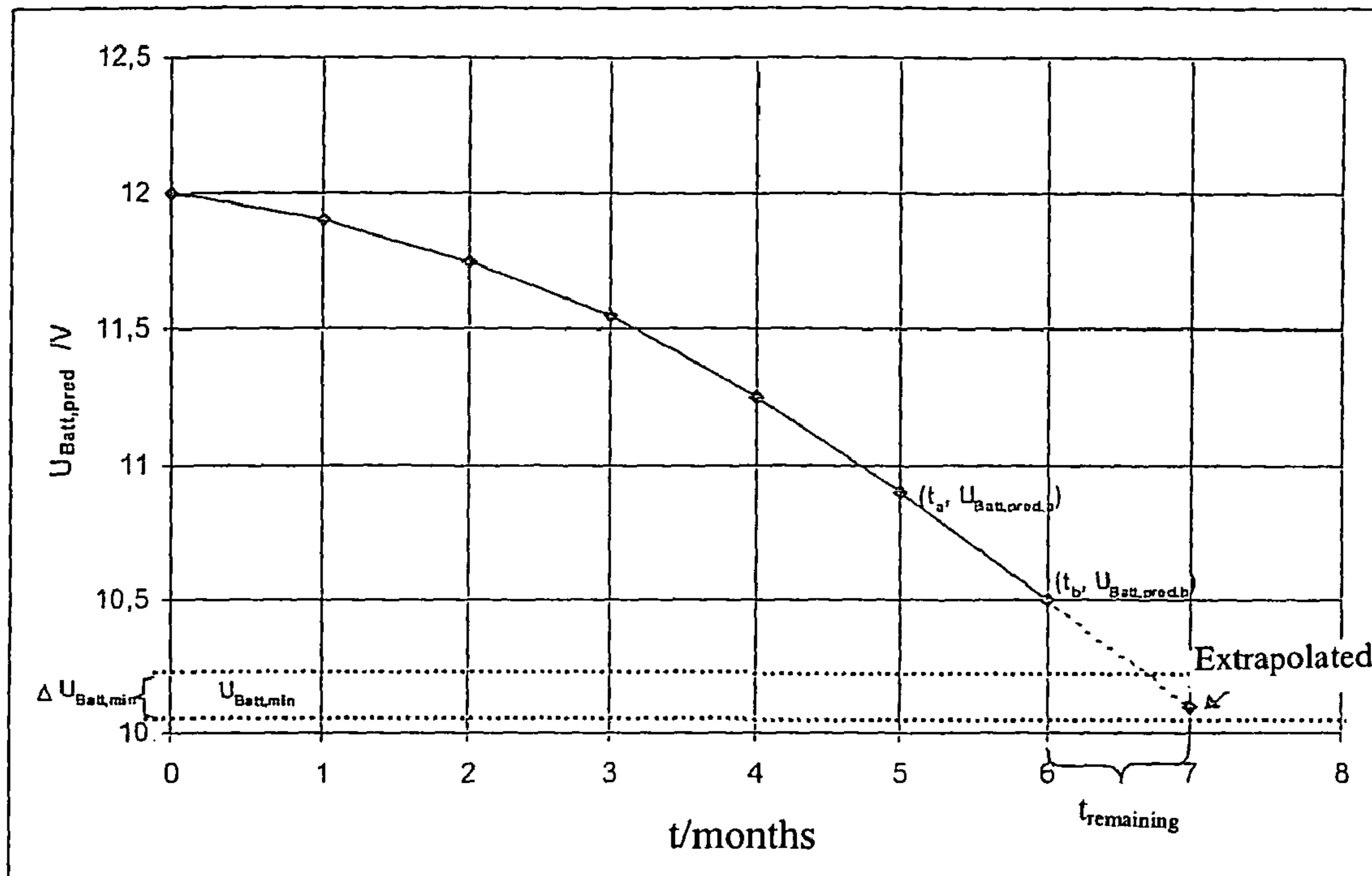
Figure 2: Extrapolation of the example of voltage prediction
