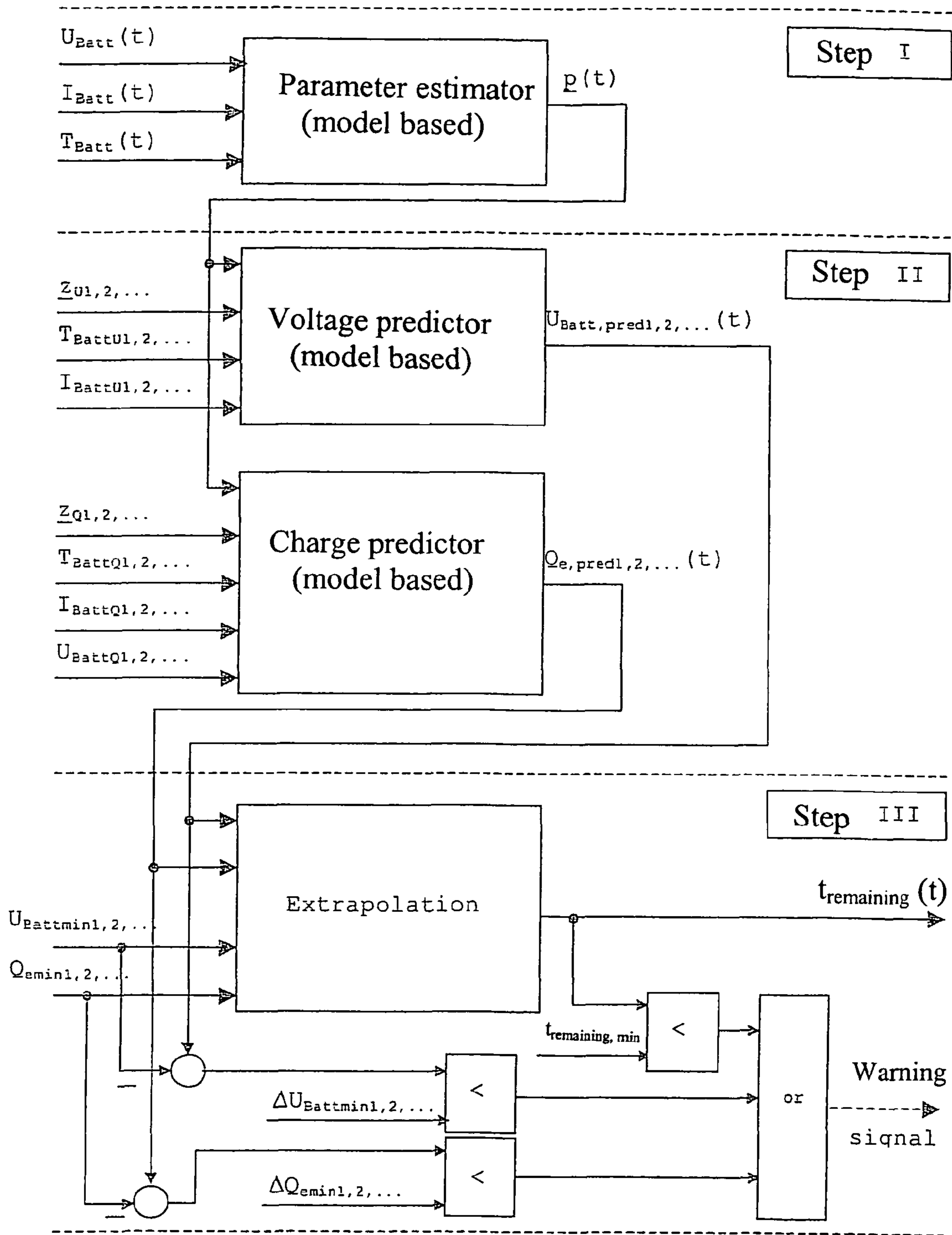
Figure 1: Structure of the lifetime predictor
