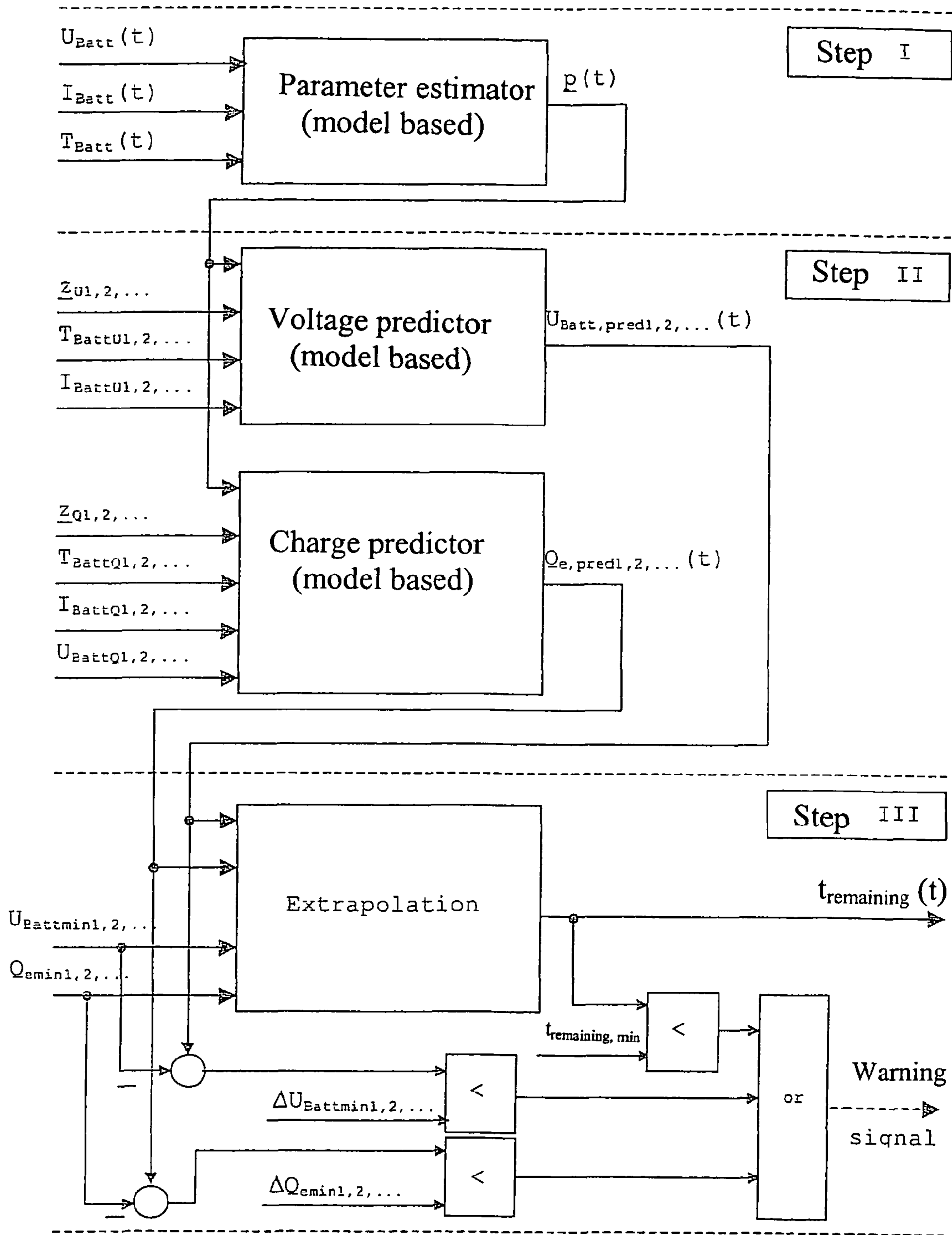
Figure 1: Structure of the lifetime predictor
