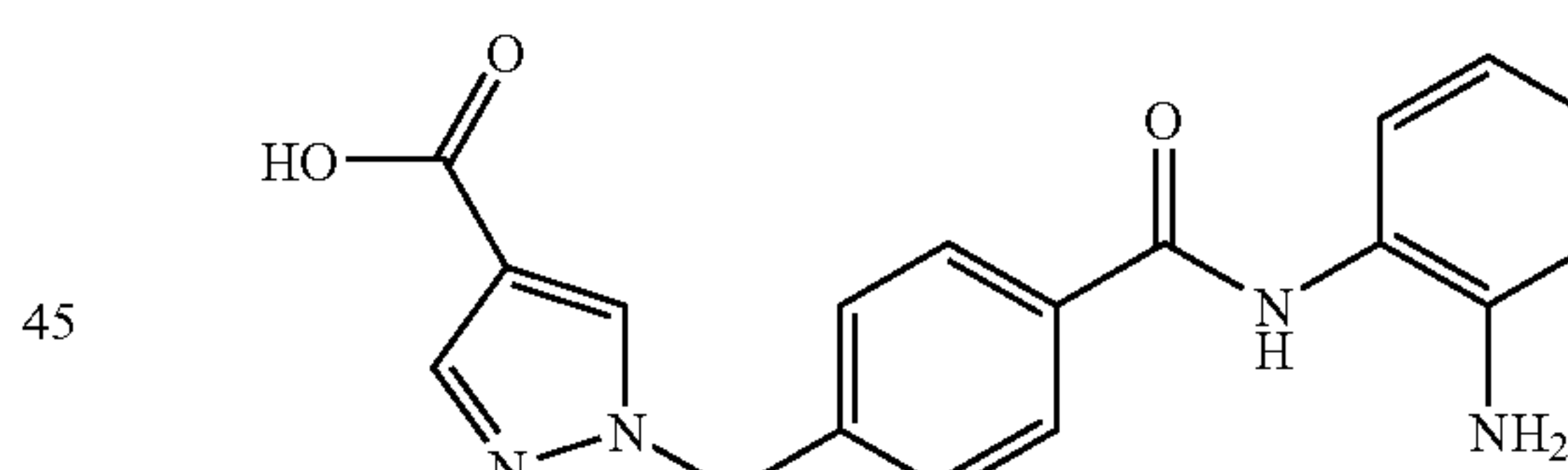
1-(4-((2-aminophenyl)carbamoyl)benzyl)-1H-pyrazole-4-carboxylic acid
