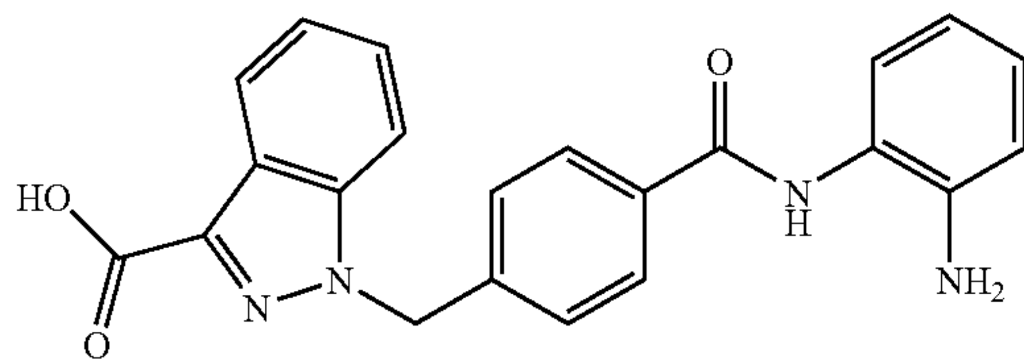
1-(4-((2-aminophenyl)carbamoyl)benzyl)-1H-indazole-3-carboxylic acid
